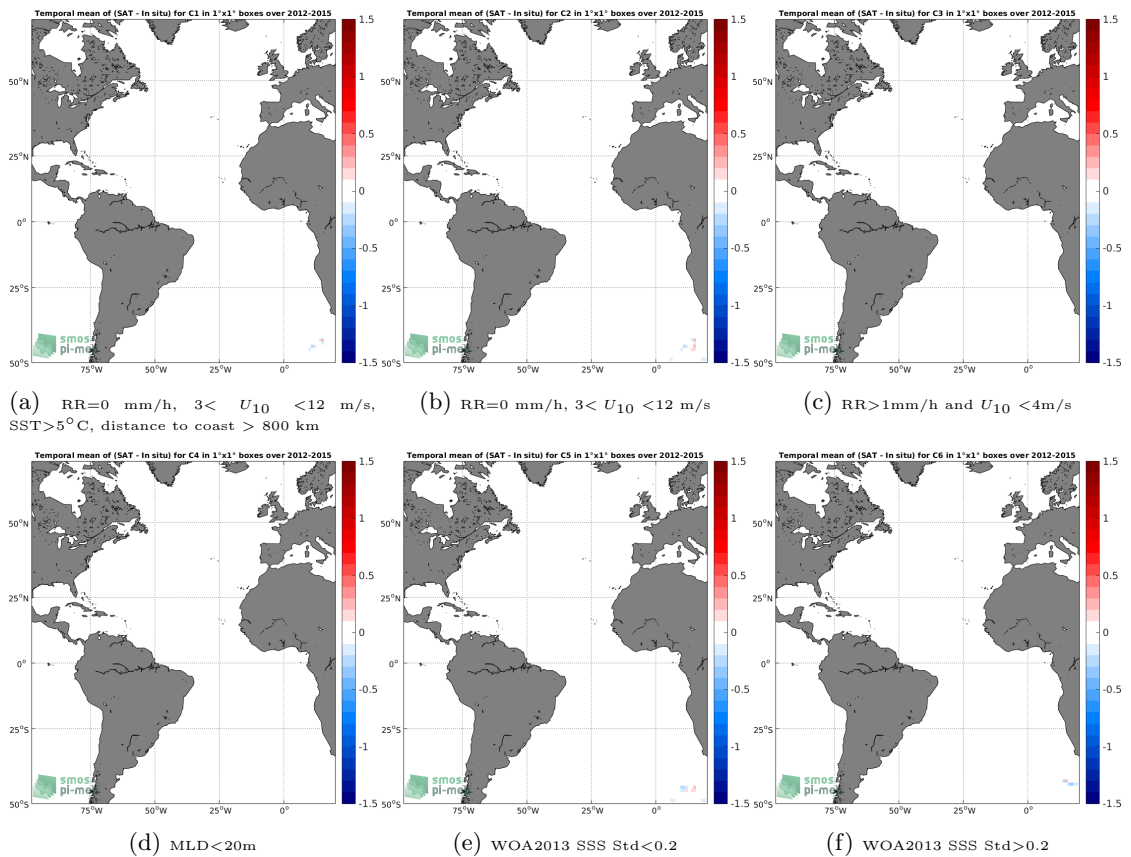
Figure 12: Temporal mean gridded over spatial boxes of size 1°x1° of \Delta SSS (Aquarius-L4-IPRC-V5-MONTHLY - Sea mammals) for 6 different subdatasets corresponding to:RR=0 mm/h, 3 < U_{10} < 12 m/s, SST>5°C, distance to coast > 800 km (a), RR=0 mm/h, 3 < U_{10} < 12 m/s (b), RR>1mm/h and U_{10} < 4 m/s (c),MLD<20m (d),WOA2013 SSS Std<0.2 (e),WOA2013 SSS Std>0.2 (f).
