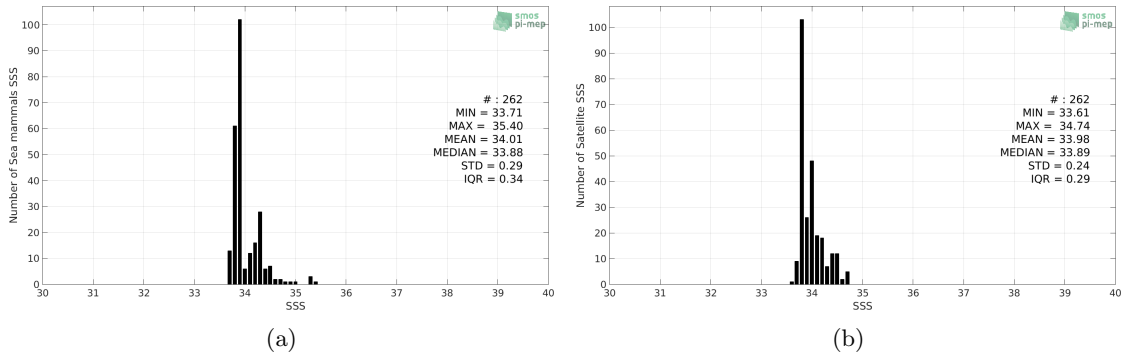
Figure 2: Histograms of SSS from Sea mammals (a) and Aquarius-L4-IPRC-V5-MONTHLY (b) considering all match-up pairs per bins of 0.1 over the Atlantic Ocean Pi-MEP region and for the full satellite product period.
