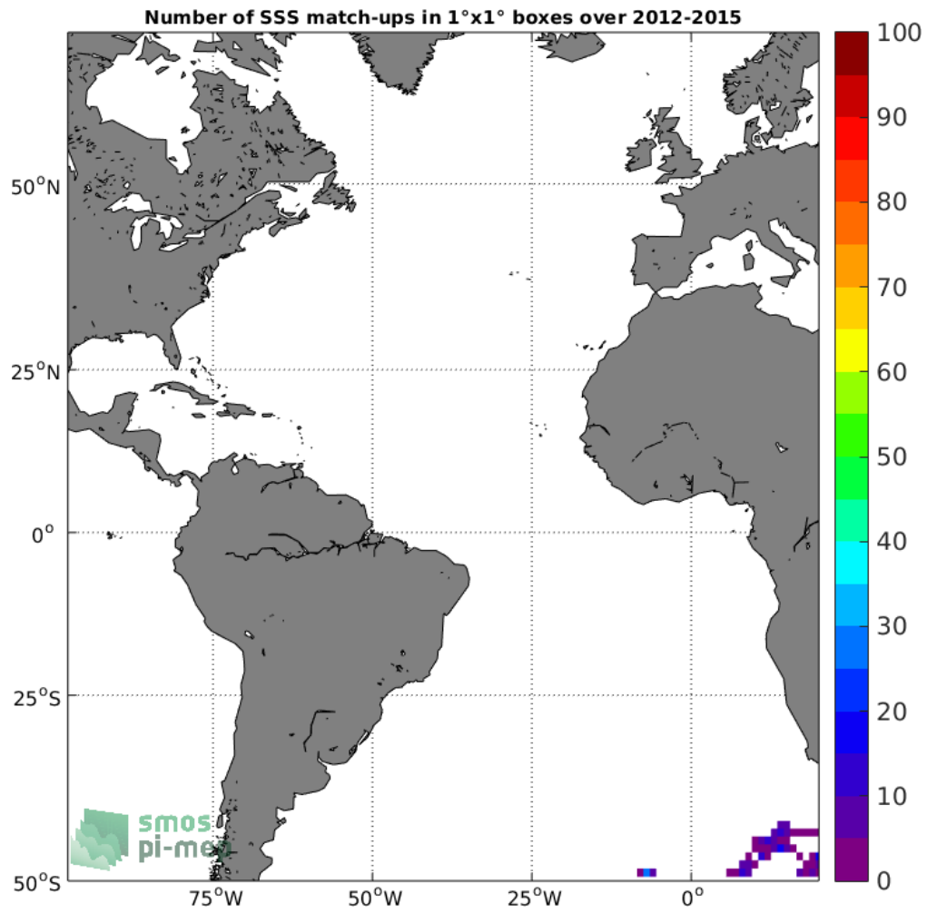
Figure 4: Number of SSS match-ups between Sea mammals SSS and the Aquarius-L4-IPRC-V5-MONTHLY SSS product for the Atlantic Ocean Pi-MEP region over 1°x1° boxes and for the full satellite product period.
