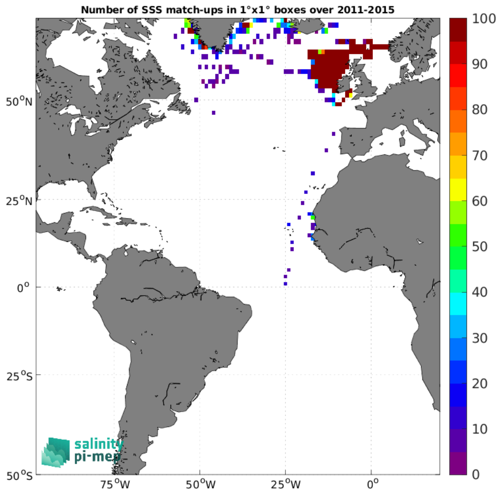
Figure 5: Number of SSS match-ups between ICES SSS and the Aquarius SSS L4 OI v5 - Monthly (IPRC) SSS product for the Atlantic Ocean Pi-MEP region over 1°x1° boxes and for the full satellite product period.
