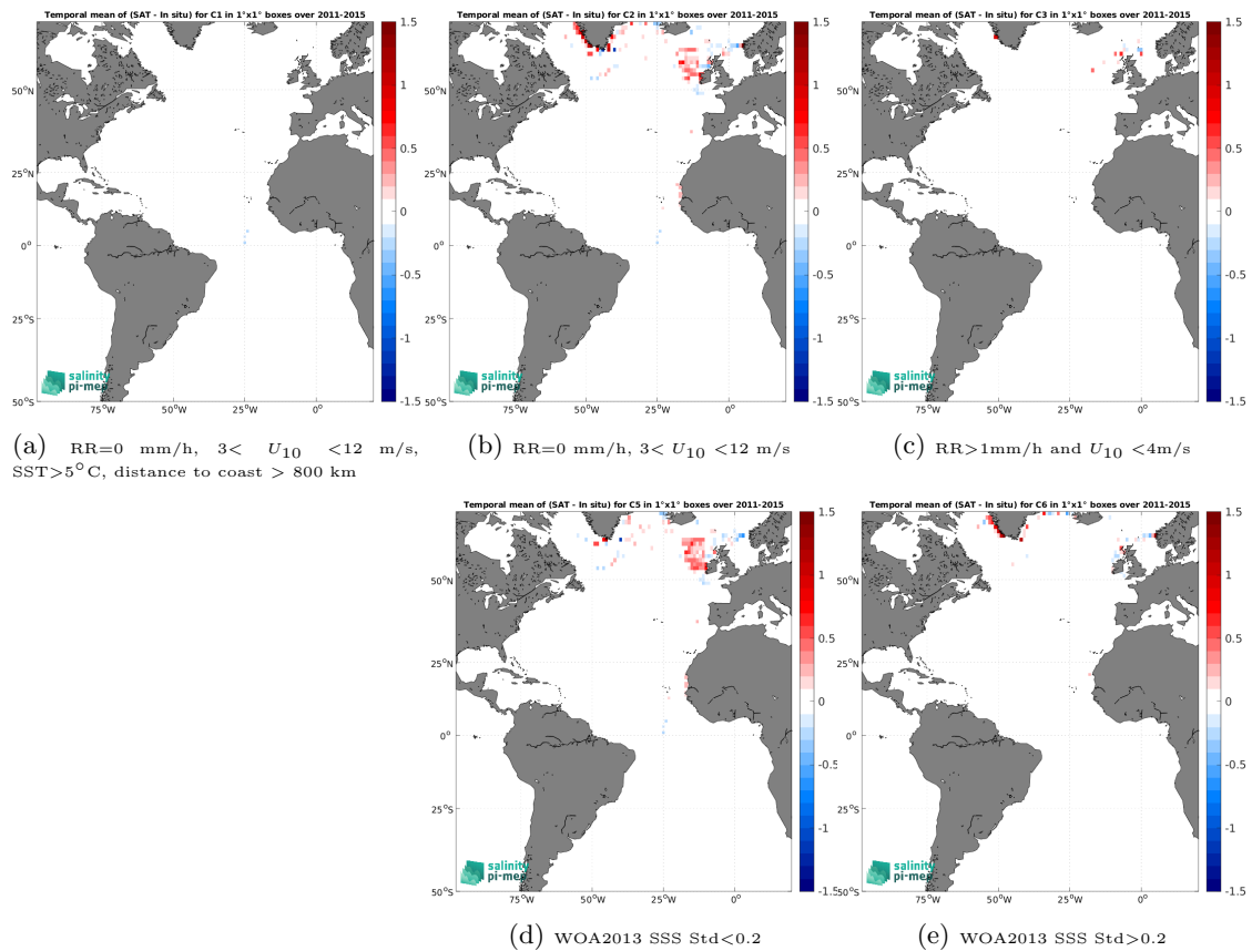
Figure 14: Temporal mean gridded over spatial boxes of size 1^\circ \times 1^\circ of \Delta SSS (Aquarius SSS L4 OI v5 - Monthly (IPRC) - ICES) for 5 different subdatasets corresponding to:RR=0 mm/h, 3 < U_{10} < 12 m/s, SST >5^\circ\text{C} , distance to coast > 800 km (a), RR=0 mm/h, 3 < U_{10} < 12 m/s (b), RR >1 mm/h and U_{10} < 4 m/s (c), WOA2013 SSS Std <0.2 (d), WOA2013 SSS Std >0.2 (e).
