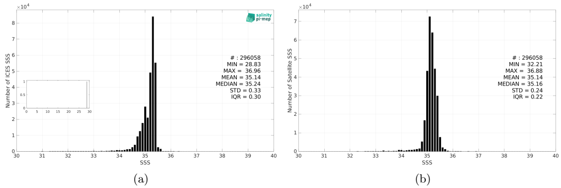
Figure 3: Histograms of SSS from ICES (a) and Aquarius SSS L4 OI v5 - Monthly (IPRC) (b) considering all match-up pairs per bins of 0.1 over the Atlantic Ocean Pi-MEP region and for the full satellite product period.
