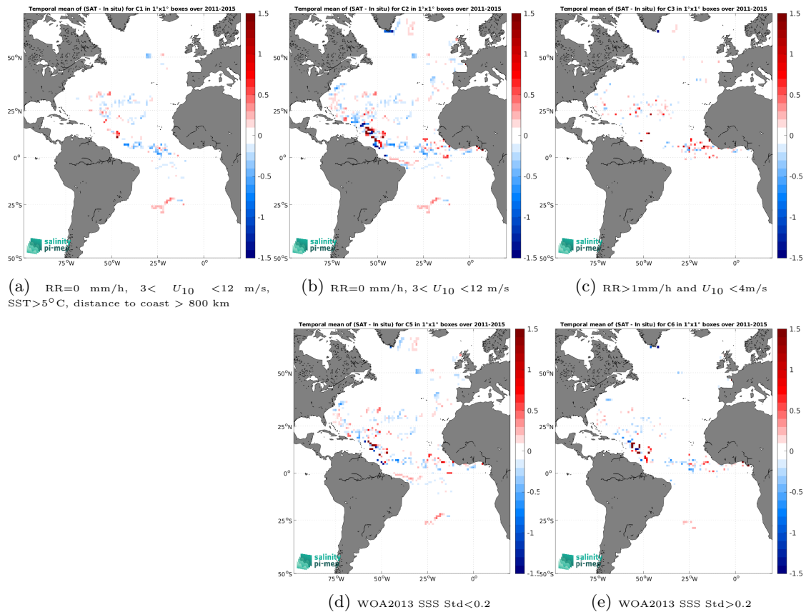
Figure 13: Temporal mean gridded over spatial boxes of size 1^\circ \times 1^\circ of \Delta SSS (Aquarius SSS L4 OI v5 - Monthly (IPRC) - Surface drifters) for 5 different subdatasets corresponding to:RR=0 mm/h, 3 < U_{10} < 12 m/s, SST >5^\circ\text{C} , distance to coast > 800 km (a), RR=0 mm/h, 3 < U_{10} < 12 m/s (b), RR >1 mm/h and U_{10} < 4 m/s (c), WOA2013 SSS Std <0.2 (d), WOA2013 SSS Std >0.2 (e).
