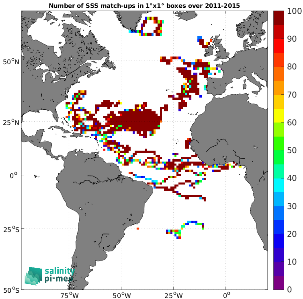
Figure 4: Number of SSS match-ups between Surface drifters SSS and the Aquarius SSS L4 OI v5 - Monthly (IPRC) SSS product for the Atlantic Ocean Pi-MEP region over 1°×1° boxes and for the full satellite product period.
