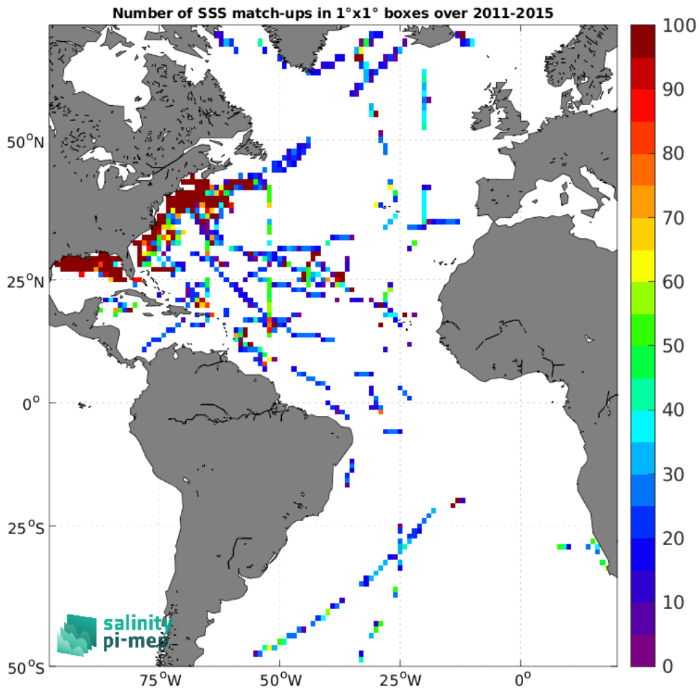
Figure 5: Number of SSS match-ups between TSG (SAMOS) SSS and the Aquarius SSS L3 OR v5 - 7-Day running (NASA-GSFC) SSS product for the Atlantic Ocean Pi-MEP region over 1^\circ \times 1^\circ boxes and for the full satellite product period.
