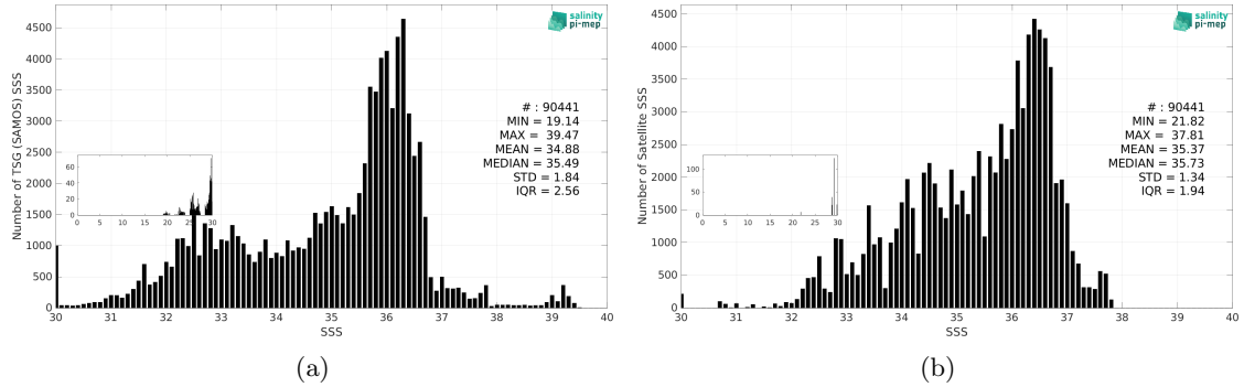
Figure 3: Histograms of SSS from TSG (SAMOS) (a) and Aquarius SSS L3 OR v5 - 7-Day running (NASA-GSFC) (b) considering all match-up pairs per bins of 0.1 over the Atlantic Ocean Pi-MEP region and for the full satellite product period.
