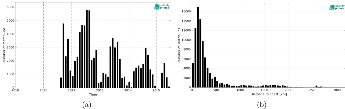
Figure 2: Number of match-ups between TSG (SAMOS) and Aquarius SSS L3 OR v5 - 7-Day running (NASA-GSFC) SSS as a function of time (a) and as function of the distance to coast (b) over the Atlantic Ocean Pi-MEP region and for the full satellite product period.
