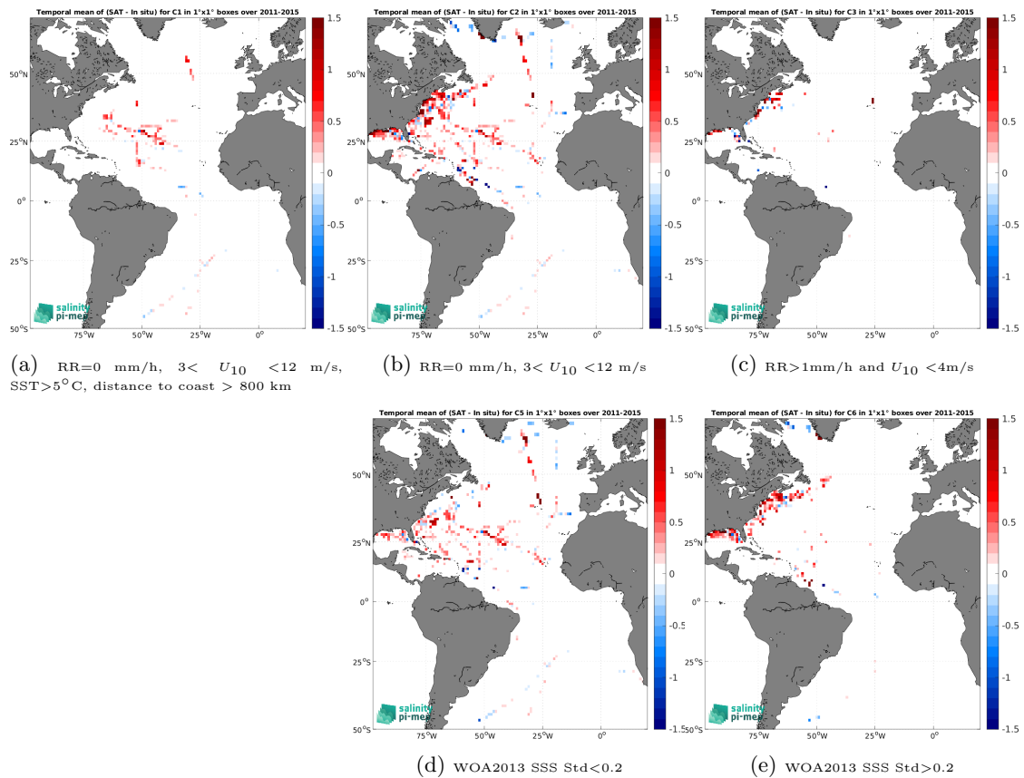
Figure 14: Temporal mean gridded over spatial boxes of size 1^\circ \times 1^\circ of \Delta\text{SSS} (Aquarius SSS L3 OR v5 - 7-Day running (NASA-GSFC) - TSG (SAMOS)) for 5 different subdatasets corresponding to:RR=0 mm/h, 3 < U_{10} < 12 m/s, SST >5^\circ\text{C} , distance to coast > 800 km (a), RR=0 mm/h, 3 < U_{10} < 12 m/s (b), RR >1 mm/h and U_{10} < 4 m/s (c), WOA2013 SSS Std <0.2 (d), WOA2013 SSS Std >0.2 (e).
