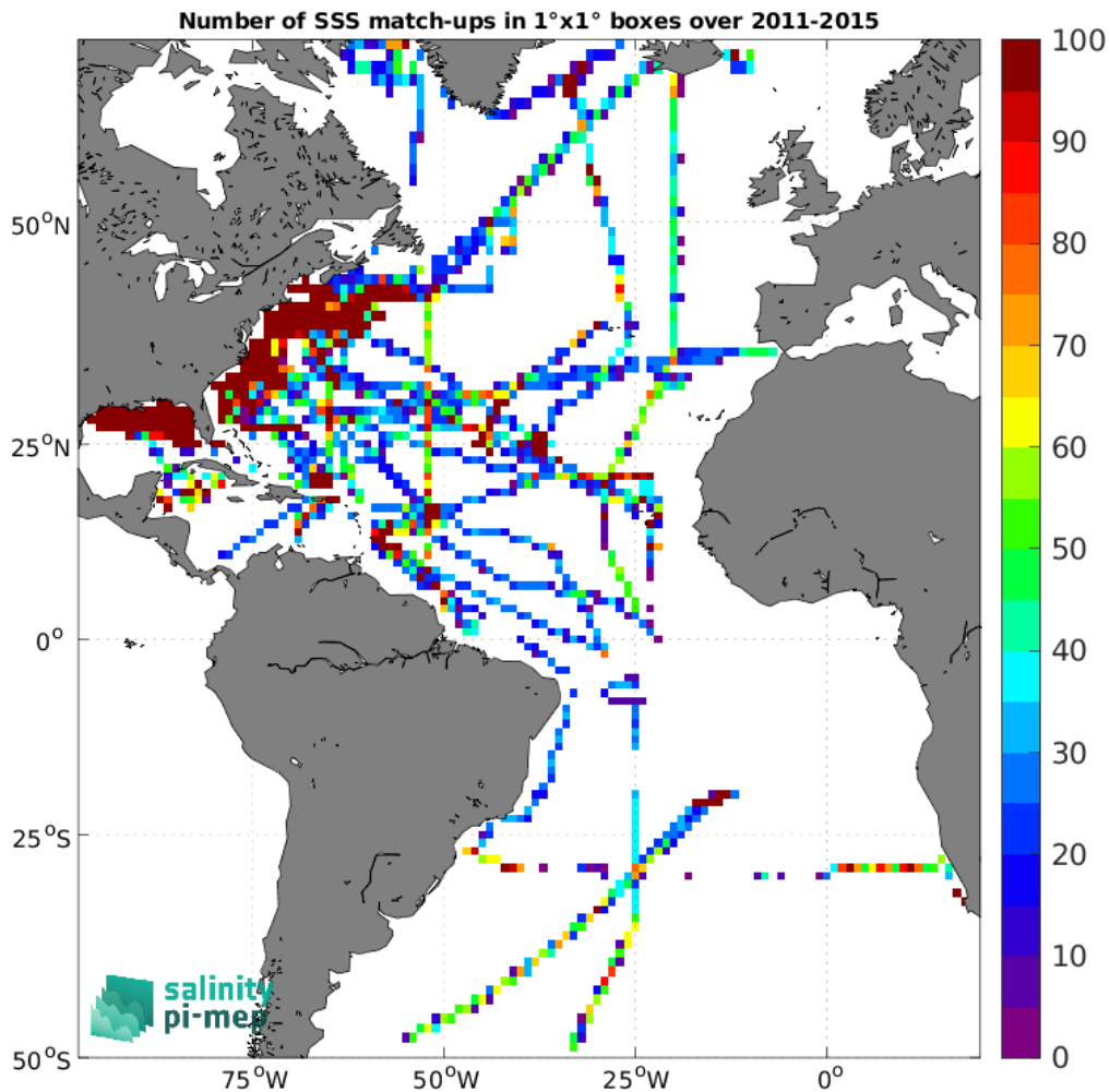
Figure 4: Number of SSS match-ups between TSG (SAMOS) SSS and the Aquarius SSS L3 OR v5 - 7-Day running (NASA-GSFC) SSS product for the Atlantic Ocean Pi-MEP region over 1°x1° boxes and for the full satellite product period.
