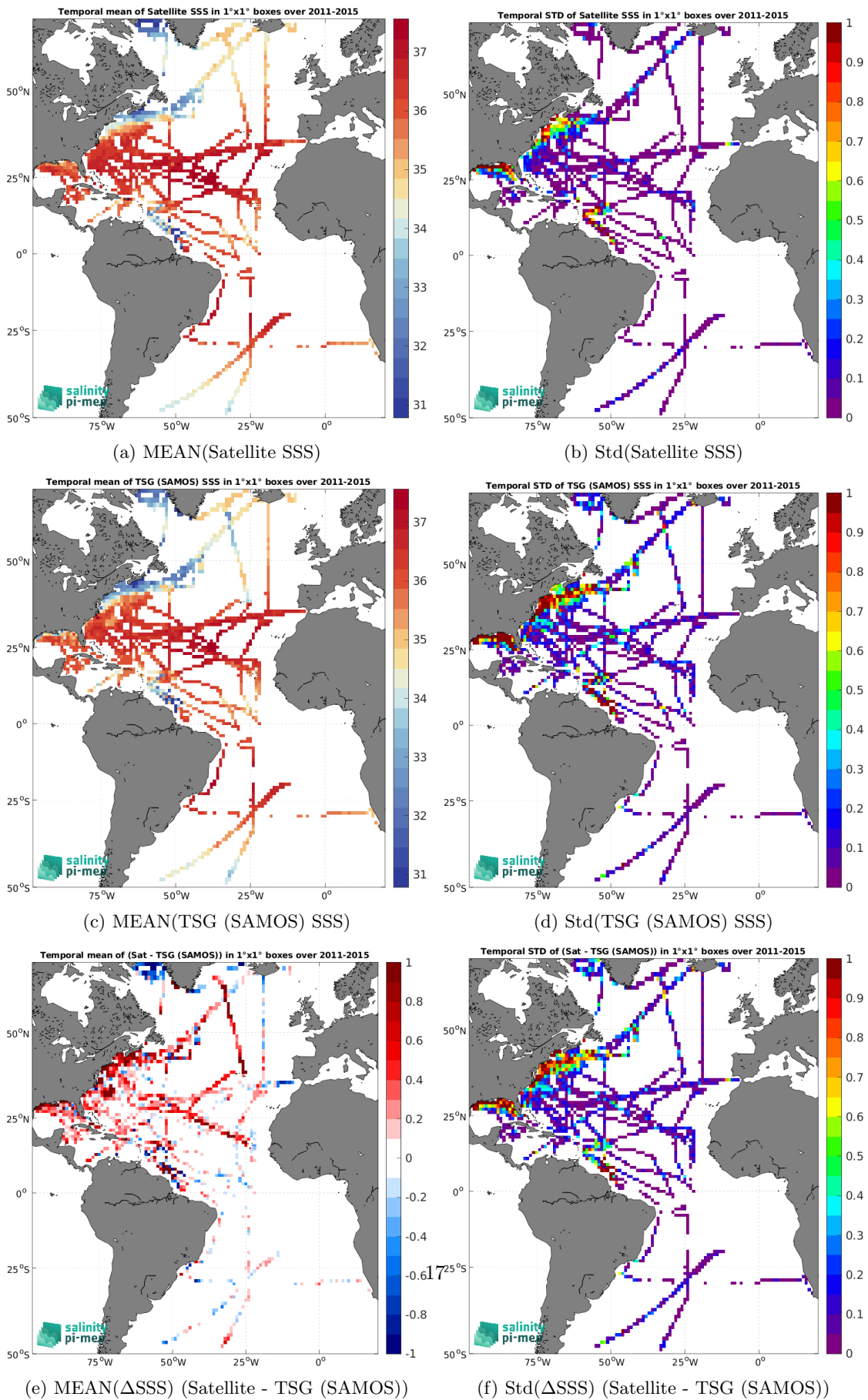
(e) MEAN( \Delta SSS) (Satellite - TSG (SAMOS)) (f) Std( \Delta SSS) (Satellite - TSG (SAMOS)) Figure 6: Temporal mean (left) and Std (right) of SSS from Aquarius SSS L3 OR v5 - 7-Day running (NASA-GSFC) (top), TSG (SAMOS) (middle), and of \Delta SSS (Satellite - TSG (SAMOS)). Only match-up pairs are used to generate these maps.
