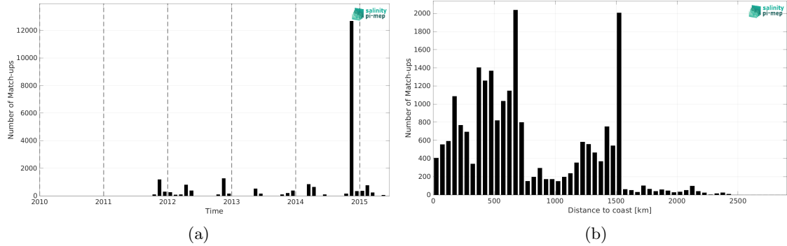
Figure 2: Number of match-ups between TSG (Polarstern) and Aquarius SSS L3 OR v5 - 7-Day running (NASA-GSFC) SSS as a function of time (a) and as function of the distance to coast (b) over the Atlantic Ocean Pi-MEP region and for the full satellite product period.
