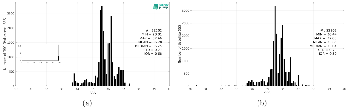
Figure 3: Histograms of SSS from TSG (Polarstern) (a) and Aquarius SSS L3 OR v5 - 7-Day running (NASA-GSFC) (b) considering all match-up pairs per bins of 0.1 over the Atlantic Ocean Pi-MEP region and for the full satellite product period.
