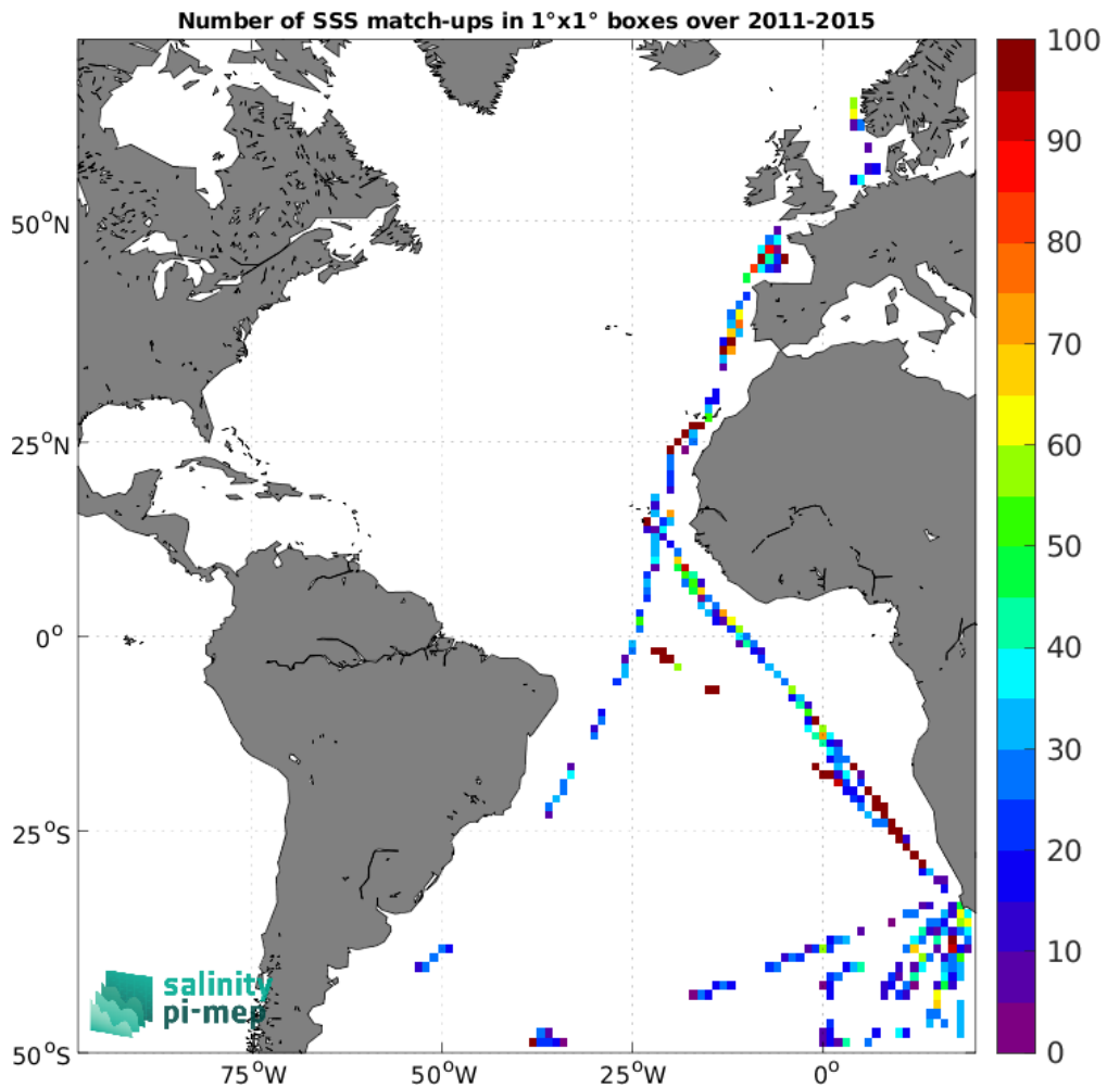
Figure 5: Number of SSS match-ups between TSG (Polarstern) SSS and the Aquarius SSS L3 OR v5 - 7-Day running (NASA-GSFC) SSS product for the Atlantic Ocean Pi-MEP region over 1^\circ \times 1^\circ boxes and for the full satellite product period.
