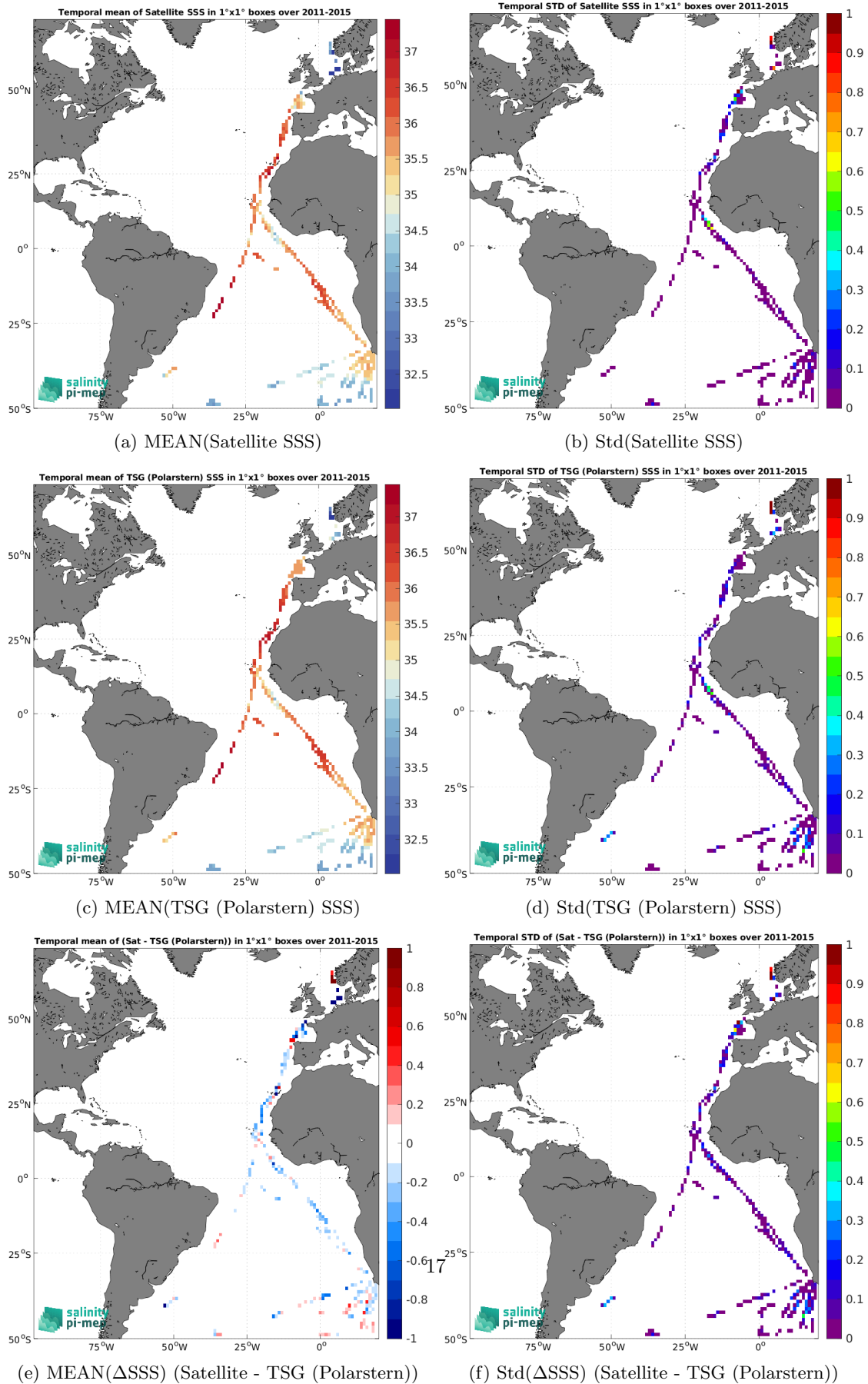
Figure 7: Temporal mean (left) and Std (right) of SSS from Aquarius SSS L3 OR v5 - 7-Day running (NASA-GSFC) (top), TSG (Polarstern) (middle), and of \Delta SSS (Satellite - TSG (Polarstern)). Only match-up pairs are used to generate these maps.
