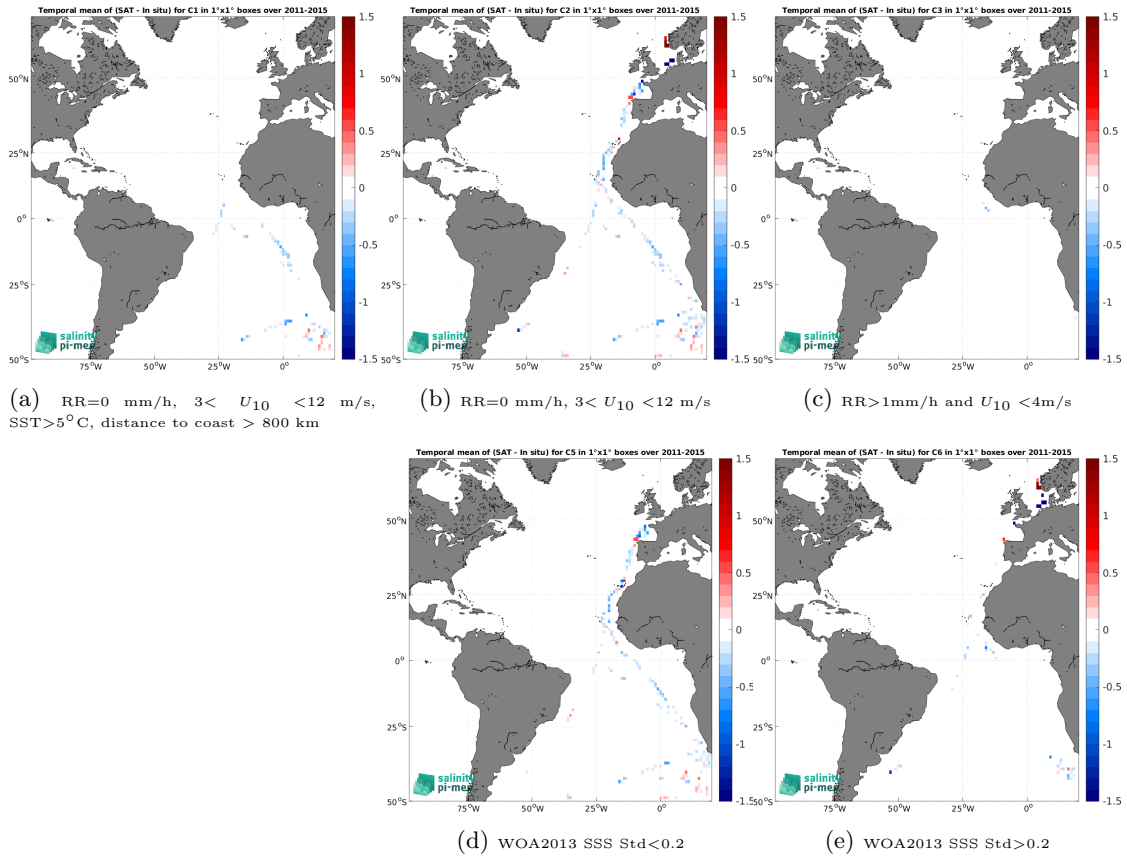
Figure 14: Temporal mean gridded over spatial boxes of size 1^\circ \times 1^\circ of \Delta SSS (Aquarius SSS L3 OR v5 - 7-Day running (NASA-GSFC) - TSG (Polarstern)) for 5 different subdatasets corresponding to:RR=0 mm/h, 3 < U_{10} < 12 m/s, SST >5^\circ\text{C} , distance to coast > 800 km (a), RR=0 mm/h, 3 < U_{10} < 12 m/s (b), RR >1 mm/h and U_{10} < 4 m/s (c), WOA2013 SSS Std <0.2 (d), WOA2013 SSS Std >0.2 (e).
