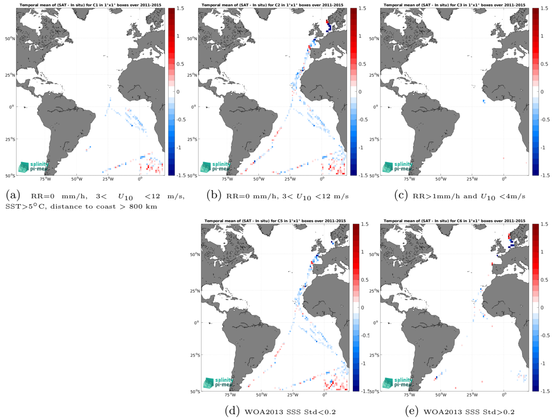
Figure 12: Temporal mean gridded over spatial boxes of size 1^\circ \times 1^\circ of \Delta SSS (Aquarius SSS L3 OR v5 - 7-Day running (NASA-GSFC) - TSG (Polarstern)) for 5 different subdatasets corresponding to:RR=0 mm/h, 3 < U_{10} < 12 m/s, SST >5^\circ\text{C} , distance to coast > 800 km (a), RR=0 mm/h, 3 < U_{10} < 12 m/s (b), RR >1 mm/h and U_{10} < 4 m/s (c), WOA2013 SSS Std <0.2 (d), WOA2013 SSS Std >0.2 (e).
