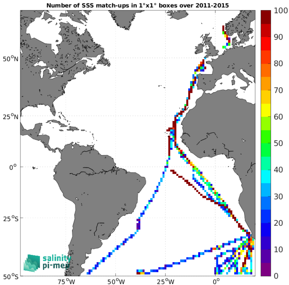
Figure 4: Number of SSS match-ups between TSG (Polarstern) SSS and the Aquarius SSS L3 OR v5 - 7-Day running (NASA-GSFC) SSS product for the Atlantic Ocean Pi-MEP region over 1^\circ \times 1^\circ boxes and for the full satellite product period.
