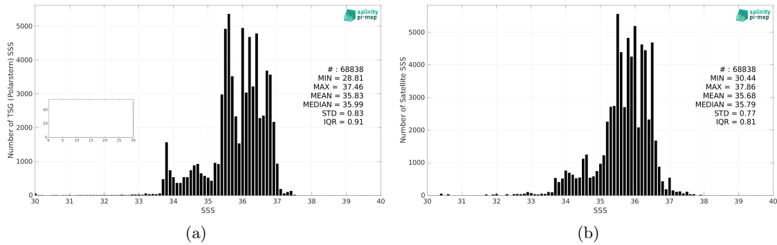
Figure 2: Histograms of SSS from TSG (Polarstern) (a) and Aquarius SSS L3 OR v5 - 7-Day running (NASA-GSFC) (b) considering all match-up pairs per bins of 0.1 over the Atlantic Ocean Pi-MEP region and for the full satellite product period.
