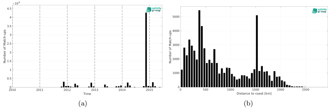
Figure 1: Number of match-ups between TSG (Polarstern) and Aquarius SSS L3 OR v5 - 7-Day running (NASA-GSFC) SSS as a function of time (a) and as function of the distance to coast (b) over the Atlantic Ocean Pi-MEP region and for the full satellite product period.
