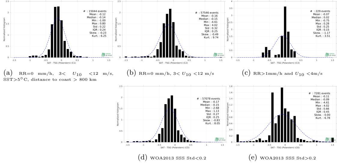
Figure 13: Normalized histogram of \Delta\text{SSS} (Aquarius SSS L3 OR v5 - 7-Day running (NASA-GSFC) - TSG (Polarstern)) for 5 different subdatasets corresponding to: RR=0 mm/h, 3 < U_{10} < 12 m/s, SST>5°C, distance to coast > 800 km (a), RR=0 mm/h, 3 < U_{10} < 12 m/s (b), RR>1mm/h and U_{10} < 4 m/s (c), WOA2013 SSS Std<0.2 (d), WOA2013 SSS Std>0.2 (e).
