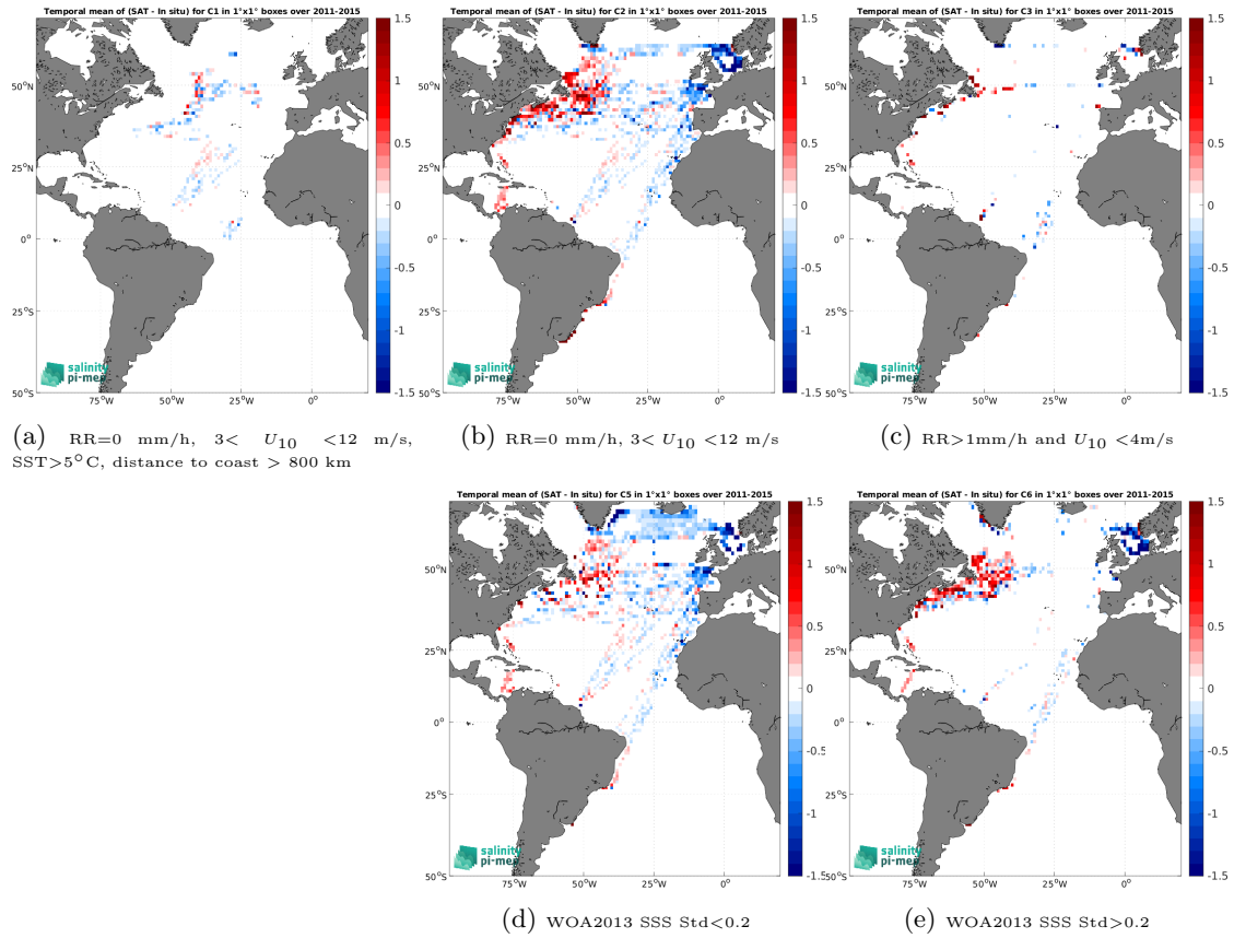
Figure 12: Temporal mean gridded over spatial boxes of size 1^\circ \times 1^\circ of \Delta SSS (Aquarius SSS L3 OR v5 - 7-Day running (NASA-GSFC) - TSG (LEGOS-DM)) for 5 different subdatasets corresponding to:RR=0 mm/h, 3 < U_{10} < 12 m/s, SST >5^\circ\text{C} , distance to coast > 800 km (a), RR=0 mm/h, 3 < U_{10} < 12 m/s (b), RR >1 mm/h and U_{10} < 4 m/s (c), WOA2013 SSS Std <0.2 (d), WOA2013 SSS Std >0.2 (e).
