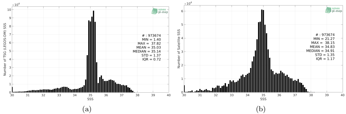
Figure 2: Histograms of SSS from TSG (LEGOS-DM) (a) and Aquarius SSS L3 OR v5 - 7-Day running (NASA-GSFC) (b) considering all match-up pairs per bins of 0.1 over the Atlantic Ocean Pi-MEP region and for the full satellite product period.
