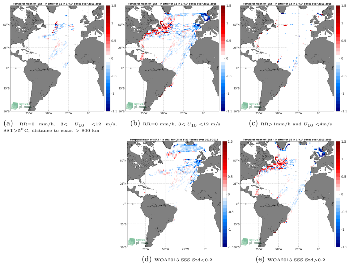
Figure 12: Temporal mean gridded over spatial boxes of size 1^\circ \times 1^\circ of \Delta\text{SSS} (Aquarius SSS L3 OR v5 - 7-Day running (NASA-GSFC) - TSG (LEGOS-DM)) for 5 different subdatasets corresponding to:RR=0 mm/h, 3 < U_{10} < 12 m/s, SST >5^\circ\text{C} , distance to coast > 800 km (a), RR=0 mm/h, 3 < U_{10} < 12 m/s (b), RR >1 mm/h and U_{10} < 4 m/s (c), WOA2013 SSS Std <0.2 (d), WOA2013 SSS Std >0.2 (e).
