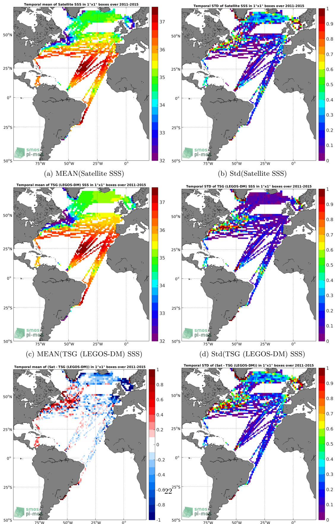
(e) MEAN( \Delta SSS) (Satellite - TSG (LEGOS-DM)) (f) Std( \Delta SSS) (Satellite - TSG (LEGOS-DM)) Figure 6: Temporal mean (left) and Std (right) of SSS from Aquarius SSS L3 OR v5 - 7-Day running (NASA-GSFC) (top), TSG (LEGOS-DM) (middle), and of \Delta SSS (Satellite - TSG (LEGOS-DM)). Only match-up pairs are used to generate these maps.
