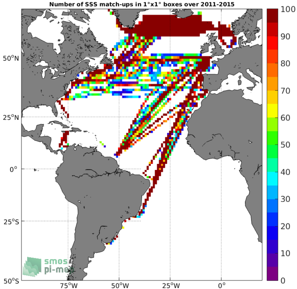
Figure 4: Number of SSS match-ups between TSG (LEGOS-DM) SSS and the Aquarius SSS L3 OR v5 - 7-Day running (NASA-GSFC) SSS product for the Atlantic Ocean Pi-MEP region over 1^\circ \times 1^\circ boxes and for the full satellite product period.
