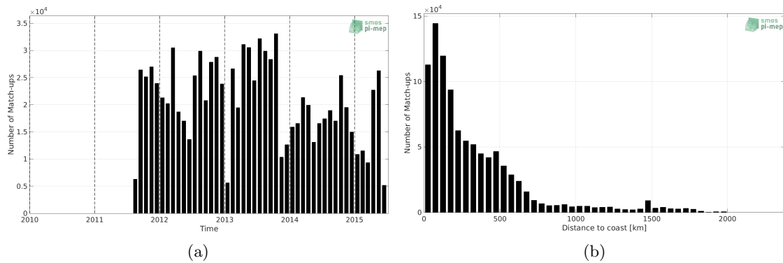
Figure 1: Number of match-ups between TSG (LEGOS-DM) and Aquarius SSS L3 OR v5 - 7-Day running (NASA-GSFC) SSS as a function of time (a) and as function of the distance to coast (b) over the Atlantic Ocean Pi-MEP region and for the full satellite product period.
