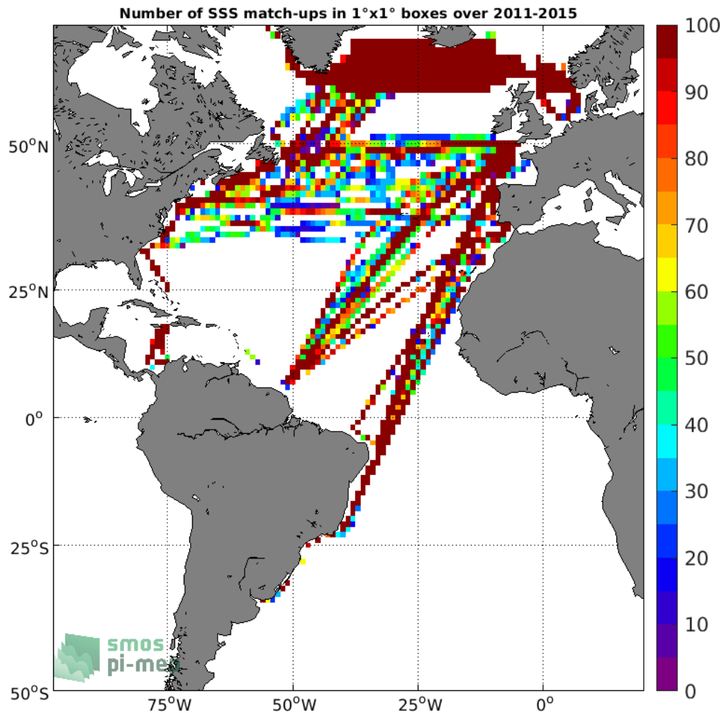
Figure 4: Number of SSS match-ups between TSG (LEGOS-DM) SSS and the Aquarius SSS L3 OR v5 - 7-Day running (NASA-GSFC) SSS product for the Atlantic Ocean Pi-MEP region over 1°x1° boxes and for the full satellite product period.
