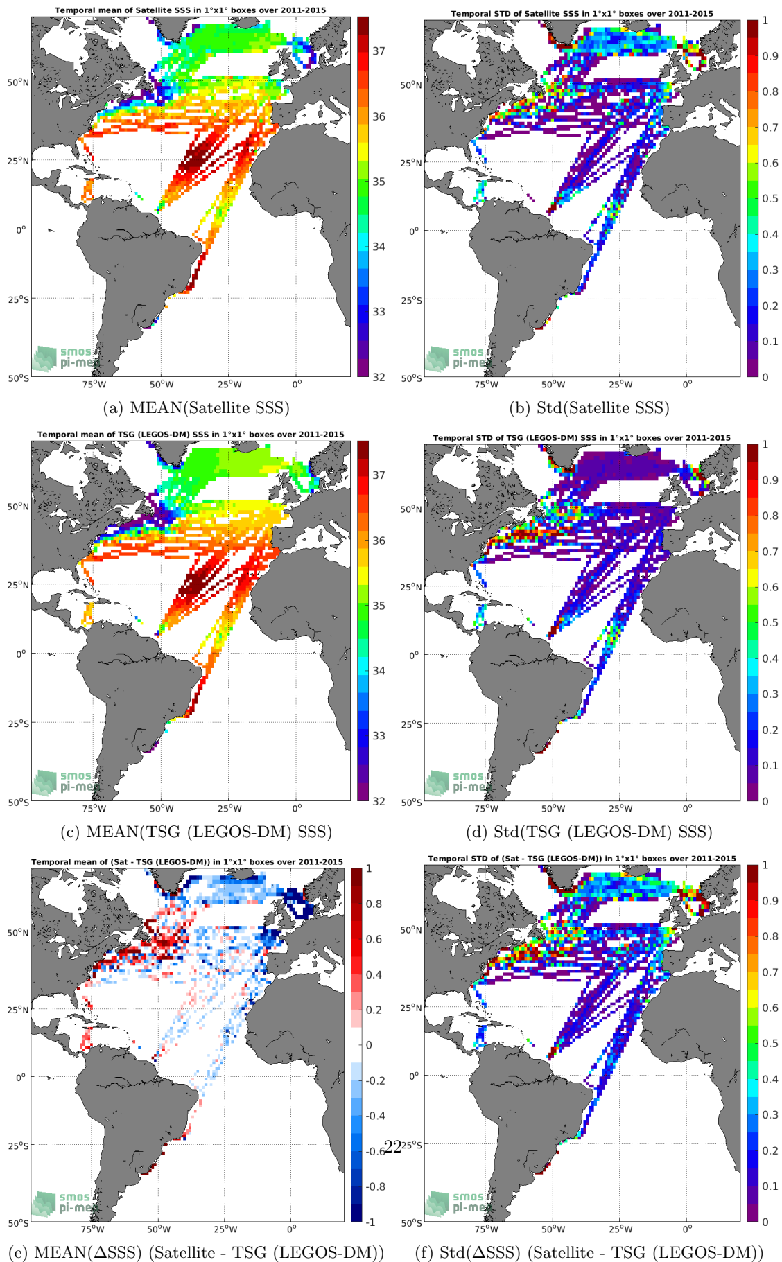
Figure 6: Temporal mean (left) and Std (right) of SSS from Aquarius SSS L3 OR v5 - 7-Day running (NASA-GSFC) (top), TSG (LEGOS-DM) (middle), and of \Delta SSS (Satellite - TSG (LEGOS-DM)). Only match-up pairs are used to generate these maps.
