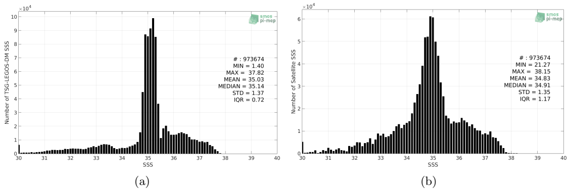
Figure 2: Histograms of SSS from TSG-LEGOS-DM (a) and Aquarius-L3-OR-V5-7DAY-RUNNING-1DEG (b) considering all match-up pairs per bins of 0.1 over the Atlantic Ocean Pi-MEP region and for the full satellite product period.
