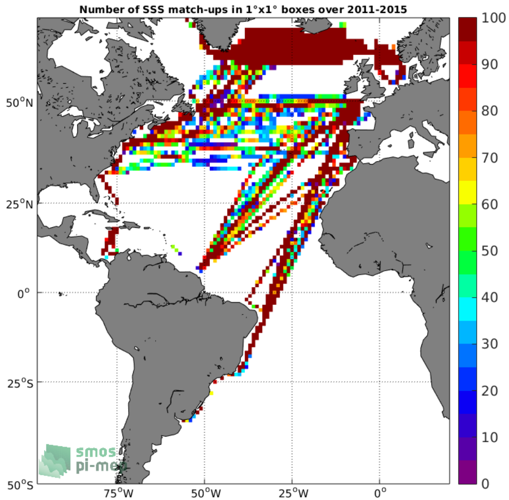
Figure 4: Number of SSS match-ups between TSG-LEGOS-DM SSS and the Aquarius-L3-OR-V5-7DAY-RUNNING-1DEG SSS product for the Atlantic Ocean Pi-MEP region over 1°x1° boxes and for the full satellite product period.
