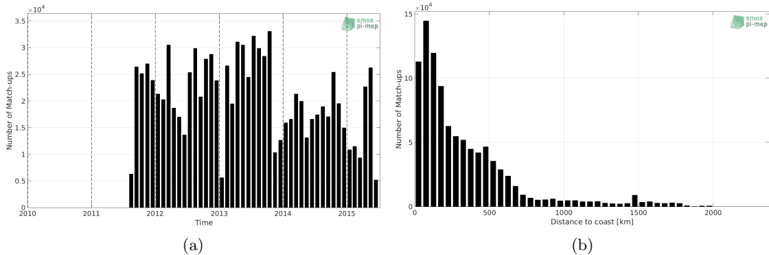
Figure 1: Number of match-ups between TSG-LEGOS-DM and Aquarius-L3-OR-V5-7DAY-RUNNING-1DEG SSS as a function of time (a) and as function of the distance to coast (b) over the Atlantic Ocean Pi-MEP region and for the full satellite product period.
