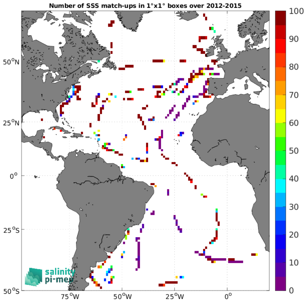
Figure 5: Number of SSS match-ups between TSG (GOSUD-Sailing-ship) SSS and the Aquarius SSS L3 OR v5 - 7-Day running (NASA-GSFC) SSS product for the Atlantic Ocean Pi-MEP region over 1^\circ \times 1^\circ boxes and for the full satellite product period.
