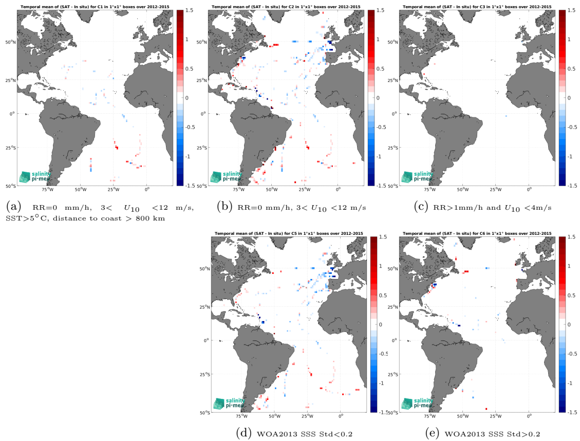
Figure 14: Temporal mean gridded over spatial boxes of size 1^\circ \times 1^\circ of \Delta\text{SSS} (Aquarius SSS L3 OR v5 - 7-Day running (NASA-GSFC) - TSG (GOSUD-Sailing-ship)) for 5 different subdatasets corresponding to:RR=0 mm/h, 3 < U_{10} < 12 m/s, SST>5°C, distance to coast > 800 km (a), RR=0 mm/h, 3 < U_{10} < 12 m/s (b), RR>1mm/h and U_{10} < 4 m/s (c), WOA2013 SSS Std<0.2 (d), WOA2013 SSS Std>0.2 (e).
