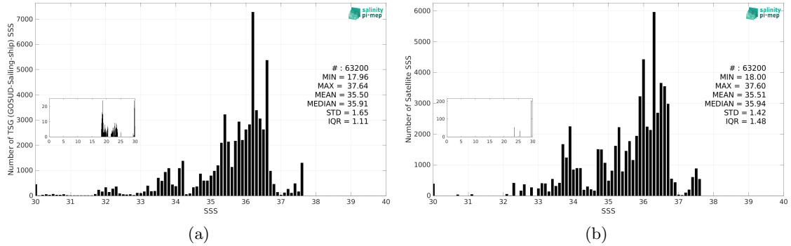
Figure 3: Histograms of SSS from TSG (GOSUD-Sailing-ship) (a) and Aquarius SSS L3 OR v5 - 7-Day running (NASA-GSFC) (b) considering all match-up pairs per bins of 0.1 over the Atlantic Ocean Pi-MEP region and for the full satellite product period.
