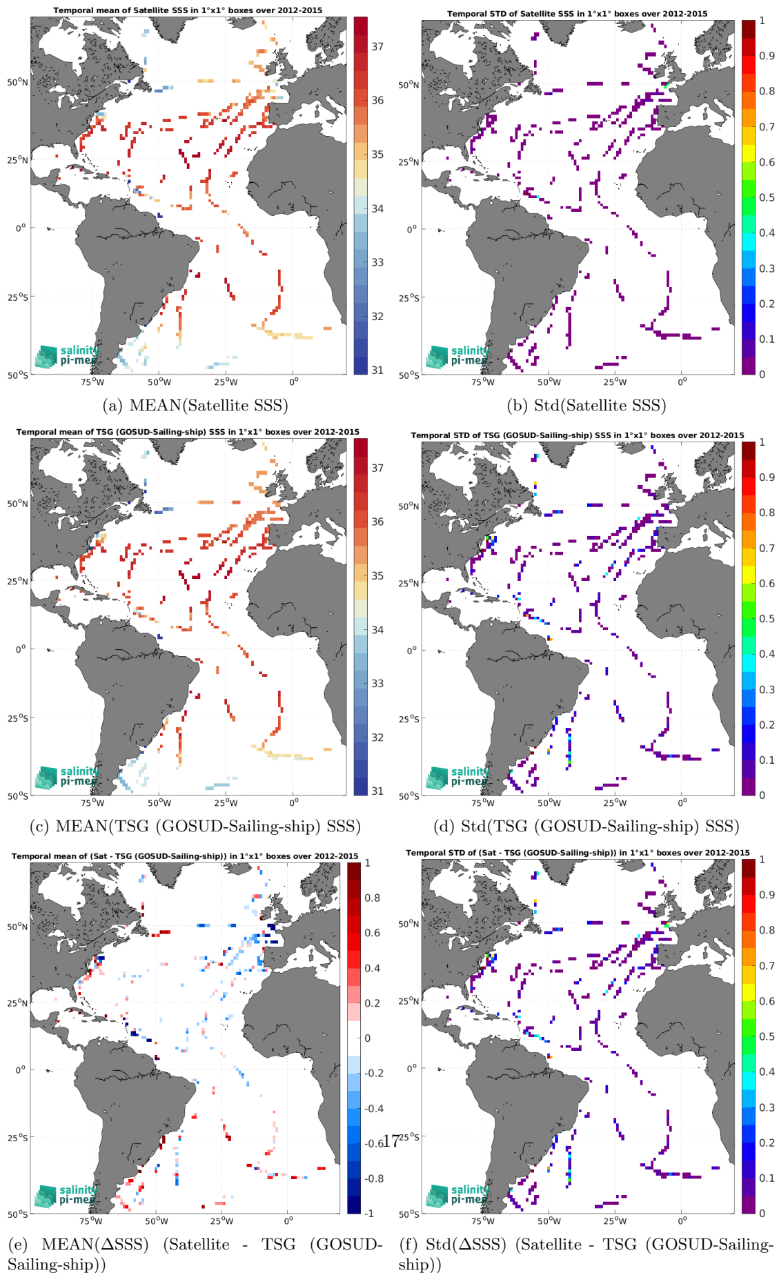
Figure 7: Temporal mean (left) and Std (right) of SSS from Aquarius SSS L3 OR v5 - 7-Day running (NASA-GSFC) (top), TSG (GOSUD-Sailing-ship) (middle), and of \Delta SSS (Satellite - TSG (GOSUD-Sailing-ship)). Only match-up pairs are used to generate these maps.
