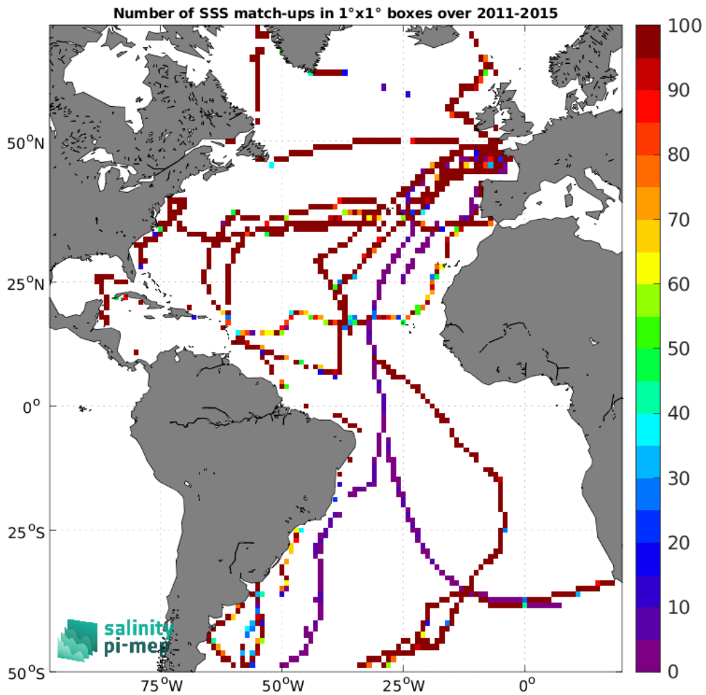
Figure 4: Number of SSS match-ups between TSG (GOSUD-Sailing-ship) SSS and the Aquarius SSS L3 OR v5 - 7-Day running (NASA-GSFC) SSS product for the Atlantic Ocean Pi-MEP region over 1^\circ \times 1^\circ boxes and for the full satellite product period.
