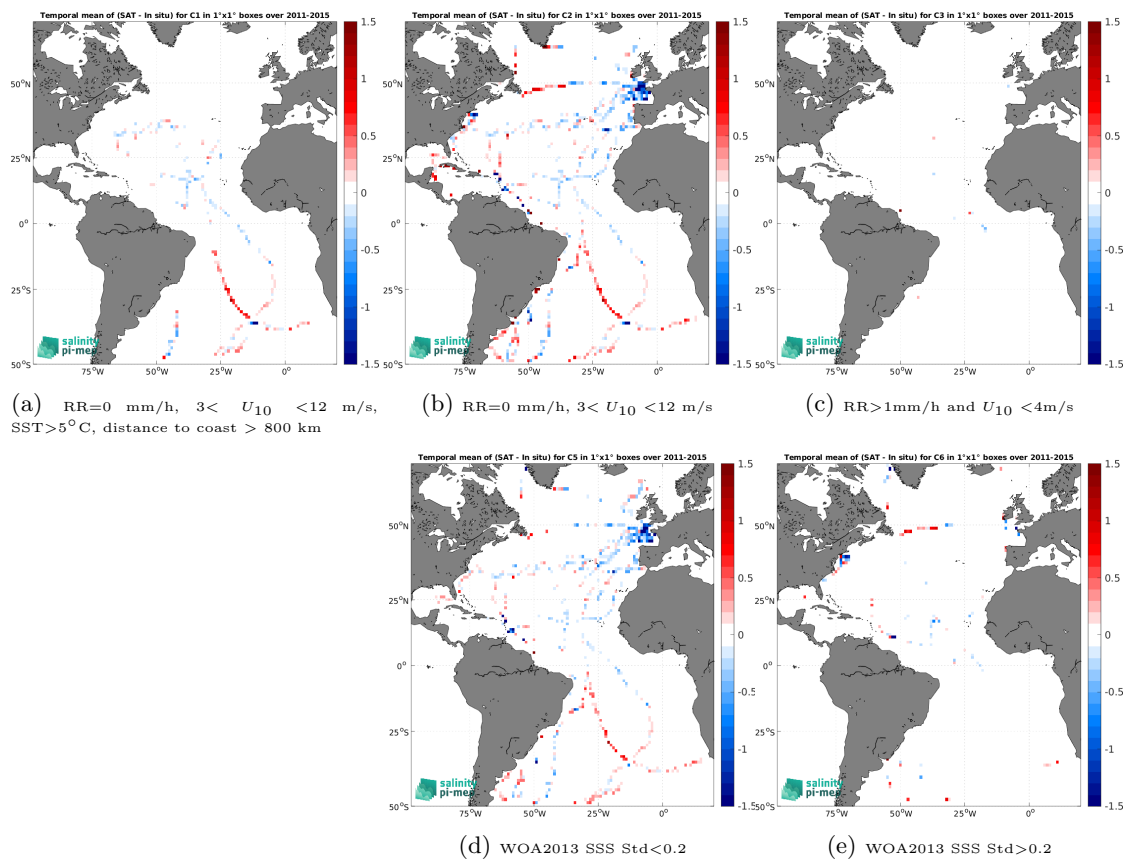
Figure 12: Temporal mean gridded over spatial boxes of size 1^\circ \times 1^\circ of \Delta\text{SSS} (Aquarius SSS L3 OR v5 - 7-Day running (NASA-GSFC) - TSG (GOSUD-Sailing-ship)) for 5 different subdatasets corresponding to:RR=0 mm/h, 3 < U_{10} < 12 m/s, SST >5^\circ\text{C} , distance to coast > 800 km (a), RR=0 mm/h, 3 < U_{10} < 12 m/s (b), RR >1 mm/h and U_{10} < 4 m/s (c), WOA2013 SSS Std <0.2 (d), WOA2013 SSS Std >0.2 (e).
