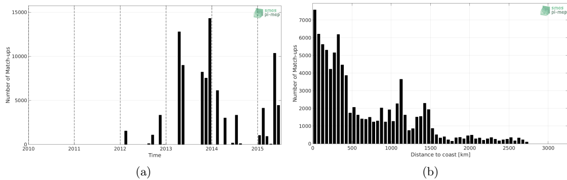
Figure 1: Number of match-ups between TSG-GOSUD-Sailing-ship and Aquarius-L3-OR-V5-7DAY-RUNNING-1DEG SSS as a function of time (a) and as function of the distance to coast (b) over the Atlantic Ocean Pi-MEP region and for the full satellite product period.
