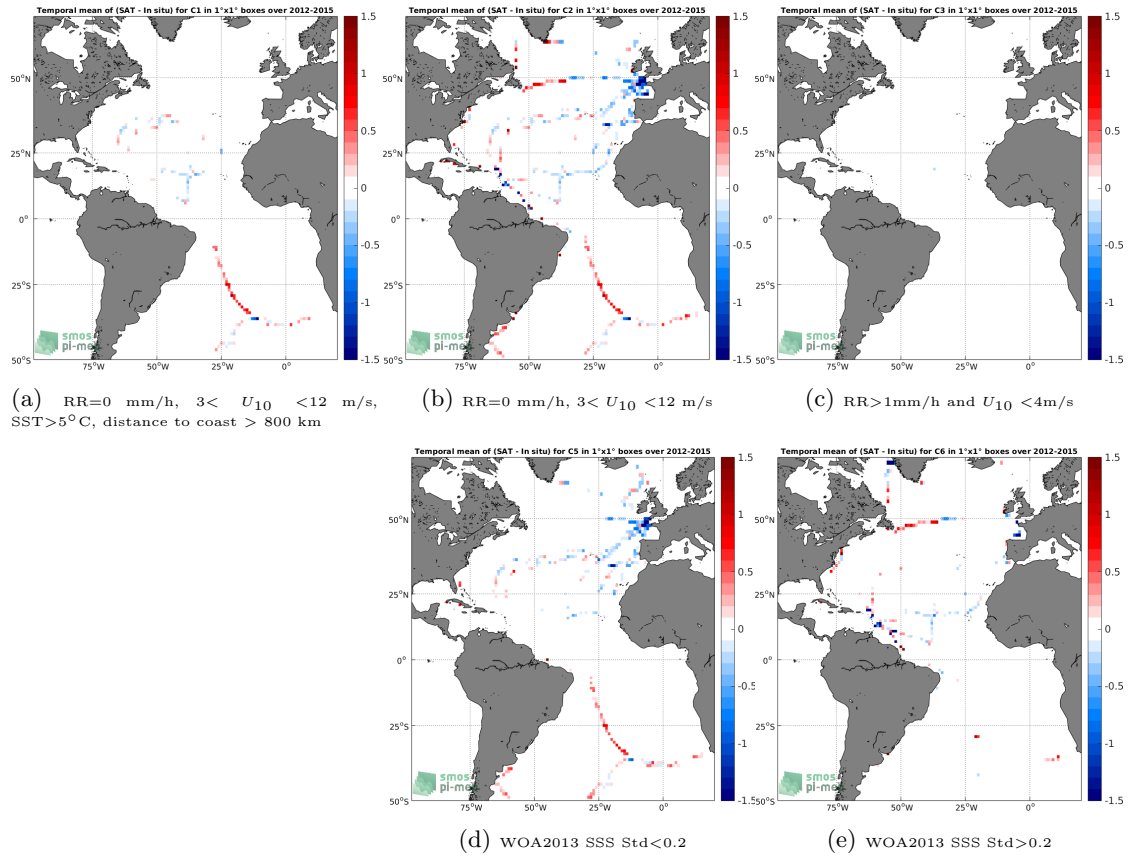
Figure 12: Temporal mean gridded over spatial boxes of size 1^\circ \times 1^\circ of \Delta SSS (Aquarius-L3-OR-V5-7DAY-RUNNING-1DEG - TSG-GOSUD-Sailing-ship) for 5 different subdatasets corresponding to:RR=0 mm/h, 3 < U_{10} < 12 m/s, SST >5^\circ C, distance to coast > 800 km (a), RR=0 mm/h, 3 < U_{10} < 12 m/s (b), RR >1 mm/h and U_{10} < 4 m/s (c), WOA2013 SSS Std <0.2 (d), WOA2013 SSS Std >0.2 (e).
