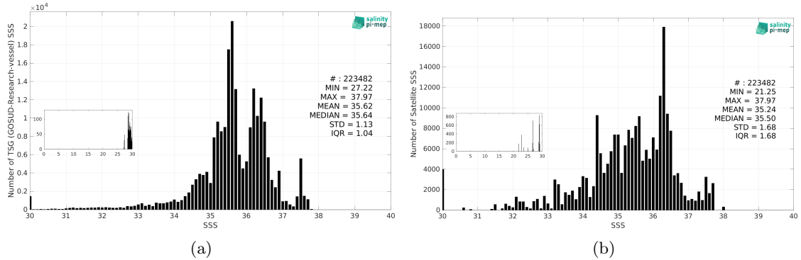
Figure 3: Histograms of SSS from TSG (GOSUD-Research-vessel) (a) and Aquarius SSS L3 OR v5 - 7-Day running (NASA-GSFC) (b) considering all match-up pairs per bins of 0.1 over the Atlantic Ocean Pi-MEP region and for the full satellite product period.
