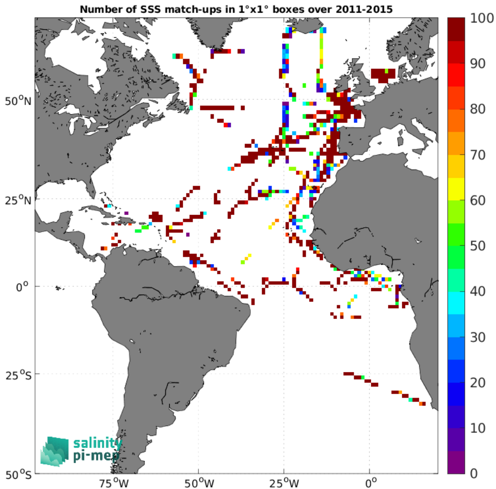
Figure 5: Number of SSS match-ups between TSG (GOSUD-Research-vessel) SSS and the Aquarius SSS L3 OR v5 - 7-Day running (NASA-GSFC) SSS product for the Atlantic Ocean Pi-MEP region over 1^\circ \times 1^\circ boxes and for the full satellite product period.
