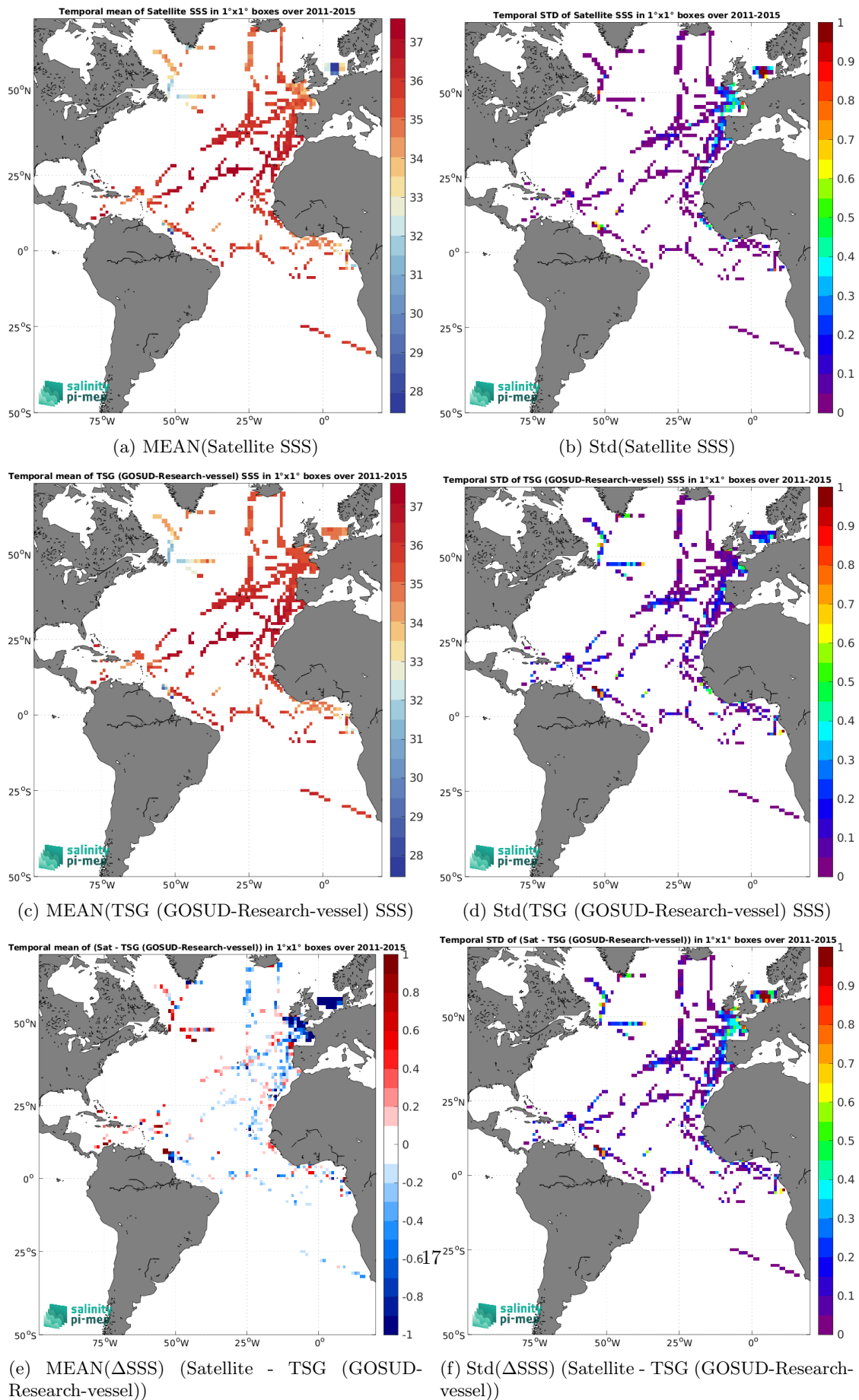
Figure 7: Temporal mean (left) and Std (right) of SSS from Aquarius SSS L3 OR v5 - 7-Day running (NASA-GSFC) (top), TSG (GOSUD-Research-vessel) (middle), and of \Delta SSS (Satellite - TSG (GOSUD-Research-vessel)). Only match-up pairs are used to generate these maps.
