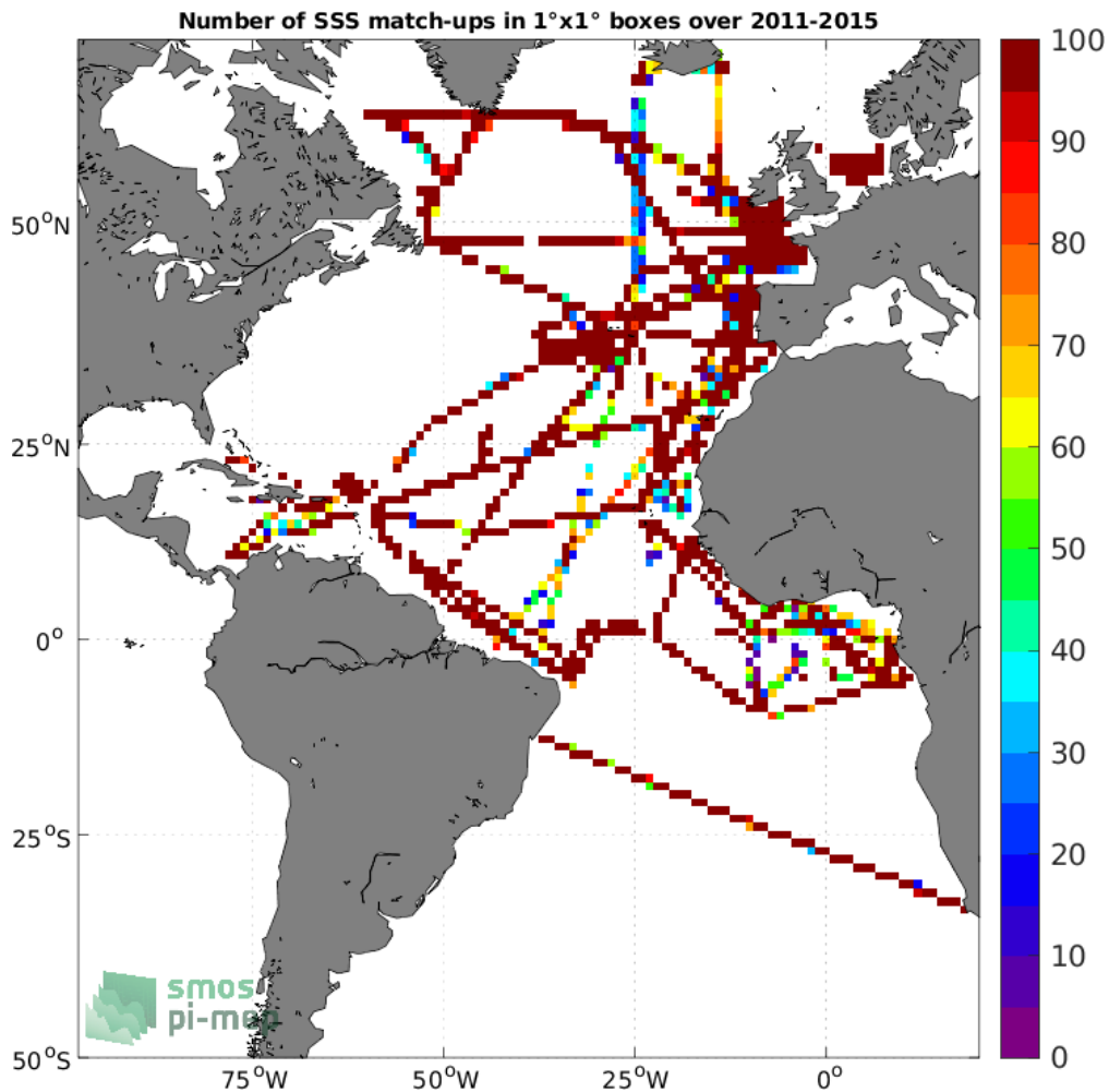
Figure 4: Number of SSS match-ups between TSG (GOSUD-Research-vessel) SSS and the Aquarius SSS L3 OR v5 - 7-Day running (NASA-GSFC) SSS product for the Atlantic Ocean Pi-MEP region over 1°x1° boxes and for the full satellite product period.
