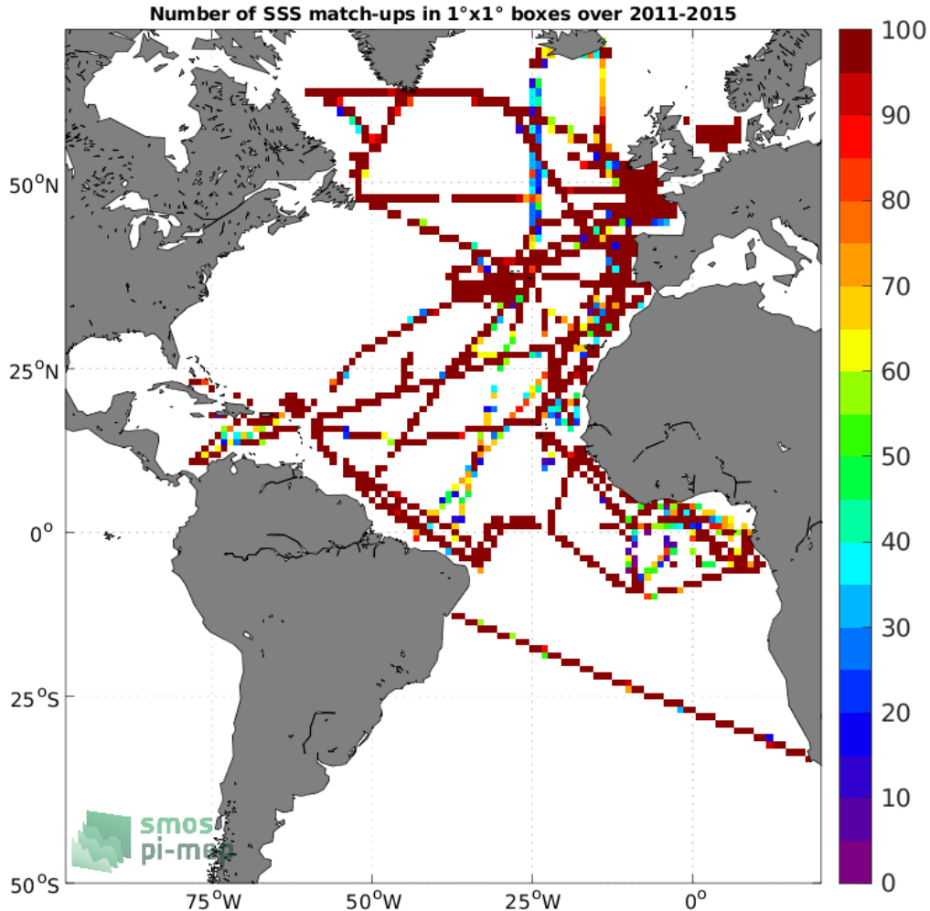
Figure 4: Number of SSS match-ups between TSG (GOSUD-Research-vessel) SSS and the Aquarius SSS L3 OR v5 - 7-Day running (NASA-GSFC) SSS product for the Atlantic Ocean Pi-MEP region over 1^\circ \times 1^\circ boxes and for the full satellite product period.
