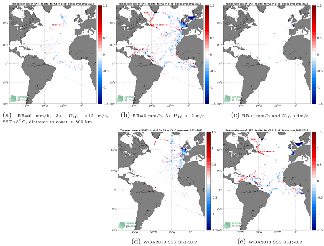
Figure 12: Temporal mean gridded over spatial boxes of size 1^\circ \times 1^\circ of \Delta SSS (Aquarius SSS L3 OR v5 - 7-Day running (NASA-GSFC) - TSG (GOSUD-Research-vessel)) for 5 different subdatasets corresponding to:RR=0 mm/h, 3 < U_{10} < 12 m/s, SST>5°C, distance to coast > 800 km (a), RR=0 mm/h, 3 < U_{10} < 12 m/s (b), RR>1mm/h and U_{10} < 4 m/s (c), WOA2013 SSS Std<0.2 (d), WOA2013 SSS Std>0.2 (e).
