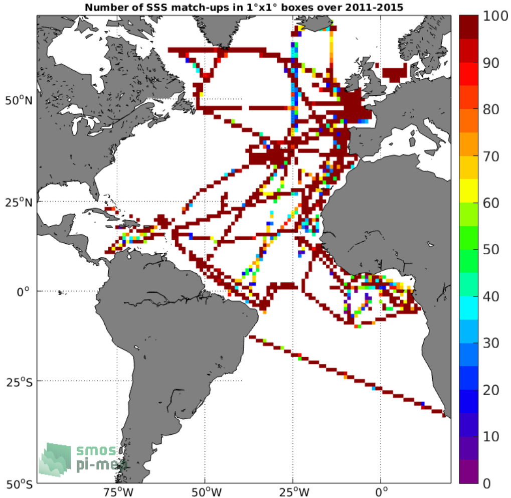
Figure 4: Number of SSS match-ups between TSG (GOSUD-Research-vessel) SSS and the Aquarius SSS L3 OR v5 - 7-Day running (NASA-GSFC) SSS product for the Atlantic Ocean Pi-MEP region over 1^\circ \times 1^\circ boxes and for the full satellite product period.
