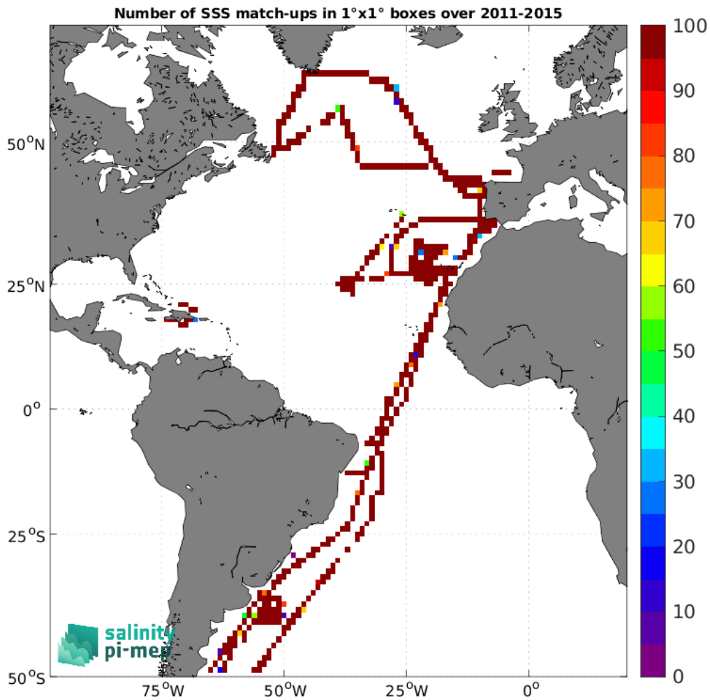
Figure 4: Number of SSS match-ups between TSG (CSIC-UTM) SSS and the Aquarius SSS L3 OR v5 - 7-Day running (NASA-GSFC) SSS product for the Atlantic Ocean Pi-MEP region over 1^\circ \times 1^\circ boxes and for the full satellite product period.
