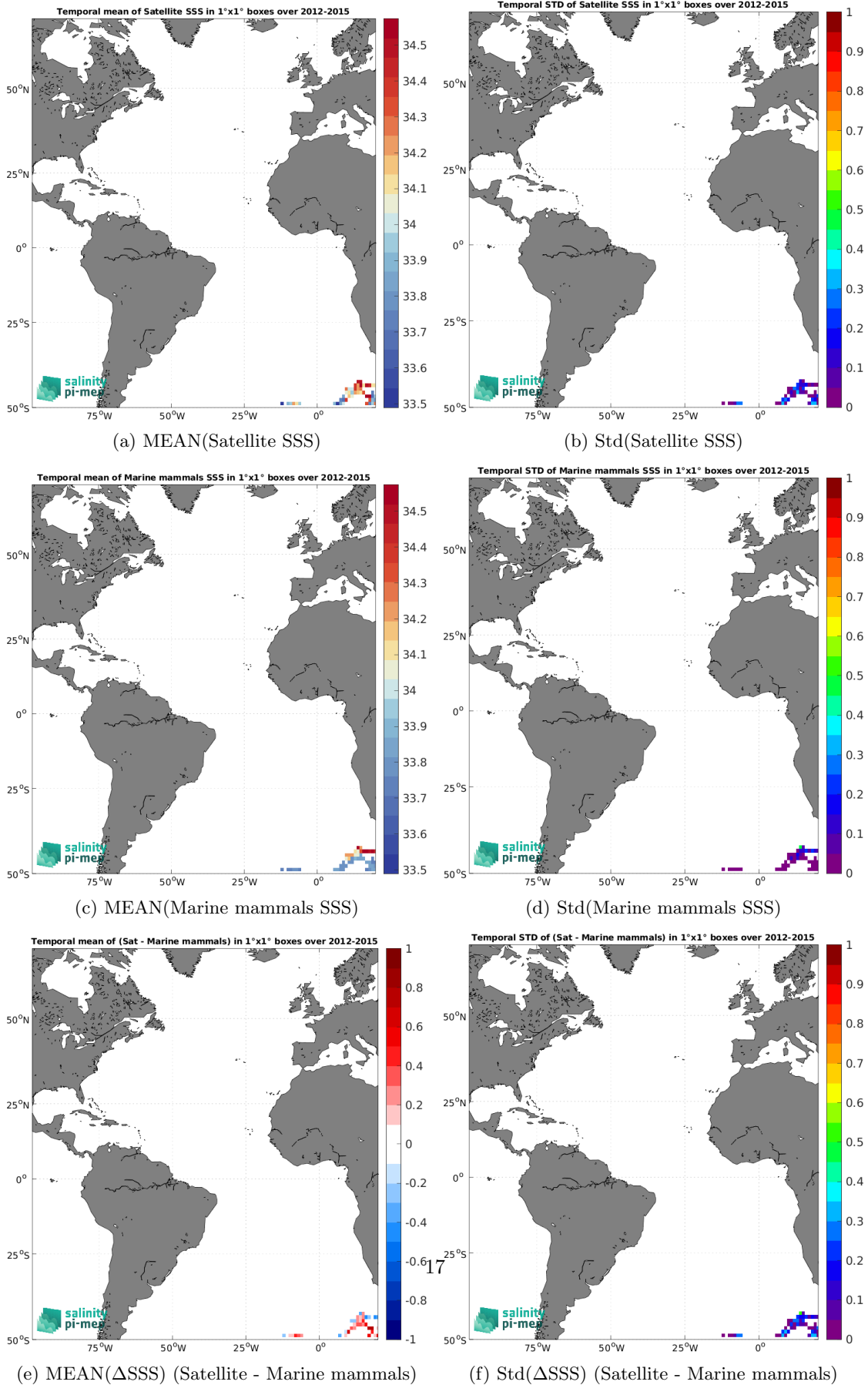
Figure 6: Temporal mean (left) and Std (right) of SSS from Aquarius SSS L3 OR v5 - 7-Day running (NASA-GSFC) (top), Marine mammals (middle), and of \Delta SSS (Satellite - Marine mammals). Only match-up pairs are used to generate these maps.
