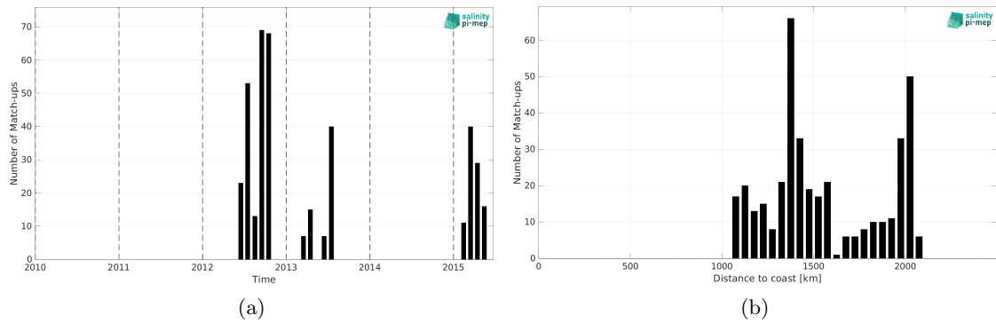
Figure 1: Number of match-ups between Marine mammals and Aquarius SSS L3 OR v5 - 7-Day running (NASA-GSFC) SSS as a function of time (a) and as function of the distance to coast (b) over the Atlantic Ocean Pi-MEP region and for the full satellite product period.
