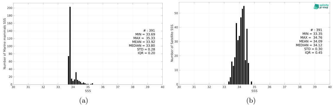
Figure 2: Histograms of SSS from Marine mammals (a) and Aquarius SSS L3 OR v5 - 7-Day running (NASA-GSFC) (b) considering all match-up pairs per bins of 0.1 over the Atlantic Ocean Pi-MEP region and for the full satellite product period.
