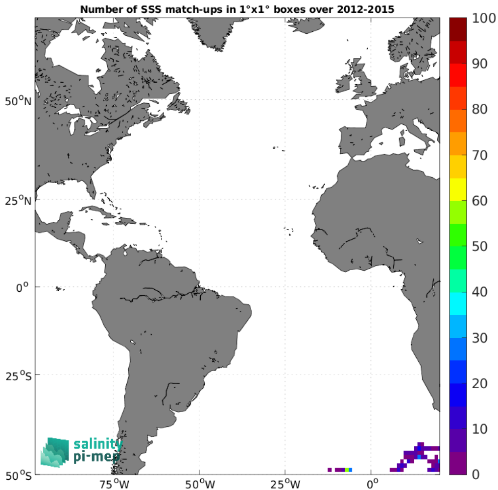
Figure 4: Number of SSS match-ups between Marine mammals SSS and the Aquarius SSS L3 OR v5 - 7-Day running (NASA-GSFC) SSS product for the Atlantic Ocean Pi-MEP region over 1°×1° boxes and for the full satellite product period.
