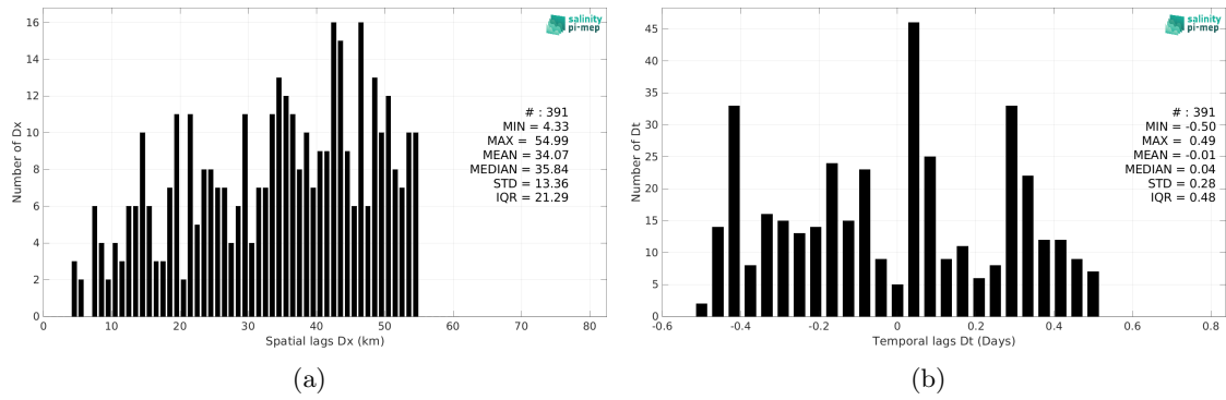
Figure 5: Histograms of the spatial (a) and temporal (b) lags between the location/time of the Marine mammals measurement and the date of the corresponding Aquarius SSS L3 OR v5 - 7-Day running (NASA-GSFC) SSS pixel.
