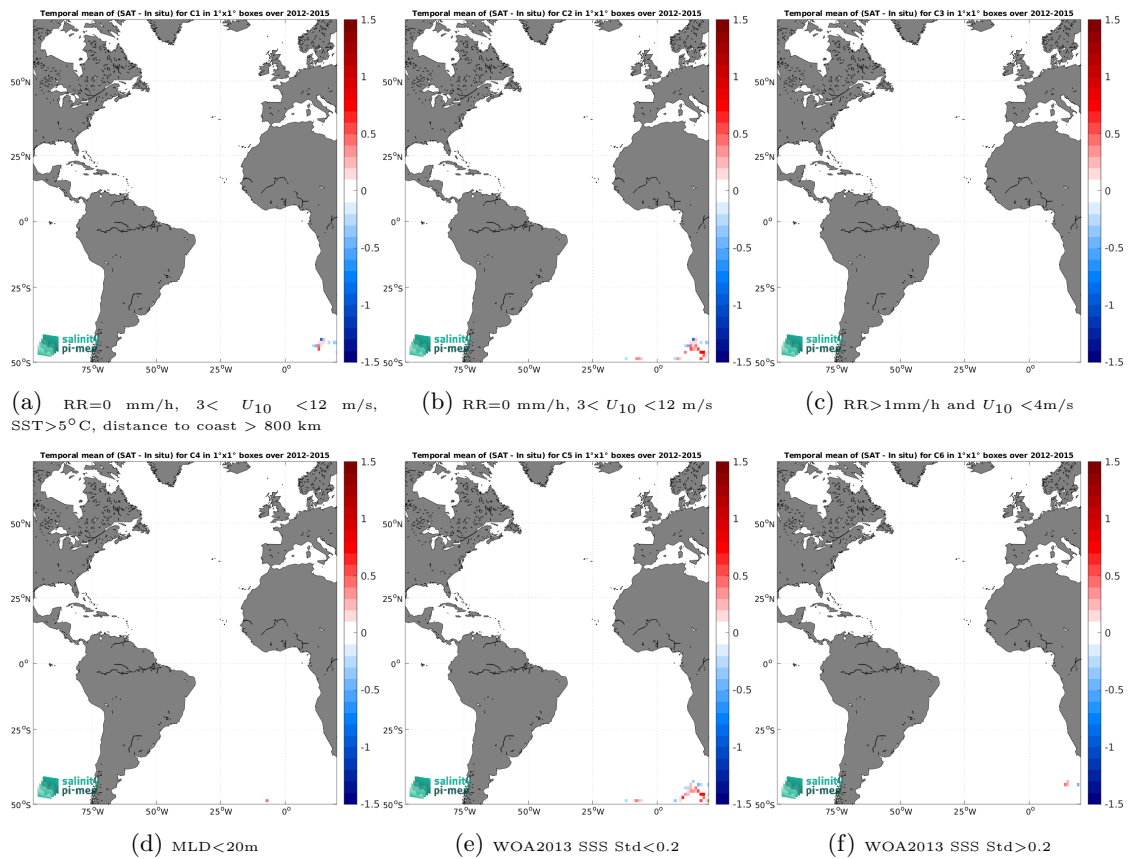
Figure 12: Temporal mean gridded over spatial boxes of size 1^\circ \times 1^\circ of \Delta SSS (Aquarius SSS L3 OR v5 - 7-Day running (NASA-GSFC) - Marine mammals) for 6 different subdatasets corresponding to: RR=0 mm/h, 3 < U_{10} < 12 m/s, SST > 5°C, distance to coast > 800 km (a), RR=0 mm/h, 3 < U_{10} < 12 m/s (b), RR > 1mm/h and U_{10} < 4 m/s (c), MLD < 20m (d), WOA2013 SSS Std < 0.2 (e), WOA2013 SSS Std > 0.2 (f).
