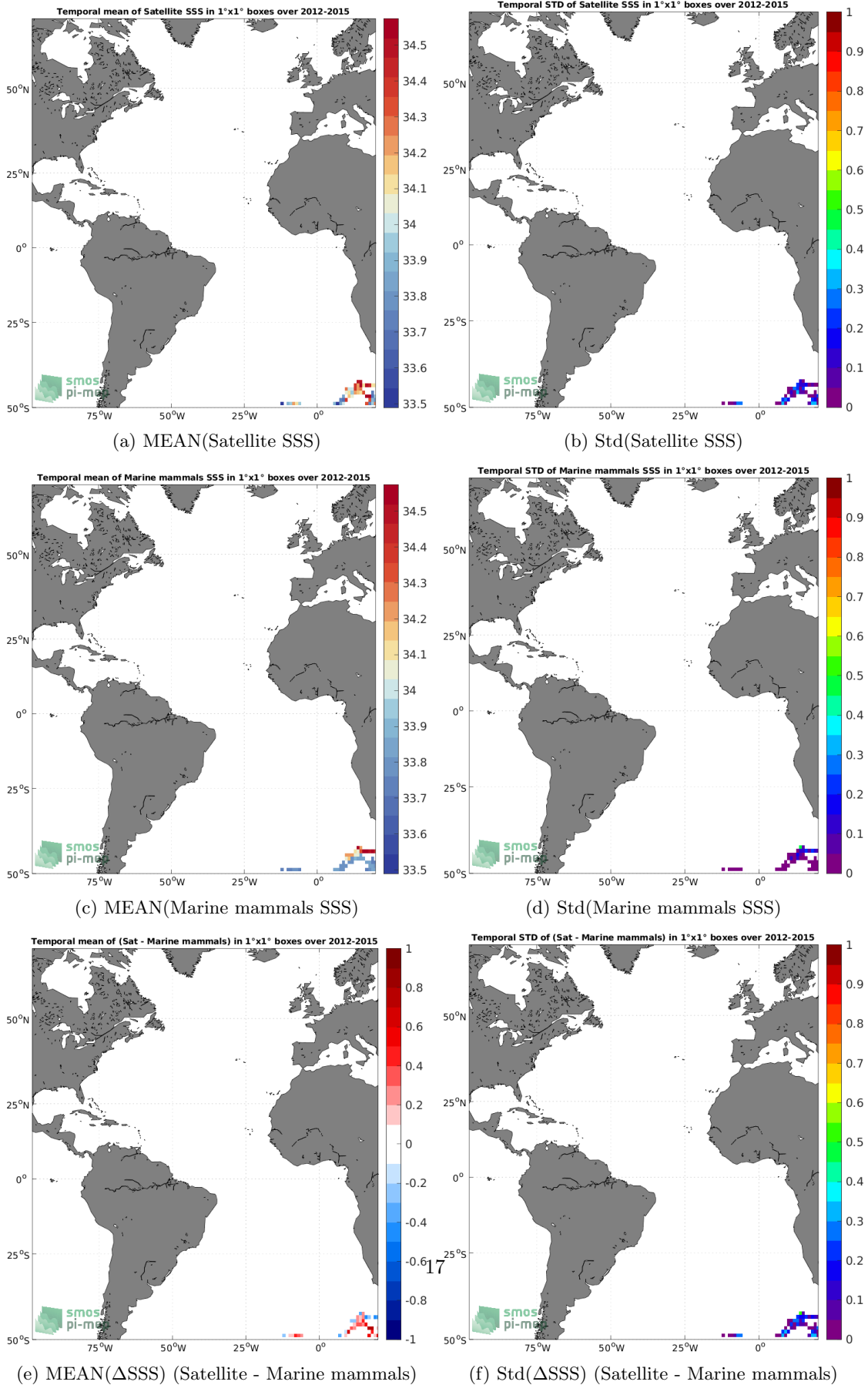
(e) MEAN( \Delta SSS) (Satellite - Marine mammals) (f) Std( \Delta SSS) (Satellite - Marine mammals) Figure 6: Temporal mean (left) and Std (right) of SSS from Aquarius SSS L3 OR v5 - 7-Day running (NASA-GSFC) (top), Marine mammals (middle), and of \Delta SSS (Satellite - Marine mammals). Only match-up pairs are used to generate these maps.
