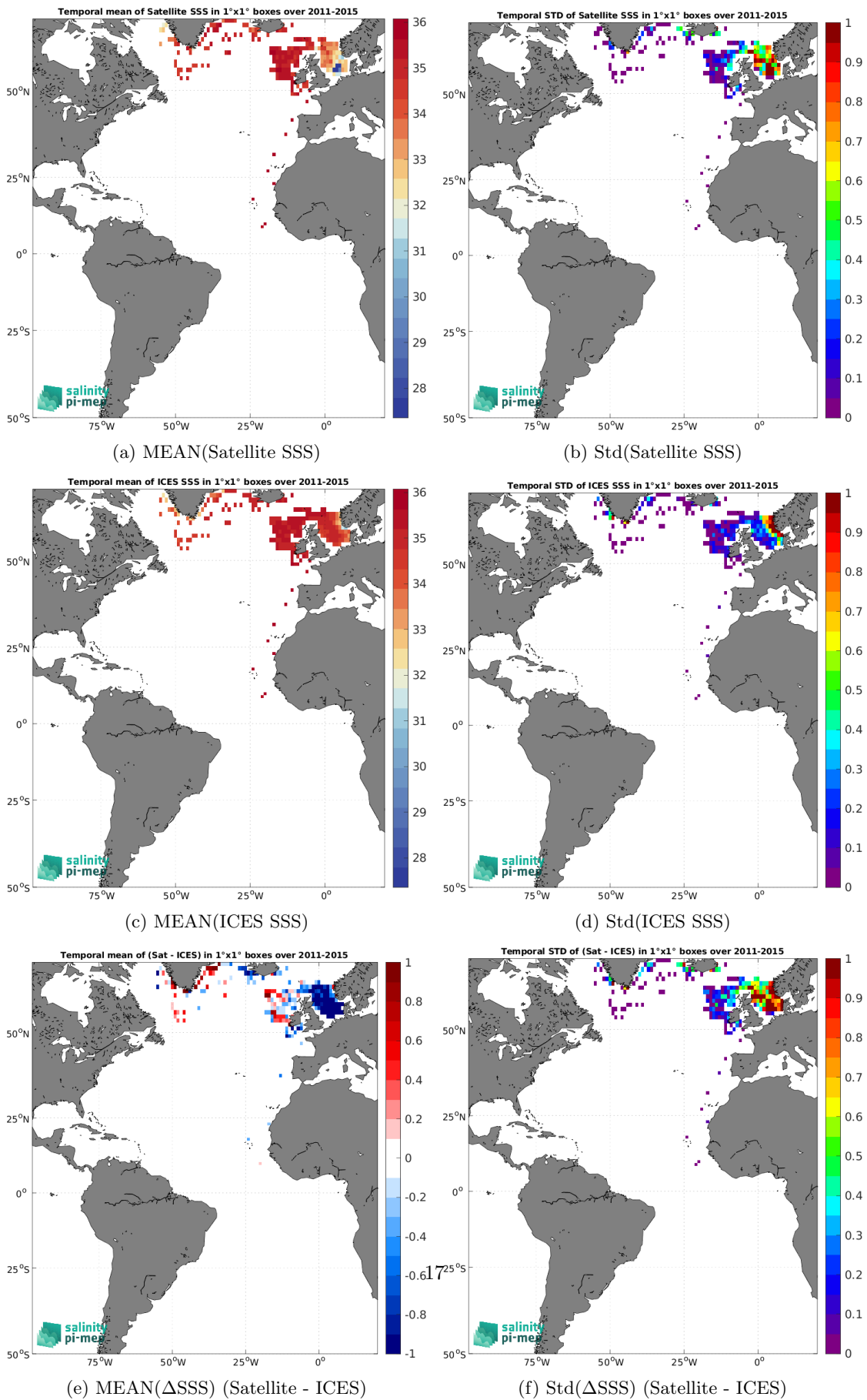
Figure 7: Temporal mean (left) and Std (right) of SSS from Aquarius SSS L3 OR v5 - 7-Day running (NASA-GSFC) (top), ICES (middle), and of \Delta SSS (Satellite - ICES). Only match-up pairs are used to generate these maps.
