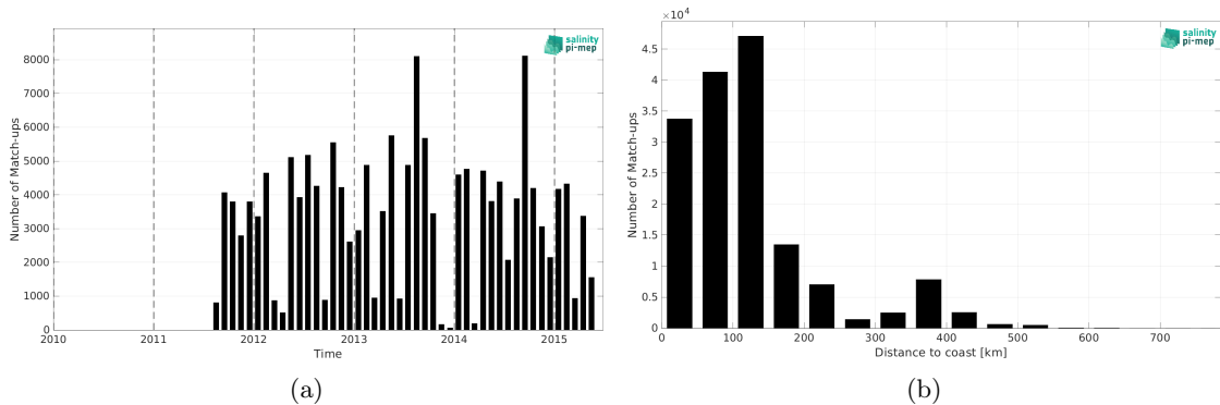
Figure 2: Number of match-ups between ICES and Aquarius SSS L3 OR v5 - 7-Day running (NASA-GSFC) SSS as a function of time (a) and as function of the distance to coast (b) over the Atlantic Ocean Pi-MEP region and for the full satellite product period.
