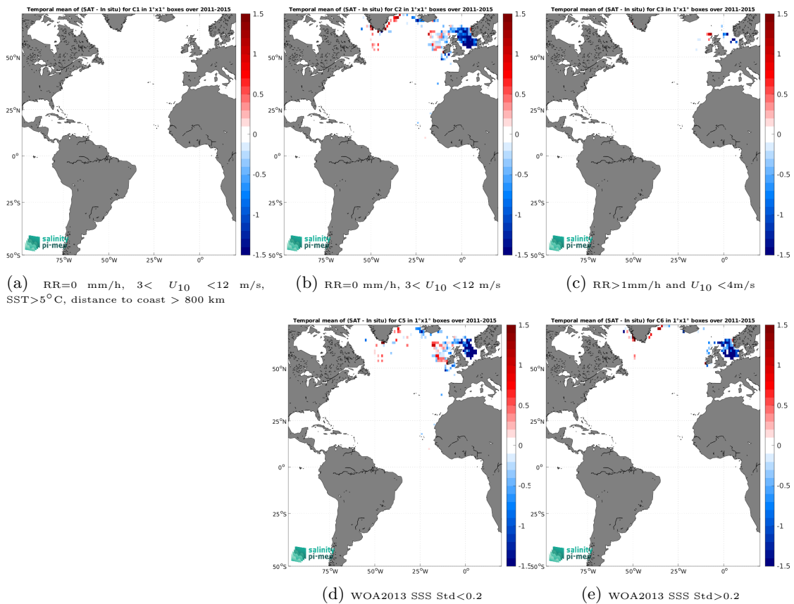
Figure 14: Temporal mean gridded over spatial boxes of size 1^\circ \times 1^\circ of \Delta SSS (Aquarius SSS L3 OR v5 - 7-Day running (NASA-GSFC) - ICES) for 5 different subdatasets corresponding to:RR=0 mm/h, 3 < U_{10} < 12 m/s, SST >5^\circ\text{C} , distance to coast > 800 km (a), RR=0 mm/h, 3 < U_{10} < 12 m/s (b), RR >1 mm/h and U_{10} < 4 m/s (c), WOA2013 SSS Std <0.2 (d), WOA2013 SSS Std >0.2 (e).
