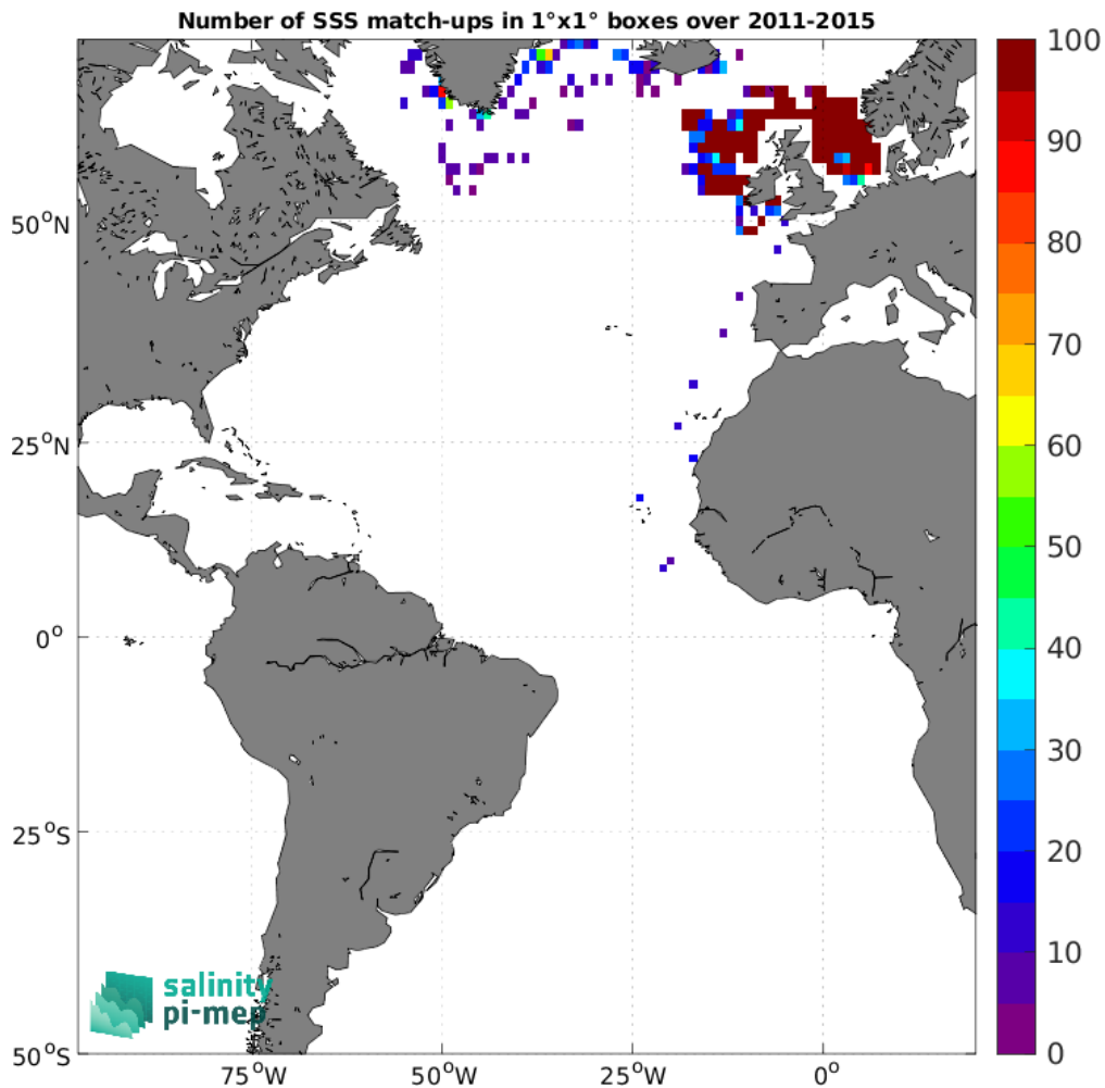
Figure 5: Number of SSS match-ups between ICES SSS and the Aquarius SSS L3 OR v5 - 7-Day running (NASA-GSFC) SSS product for the Atlantic Ocean Pi-MEP region over 1°×1° boxes and for the full satellite product period.
