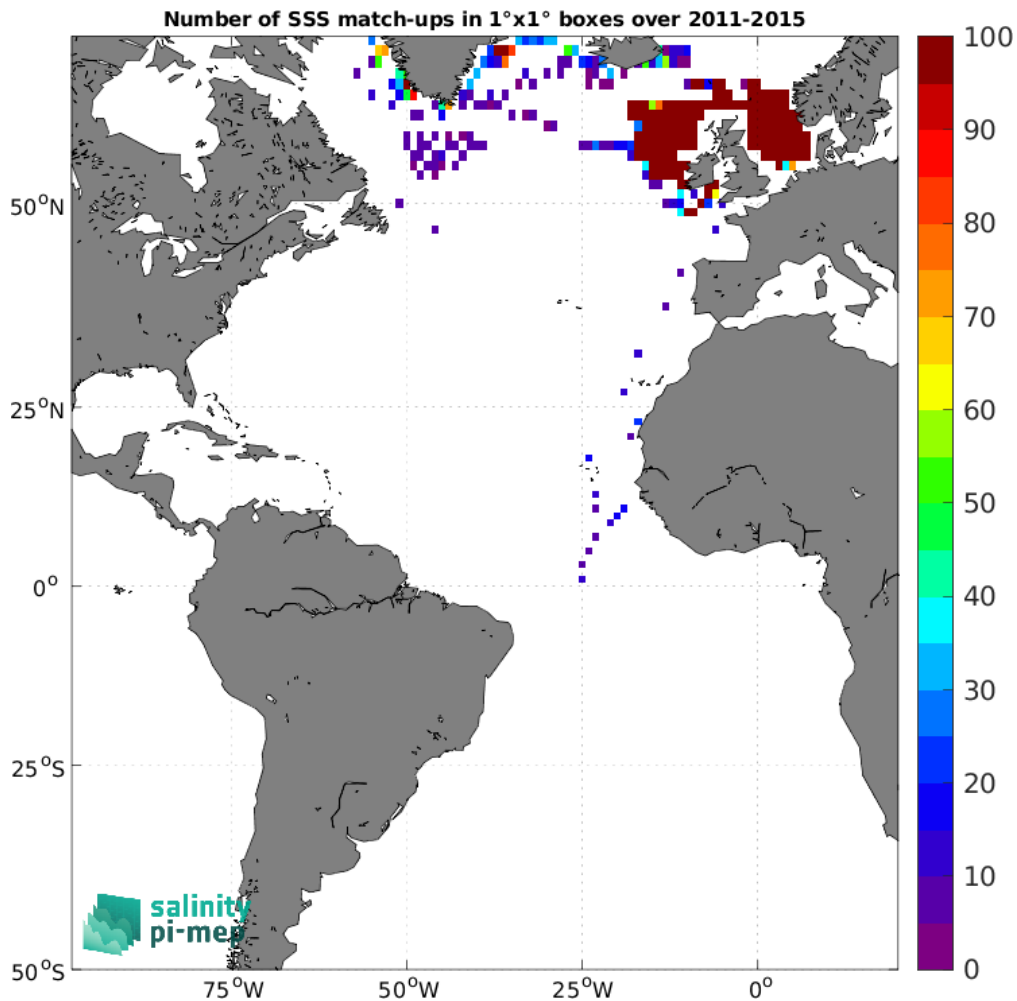
Figure 4: Number of SSS match-ups between ICES SSS and the Aquarius SSS L3 OR v5 - 7-Day running (NASA-GSFC) SSS product for the Atlantic Ocean Pi-MEP region over 1°×1° boxes and for the full satellite product period.
