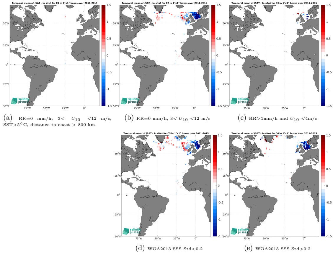
Figure 12: Temporal mean gridded over spatial boxes of size 1^\circ \times 1^\circ of \Delta\text{SSS} (Aquarius SSS L3 OR v5 - 7-Day running (NASA-GSFC) - ICES) for 5 different subdatasets corresponding to:RR=0 mm/h, 3 < U_{10} < 12 m/s, SST >5^\circ\text{C} , distance to coast > 800 km (a), RR=0 mm/h, 3 < U_{10} < 12 m/s (b), RR >1 mm/h and U_{10} < 4 m/s (c), WOA2013 SSS Std <0.2 (d), WOA2013 SSS Std >0.2 (e).
