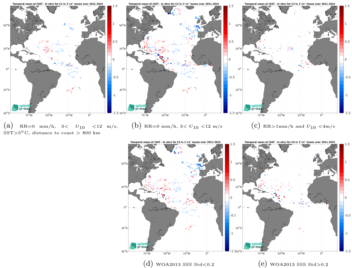
Figure 13: Temporal mean gridded over spatial boxes of size 1^\circ \times 1^\circ of \Delta SSS (Aquarius SSS L3 OR v5 - 7-Day running (NASA-GSFC) - Surface drifters) for 5 different subdatasets corresponding to:RR=0 mm/h, 3 < U_{10} < 12 m/s, SST >5^\circ\text{C} , distance to coast > 800 km (a), RR=0 mm/h, 3 < U_{10} < 12 m/s (b), RR >1 mm/h and U_{10} < 4 m/s (c), WOA2013 SSS Std <0.2 (d), WOA2013 SSS Std >0.2 (e).
