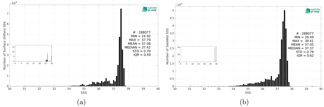
Figure 3: Histograms of SSS from Surface drifters (a) and Aquarius SSS L3 OR v5 - 7-Day running (NASA-GSFC) (b) considering all match-up pairs per bins of 0.1 over the Atlantic Ocean Pi-MEP region and for the full satellite product period.
