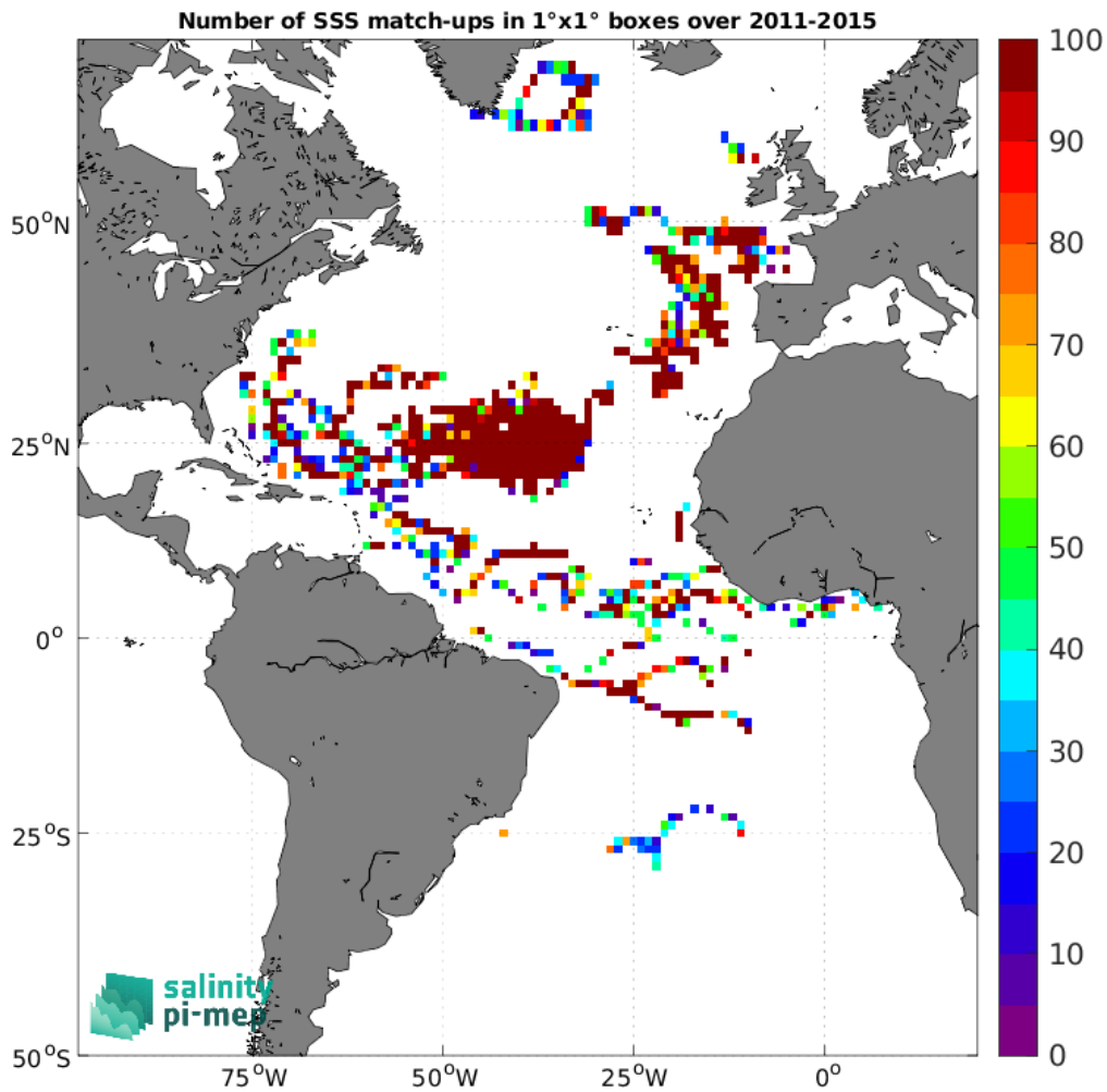
Figure 4: Number of SSS match-ups between Surface drifters SSS and the Aquarius SSS L3 OR v5 - 7-Day running (NASA-GSFC) SSS product for the Atlantic Ocean Pi-MEP region over 1°×1° boxes and for the full satellite product period.
