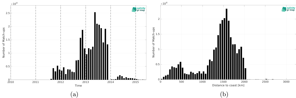
Figure 2: Number of match-ups between Surface drifters and Aquarius SSS L3 OR v5 - 7-Day running (NASA-GSFC) SSS as a function of time (a) and as function of the distance to coast (b) over the Atlantic Ocean Pi-MEP region and for the full satellite product period.
