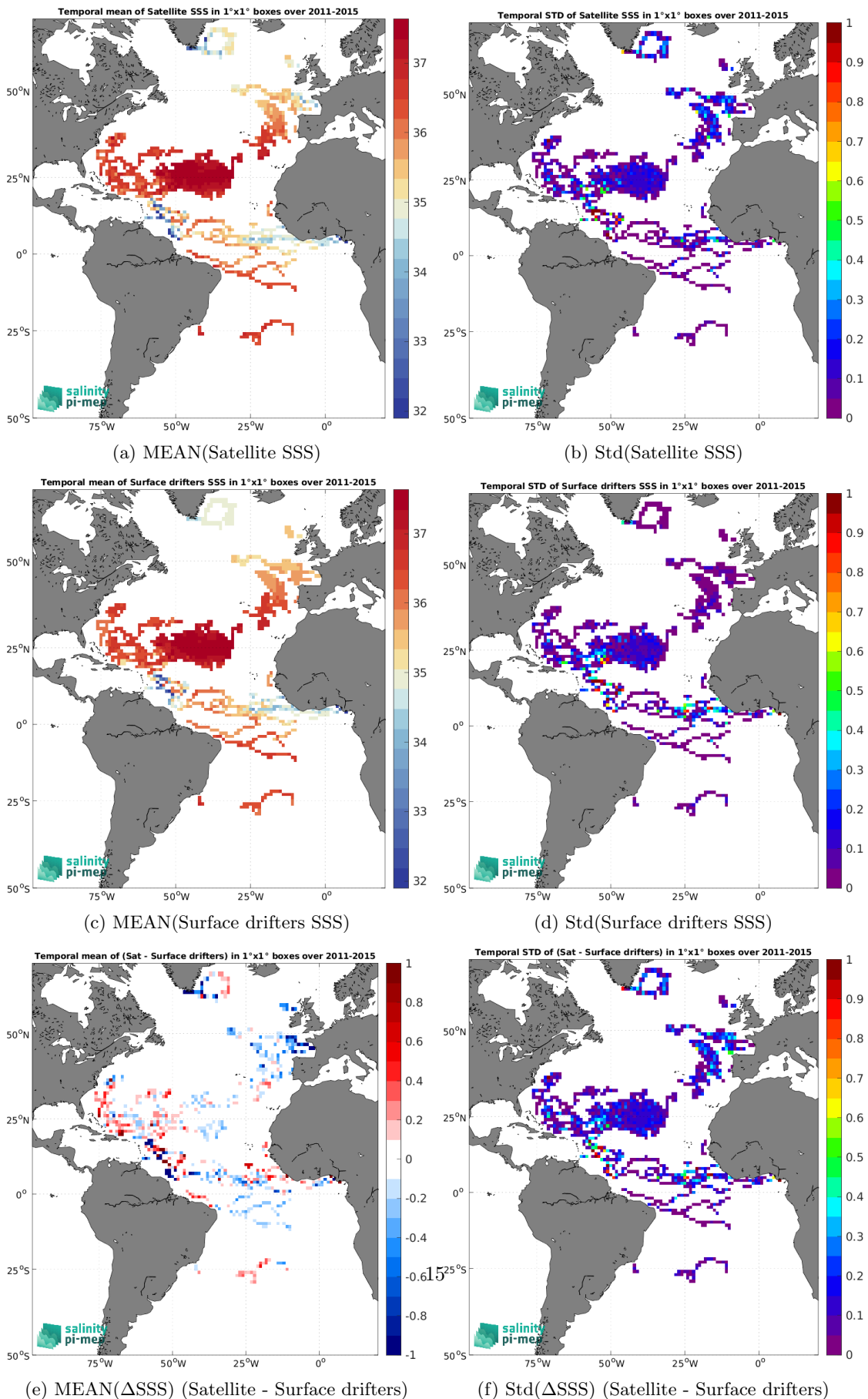
Figure 5: Temporal mean (left) and Std (right) of SSS from Aquarius SSS L3 OR v5 - 7-Day running (NASA-GSFC) (top), Surface drifters (middle), and of \Delta SSS (Satellite - Surface drifters). Only match-up pairs are used to generate these maps.
