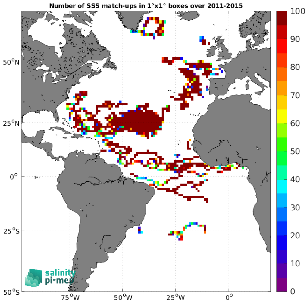
Figure 3: Number of SSS match-ups between Surface drifters SSS and the Aquarius SSS L3 OR v5 - 7-Day running (NASA-GSFC) SSS product for the Atlantic Ocean Pi-MEP region over 1°×1° boxes and for the full satellite product period.
