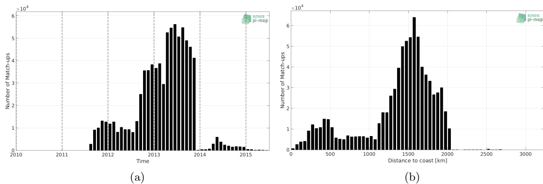
Figure 1: Number of match-ups between Surface drifters and Aquarius-L3-OR-V5-7DAY-RUNNING-1DEG SSS as a function of time (a) and as function of the distance to coast (b) over the Atlantic Ocean Pi-MEP region and for the full satellite product period.
