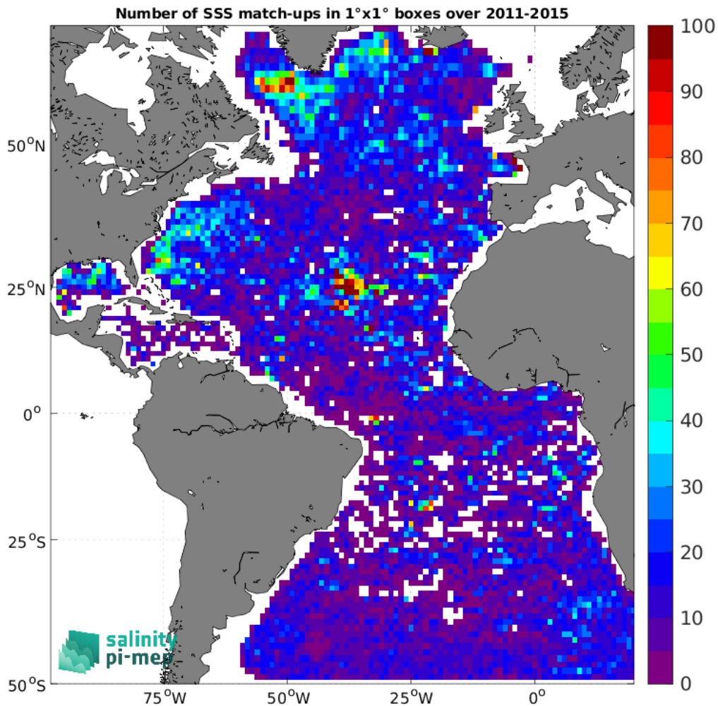
Figure 4: Number of SSS match-ups between Argo SSS and the Aquarius SSS L3 OR v5 - 7-Day running (NASA-GSFC) SSS product for the Atlantic Ocean Pi-MEP region over 1^\circ \times 1^\circ boxes and for the full satellite product period.
