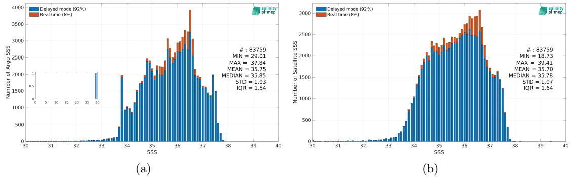
Figure 2: Histograms of SSS from Argo (a) and Aquarius SSS L3 OR v5 - 7-Day running (NASA-GSFC) (b) considering all match-up pairs per bins of 0.1 over the Atlantic Ocean Pi-MEP region and for the full satellite product period.
