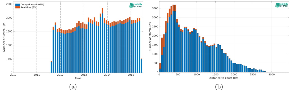
Figure 1: Number of match-ups between Argo and Aquarius SSS L3 OR v5 - 7-Day running (NASA-GSFC) SSS as a function of time (a) and as function of the distance to coast (b) over the Atlantic Ocean Pi-MEP region and for the full satellite product period.
