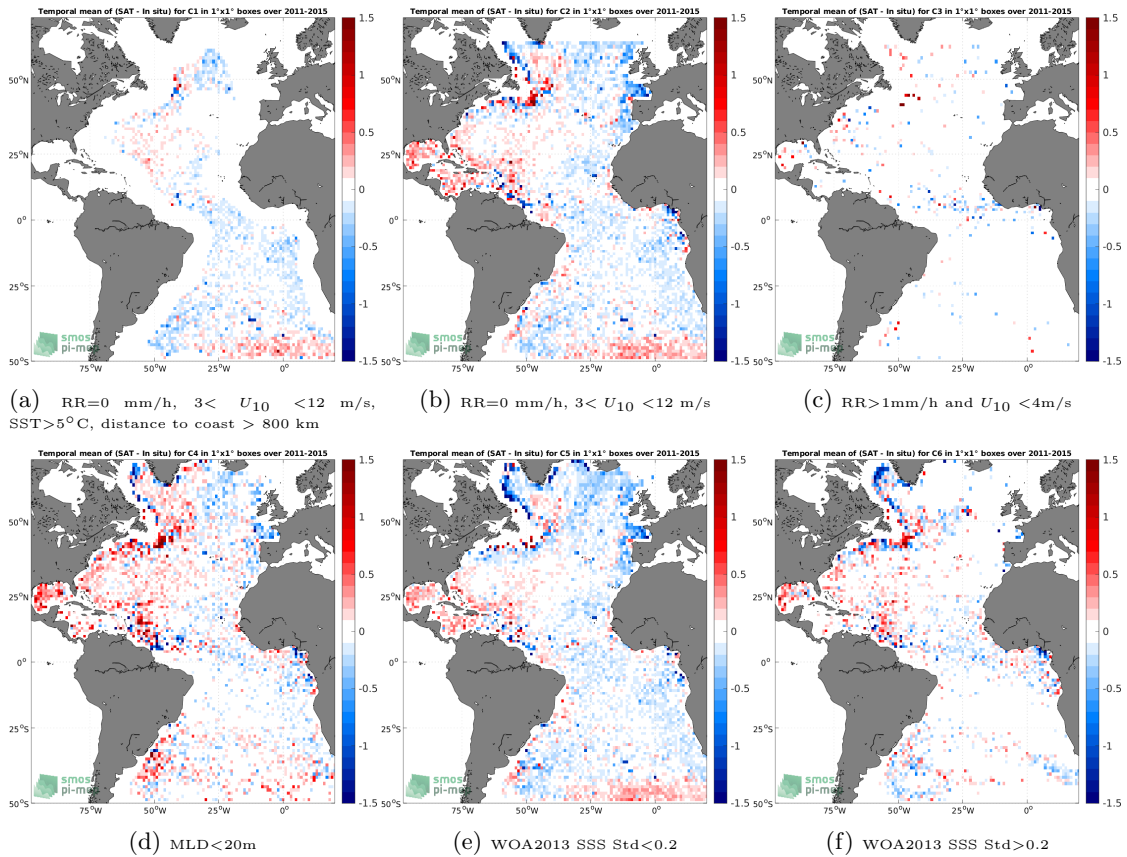
Figure 12: Temporal mean gridded over spatial boxes of size 1^\circ \times 1^\circ of \Delta SSS (Aquarius SSS L3 OR v5 - 7-Day running (NASA-GSFC) - Argo) for 6 different subdatasets corresponding to:RR=0 mm/h, 3 < U_{10} < 12 m/s, SST>5°C, distance to coast > 800 km (a), RR=0 mm/h, 3 < U_{10} < 12 m/s (b), RR>1mm/h and U_{10} < 4 m/s (c),MLD<20m (d),WOA2013 SSS Std<0.2 (e),WOA2013 SSS Std>0.2 (f).
