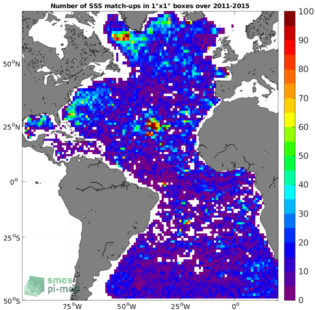
Figure 4: Number of SSS match-ups between Argo SSS and the Aquarius SSS L3 OR v5 - 7-Day running (NASA-GSFC) SSS product for the Atlantic Ocean Pi-MEP region over 1°x1° boxes and for the full satellite product period.
