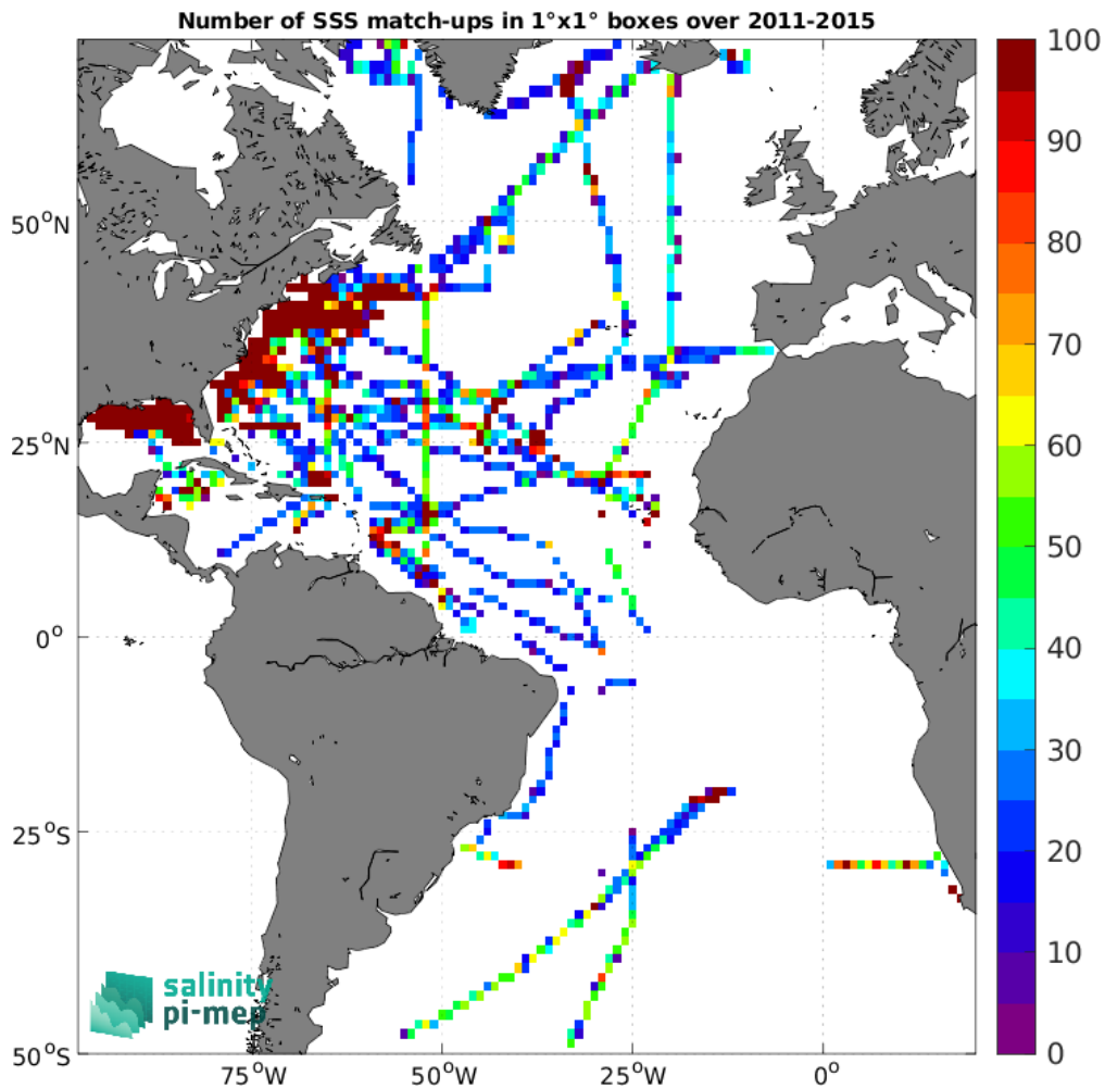
Figure 5: Number of SSS match-ups between TSG (SAMOS) SSS and the Aquarius SSS L3 OR v5 - 7-Day running - Rain mask (NASA-GSFC) SSS product for the Atlantic Ocean Pi-MEP region over 1^\circ \times 1^\circ boxes and for the full satellite product period.
