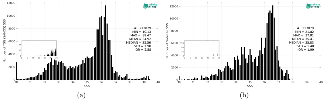
Figure 3: Histograms of SSS from TSG (SAMOS) (a) and Aquarius SSS L3 OR v5 - 7-Day running - Rain mask (NASA-GSFC) (b) considering all match-up pairs per bins of 0.1 over the Atlantic Ocean Pi-MEP region and for the full satellite product period.
