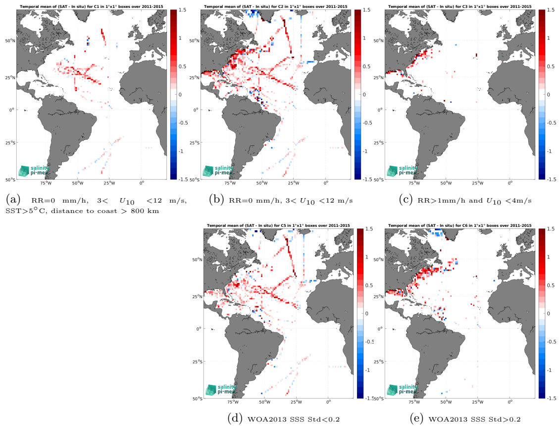
Figure 14: Temporal mean gridded over spatial boxes of size 1^\circ \times 1^\circ of \Delta SSS (Aquarius SSS L3 OR v5 - 7-Day running - Rain mask (NASA-GSFC) - TSG (SAMOS)) for 5 different subdatasets corresponding to:RR=0 mm/h, 3 < U_{10} < 12 m/s, SST >5^\circ\text{C} , distance to coast > 800 km (a), RR=0 mm/h, 3 < U_{10} < 12 m/s (b), RR >1 mm/h and U_{10} < 4 m/s (c), WOA2013 SSS Std <0.2 (d), WOA2013 SSS Std >0.2 (e).
