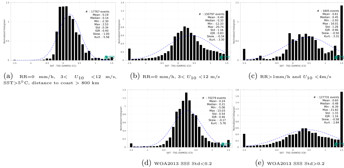
Figure 15: Normalized histogram of \Delta\text{SSS} (Aquarius SSS L3 OR v5 - 7-Day running - Rain mask (NASA-GSFC) - TSG (SAMOS)) for 5 different subdatasets corresponding to: RR=0 mm/h, 3 < U_{10} < 12 m/s, SST>5°C, distance to coast > 800 km (a), RR=0 mm/h, 3 < U_{10} < 12 m/s (b), RR>1mm/h and U_{10} < 4 m/s (c), WOA2013 SSS Std<0.2 (d), WOA2013 SSS Std>0.2 (e).
