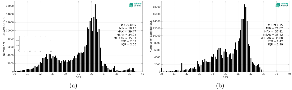
Figure 2: Histograms of SSS from TSG (SAMOS) (a) and Aquarius SSS L3 OR v5 - 7-Day running - Rain mask (NASA-GSFC) (b) considering all match-up pairs per bins of 0.1 over the Atlantic Ocean Pi-MEP region and for the full satellite product period.
