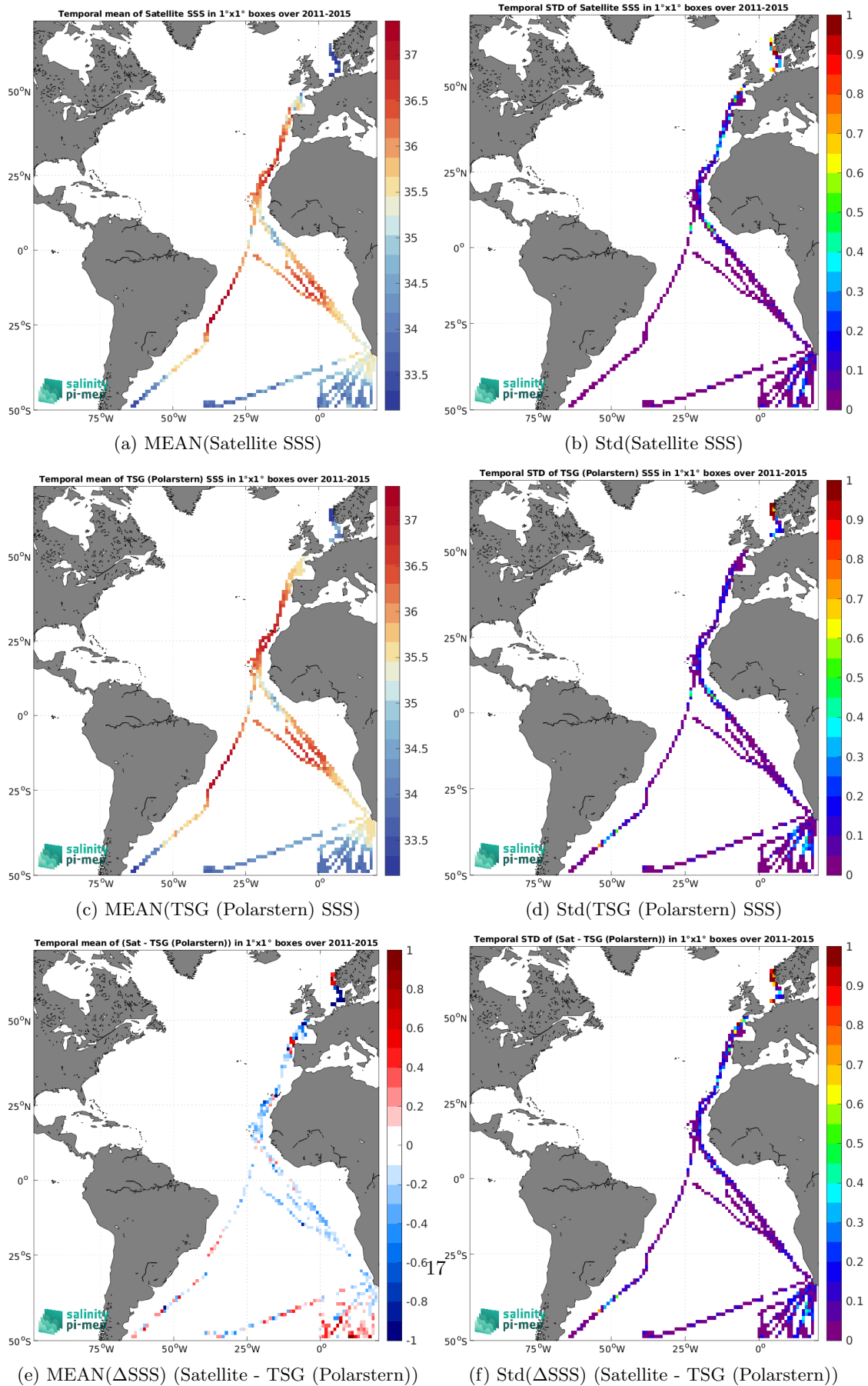
Figure 7: Temporal mean (left) and Std (right) of SSS from Aquarius SSS L3 OR v5 - 7-Day running - Rain mask (NASA-GSFC) (top), TSG (Polarstern) (middle), and of \Delta SSS (Satellite - TSG (Polarstern)). Only match-up pairs are used to generate these maps.
