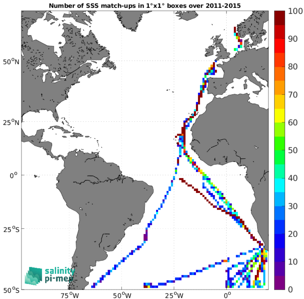
Figure 5: Number of SSS match-ups between TSG (Polarstern) SSS and the Aquarius SSS L3 OR v5 - 7-Day running - Rain mask (NASA-GSFC) SSS product for the Atlantic Ocean Pi-MEP region over 1^\circ \times 1^\circ boxes and for the full satellite product period.
