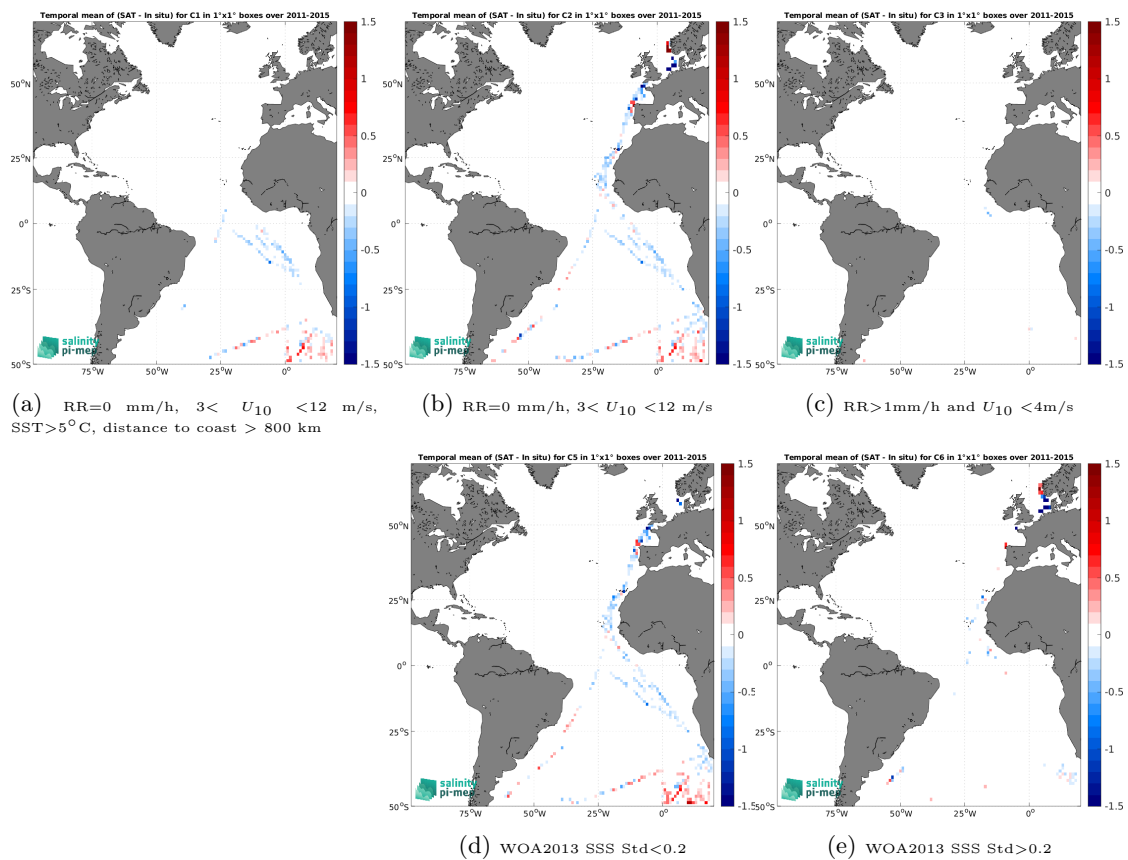
Figure 14: Temporal mean gridded over spatial boxes of size 1^\circ \times 1^\circ of \Delta SSS (Aquarius SSS L3 OR v5 - 7-Day running - Rain mask (NASA-GSFC) - TSG (Polarstern)) for 5 different subdatasets corresponding to:RR=0 mm/h, 3 < U_{10} < 12 m/s, SST >5^\circ\text{C} , distance to coast > 800 km (a), RR=0 mm/h, 3 < U_{10} < 12 m/s (b), RR >1 mm/h and U_{10} < 4 m/s (c), WOA2013 SSS Std <0.2 (d), WOA2013 SSS Std >0.2 (e).
