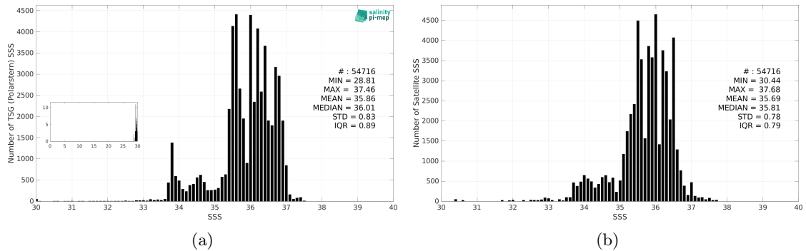
Figure 3: Histograms of SSS from TSG (Polarstern) (a) and Aquarius SSS L3 OR v5 - 7-Day running - Rain mask (NASA-GSFC) (b) considering all match-up pairs per bins of 0.1 over the Atlantic Ocean Pi-MEP region and for the full satellite product period.
