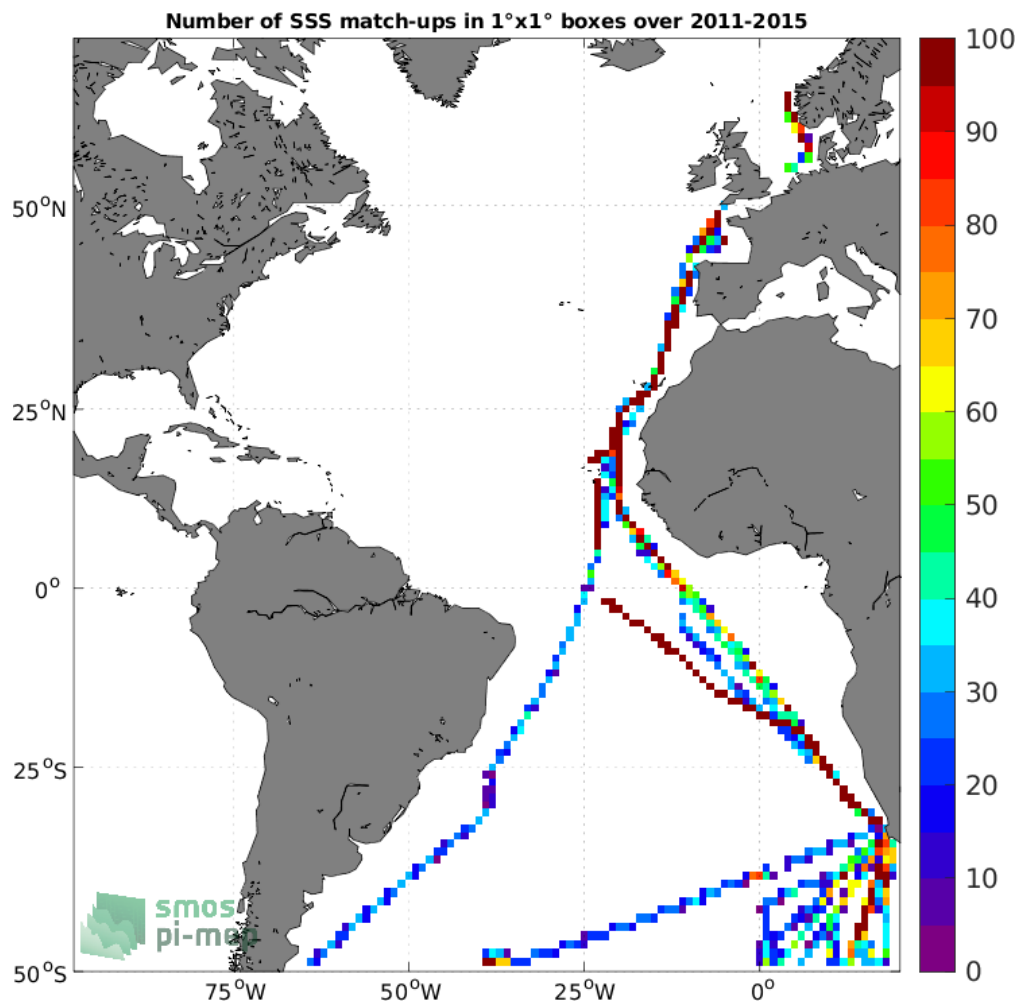
Figure 4: Number of SSS match-ups between TSG (Polarstern) SSS and the Aquarius SSS L3 OR v5 - 7-Day running - Rain mask (NASA-GSFC) SSS product for the Atlantic Ocean Pi-MEP region over 1°x1° boxes and for the full satellite product period.
