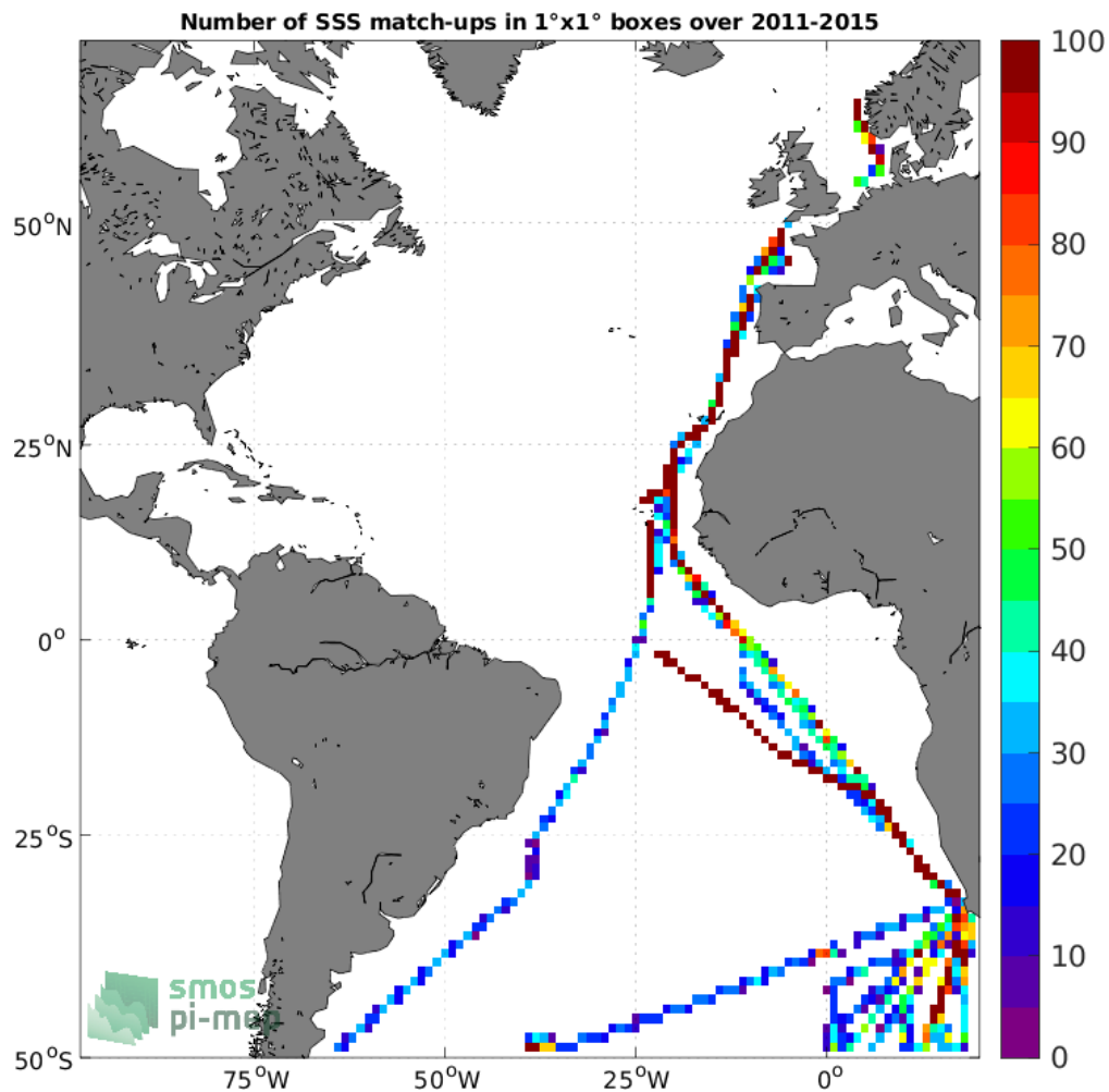
Figure 4: Number of SSS match-ups between TSG (Polarstern) SSS and the Aquarius SSS L3 OR v5 - 7-Day running - Rain mask (NASA-GSFC) SSS product for the Atlantic Ocean Pi-MEP region over 1^\circ \times 1^\circ boxes and for the full satellite product period.
