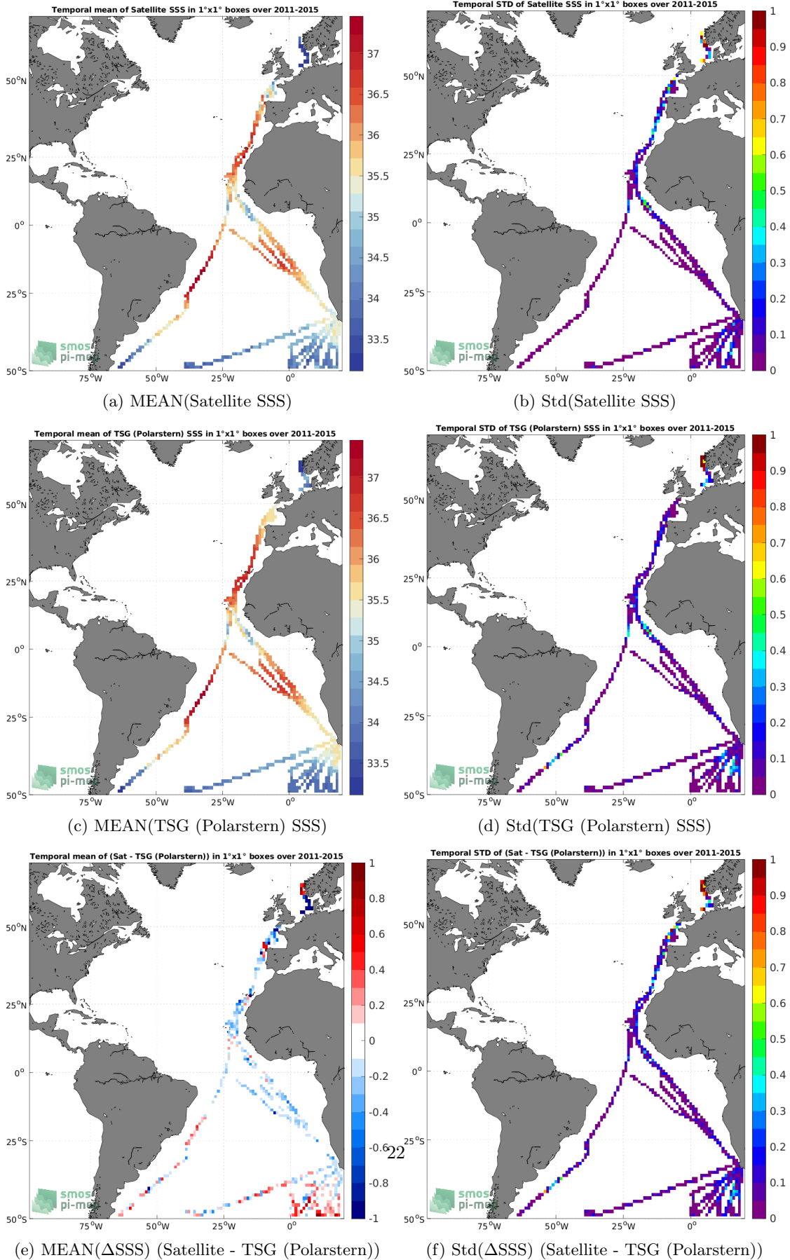
Figure 6: Temporal mean (left) and Std (right) of SSS from Aquarius SSS L3 OR v5 - 7-Day running - Rain mask (NASA-GSFC) (top), TSG (Polarstern) (middle), and of \Delta SSS (Satellite - TSG (Polarstern)). Only match-up pairs are used to generate these maps.
