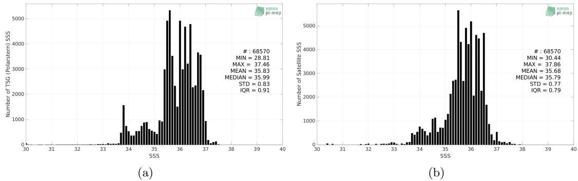
Figure 2: Histograms of SSS from TSG (Polarstern) (a) and Aquarius SSS L3 OR v5 - 7-Day running - Rain mask (NASA-GSFC) (b) considering all match-up pairs per bins of 0.1 over the Atlantic Ocean Pi-MEP region and for the full satellite product period.
