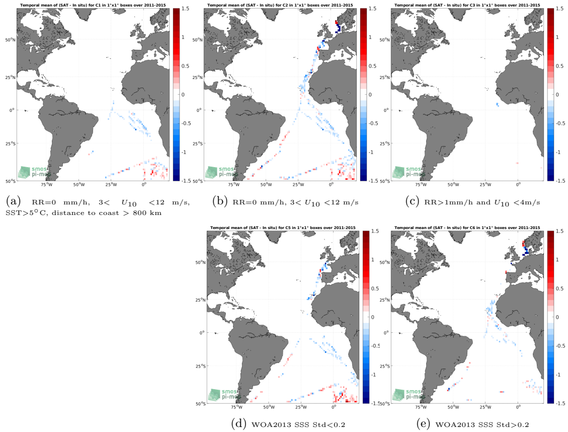
Figure 12: Temporal mean gridded over spatial boxes of size 1^\circ \times 1^\circ of \Delta SSS (Aquarius SSS L3 OR v5 - 7-Day running - Rain mask (NASA-GSFC) - TSG (Polarstern)) for 5 different subdatasets corresponding to:RR=0 mm/h, 3 < U_{10} < 12 m/s, SST >5^\circ\text{C} , distance to coast > 800 km (a), RR=0 mm/h, 3 < U_{10} < 12 m/s (b), RR >1 mm/h and U_{10} < 4 m/s (c), WOA2013 SSS Std <0.2 (d), WOA2013 SSS Std >0.2 (e).
