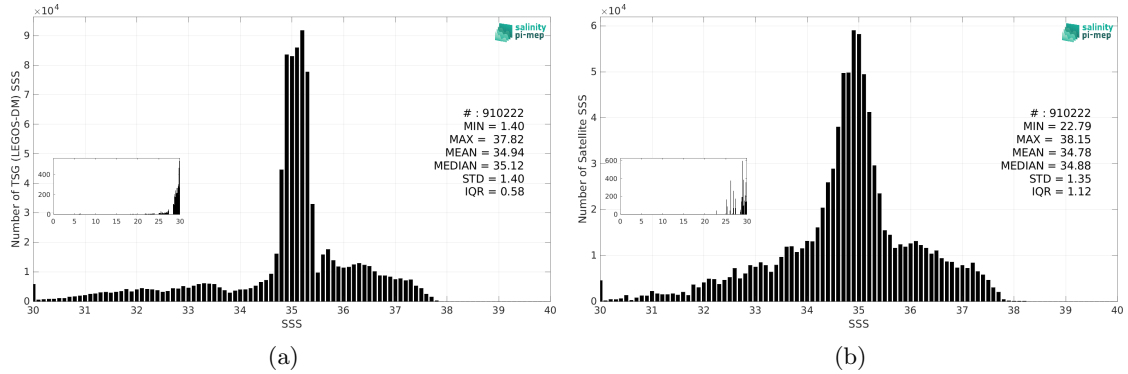
Figure 3: Histograms of SSS from TSG (LEGOS-DM) (a) and Aquarius SSS L3 OR v5 - 7-Day running - Rain mask (NASA-GSFC) (b) considering all match-up pairs per bins of 0.1 over the Atlantic Ocean Pi-MEP region and for the full satellite product period.
