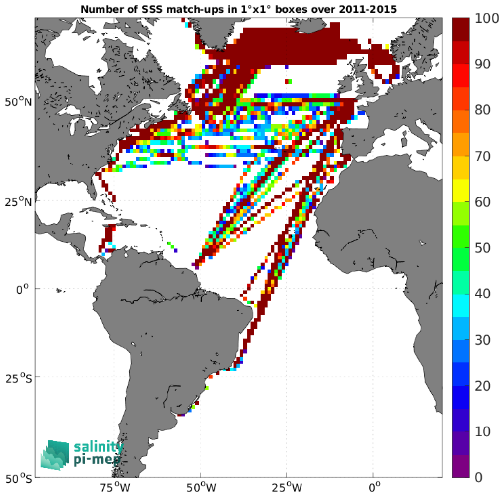
Figure 5: Number of SSS match-ups between TSG (LEGOS-DM) SSS and the Aquarius SSS L3 OR v5 - 7-Day running - Rain mask (NASA-GSFC) SSS product for the Atlantic Ocean Pi-MEP region over 1^\circ \times 1^\circ boxes and for the full satellite product period.
