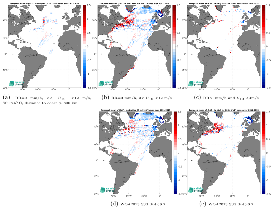
Figure 14: Temporal mean gridded over spatial boxes of size 1^\circ \times 1^\circ of \Delta SSS (Aquarius SSS L3 OR v5 - 7-Day running - Rain mask (NASA-GSFC) - TSG (LEGOS-DM)) for 5 different subdatasets corresponding to:RR=0 mm/h, 3 < U_{10} < 12 m/s, SST >5^\circ\text{C} , distance to coast > 800 km (a), RR=0 mm/h, 3 < U_{10} < 12 m/s (b), RR >1 mm/h and U_{10} < 4 m/s (c), WOA2013 SSS Std <0.2 (d), WOA2013 SSS Std >0.2 (e).
