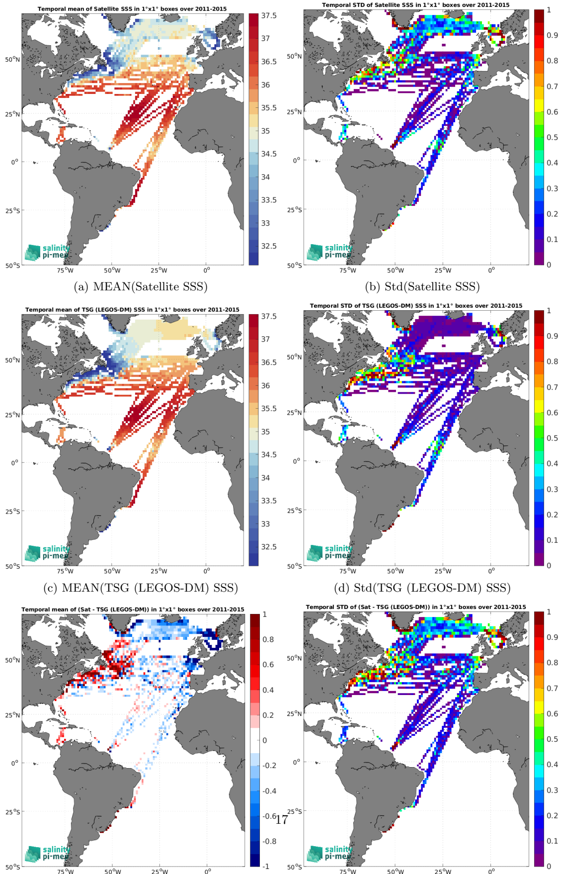
(e) MEAN( \Delta SSS) (Satellite - TSG (LEGOS-DM)) (f) Std( \Delta SSS) (Satellite - TSG (LEGOS-DM)) Figure 7: Temporal mean (left) and Std (right) of SSS from Aquarius SSS L3 OR v5 - 7-Day running - Rain mask (NASA-GSFC) (top), TSG (LEGOS-DM) (middle), and of \Delta SSS (Satellite - TSG (LEGOS-DM)). Only match-up pairs are used to generate these maps.
