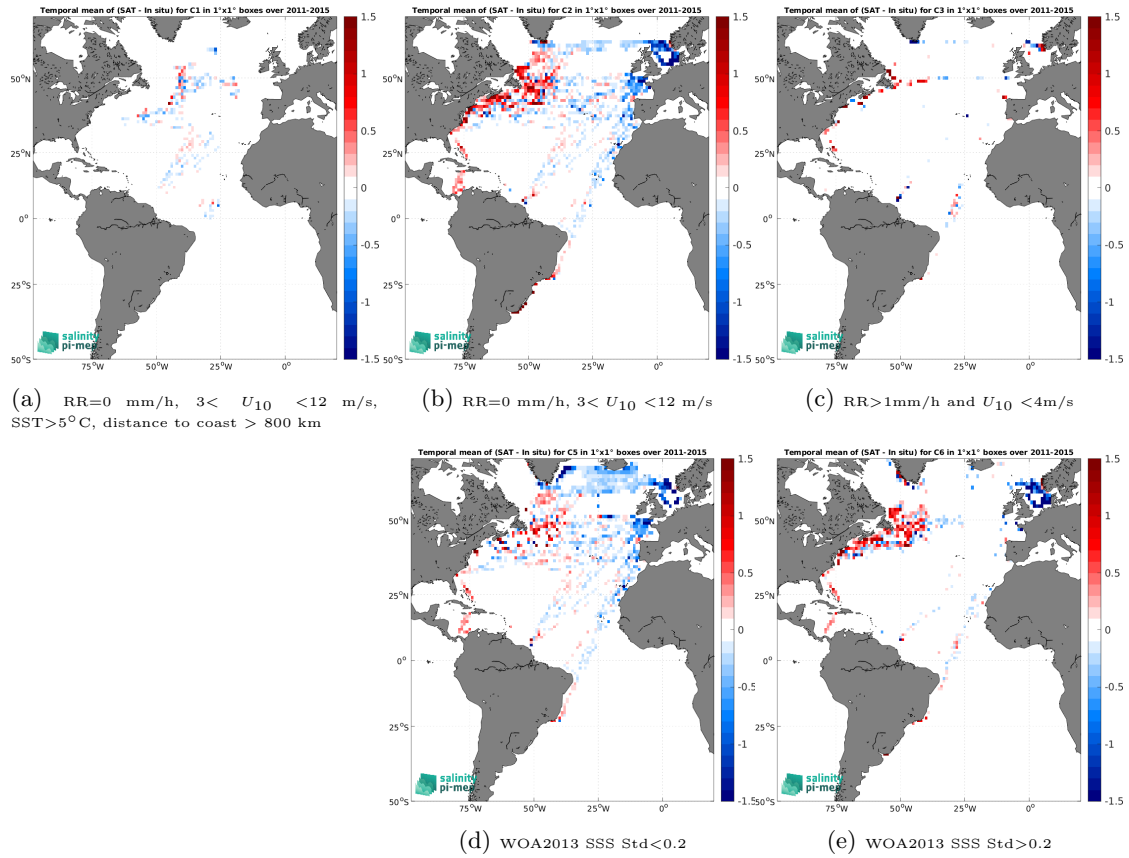
Figure 12: Temporal mean gridded over spatial boxes of size 1^\circ \times 1^\circ of \Delta\text{SSS} (Aquarius SSS L3 OR v5 - 7-Day running - Rain mask (NASA-GSFC) - TSG (LEGOS-DM)) for 5 different subdatasets corresponding to:RR=0 mm/h, 3 < U_{10} < 12 m/s, SST >5^\circ\text{C} , distance to coast > 800 km (a), RR=0 mm/h, 3 < U_{10} < 12 m/s (b), RR >1 mm/h and U_{10} < 4 m/s (c), WOA2013 SSS Std <0.2 (d), WOA2013 SSS Std >0.2 (e).
