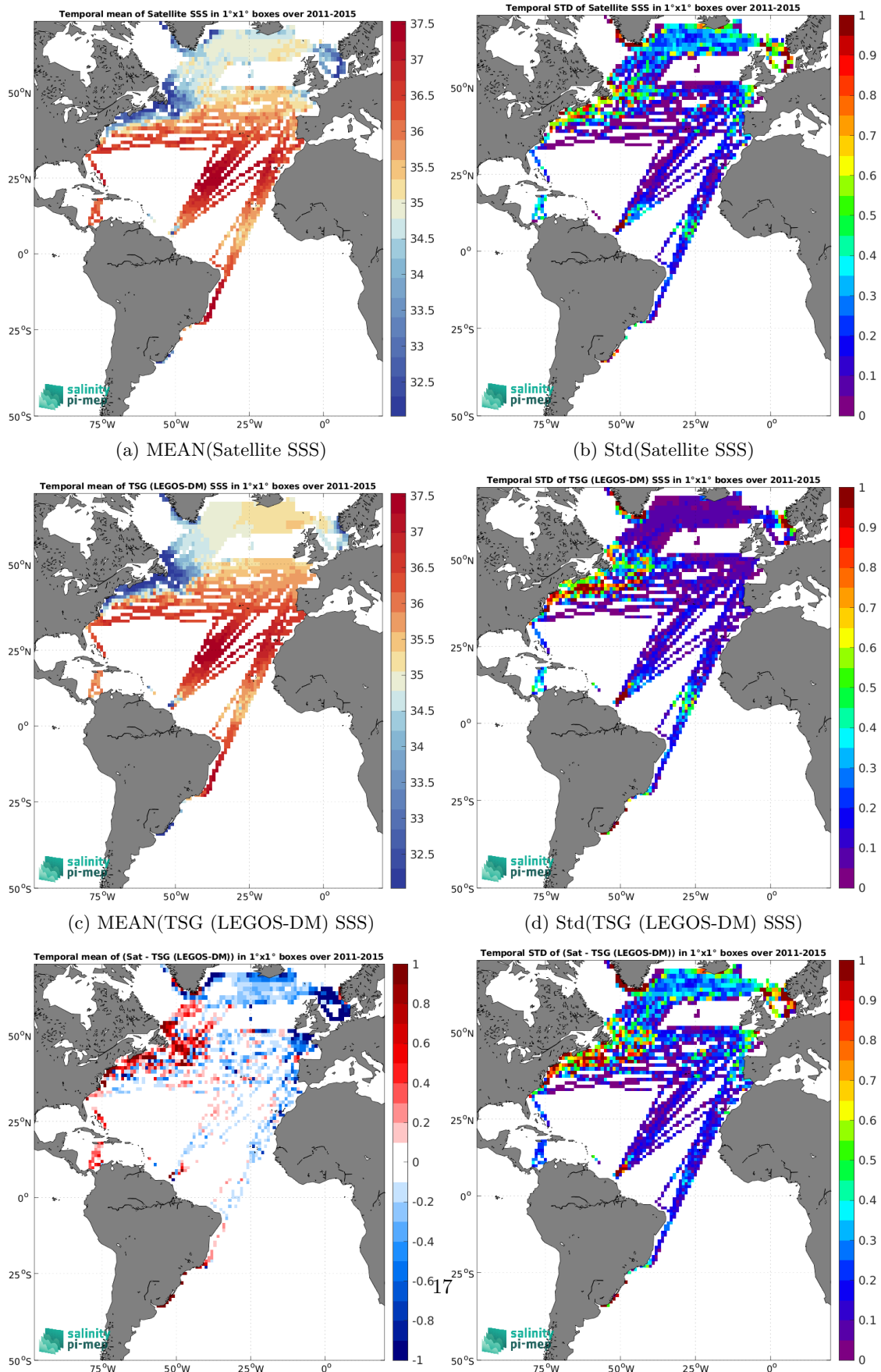
(e) MEAN( \Delta SSS) (Satellite - TSG (LEGOS-DM)) (f) Std( \Delta SSS) (Satellite - TSG (LEGOS-DM)) Figure 6: Temporal mean (left) and Std (right) of SSS from Aquarius SSS L3 OR v5 - 7-Day running - Rain mask (NASA-GSFC) (top), TSG (LEGOS-DM) (middle), and of \Delta SSS (Satellite - TSG (LEGOS-DM)). Only match-up pairs are used to generate these maps.
