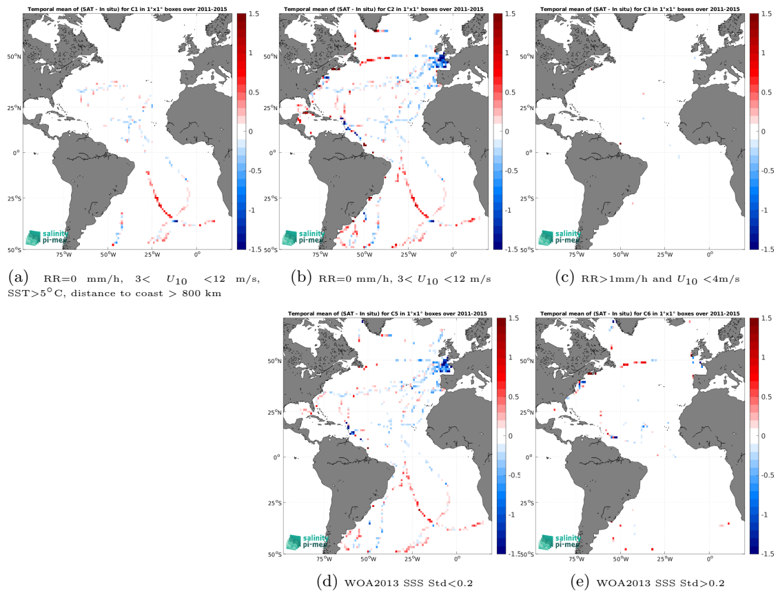
Figure 12: Temporal mean gridded over spatial boxes of size 1^\circ \times 1^\circ of \Delta SSS (Aquarius SSS L3 OR v5 - 7-Day running - Rain mask (NASA-GSFC) - TSG (GOSUD-Sailing-ship)) for 5 different subdatasets corresponding to:RR=0 mm/h, 3 < U_{10} < 12 m/s, SST >5^\circ\text{C} , distance to coast > 800 km (a), RR=0 mm/h, 3 < U_{10} < 12 m/s (b), RR >1 mm/h and U_{10} < 4 m/s (c), WOA2013 SSS Std <0.2 (d), WOA2013 SSS Std >0.2 (e).
