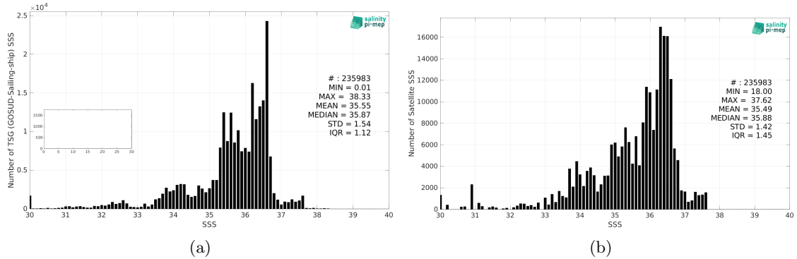
Figure 2: Histograms of SSS from TSG (GOSUD-Sailing-ship) (a) and Aquarius SSS L3 OR v5 - 7-Day running - Rain mask (NASA-GSFC) (b) considering all match-up pairs per bins of 0.1 over the Atlantic Ocean Pi-MEP region and for the full satellite product period.
