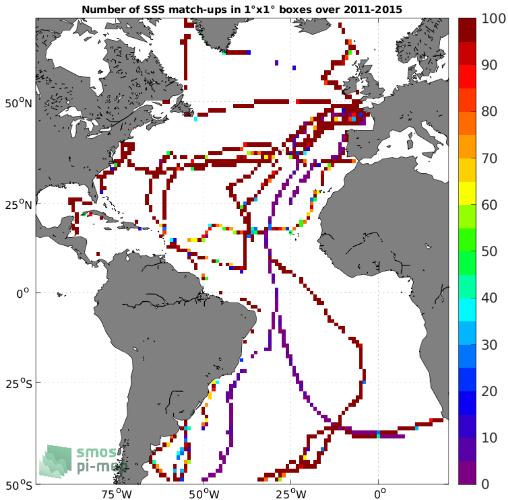
Figure 4: Number of SSS match-ups between TSG (GOSUD-Sailing-ship) SSS and the Aquarius SSS L3 OR v5 - 7-Day running - Rain mask (NASA-GSFC) SSS product for the Atlantic Ocean Pi-MEP region over 1°x1° boxes and for the full satellite product period.
