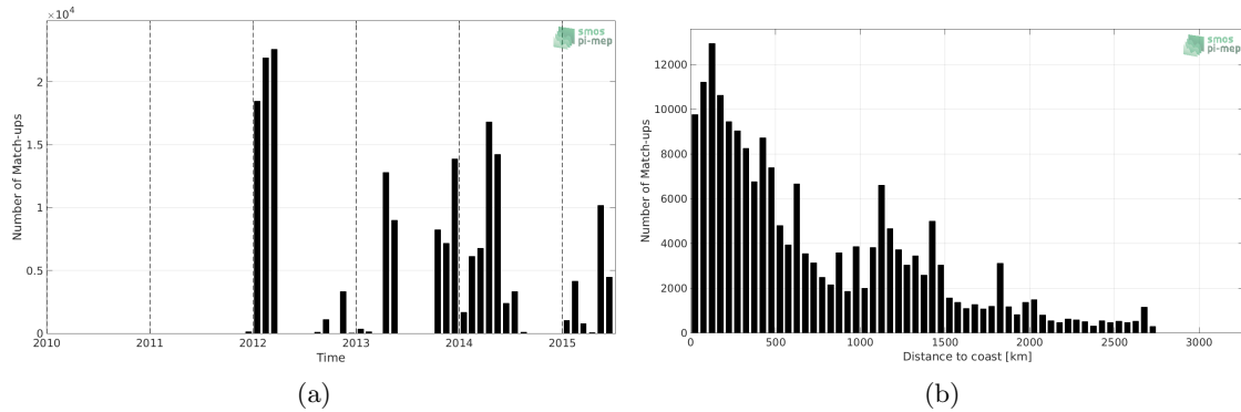
Figure 1: Number of match-ups between TSG-GOSUD-Sailing-ship and Aquarius-L3-OR-V5-7DAY-RUNNING-RAIN-MASK-1DEG SSS as a function of time (a) and as function of the distance to coast (b) over the Atlantic Ocean Pi-MEP region and for the full satellite product period.
