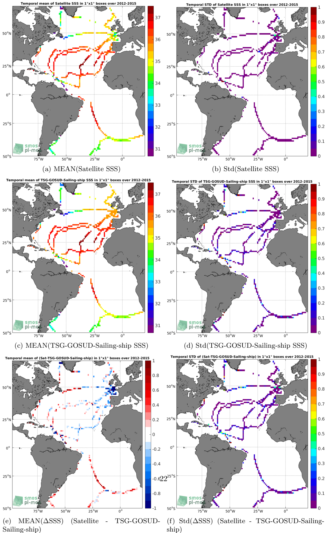
Figure 6: Temporal mean (left) and Std (right) of SSS from Aquarius-L3-OR-V5-7DAY-RUNNING-RAIN-MASK-1DEG (top), TSG-GOSUD-Sailing-ship (middle), and of \Delta SSS (Satellite - TSG-GOSUD-Sailing-ship). Only match-up pairs are used to generate these maps.
