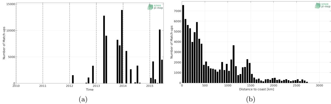
Figure 1: Number of match-ups between TSG-GOSUD-Sailing-ship and Aquarius-L3-OR-V5-7DAY-RUNNING-RAIN-MASK-1DEG SSS as a function of time (a) and as function of the distance to coast (b) over the Atlantic Ocean Pi-MEP region and for the full satellite product period.
