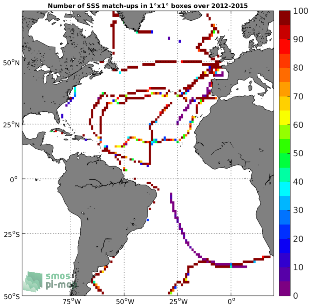
Figure 4: Number of SSS match-ups between TSG-GOSUD-Sailing-ship SSS and the Aquarius-L3-OR-V5-7DAY-RUNNING-RAIN-MASK-1DEG SSS product for the Atlantic Ocean Pi-MEP region over 1°x1° boxes and for the full satellite product period.
