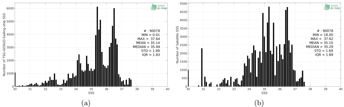
Figure 2: Histograms of SSS from TSG-GOSUD-Sailing-ship (a) and Aquarius-L3-OR-V5-7DAY-RUNNING-RAIN-MASK-1DEG (b) considering all match-up pairs per bins of 0.1 over the Atlantic Ocean Pi-MEP region and for the full satellite product period.
