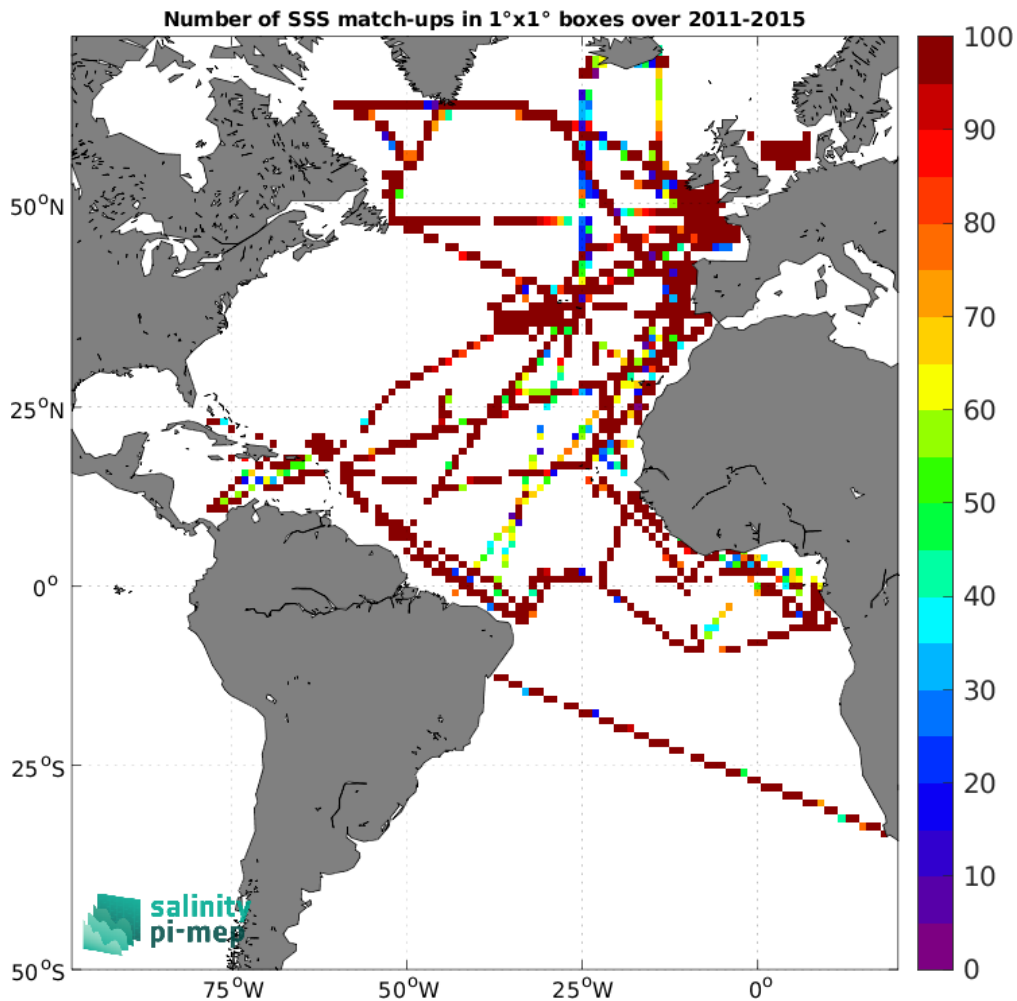
Figure 5: Number of SSS match-ups between TSG (GOSUD-Research-vessel) SSS and the Aquarius SSS L3 OR v5 - 7-Day running - Rain mask (NASA-GSFC) SSS product for the Atlantic Ocean Pi-MEP region over 1^\circ \times 1^\circ boxes and for the full satellite product period.
