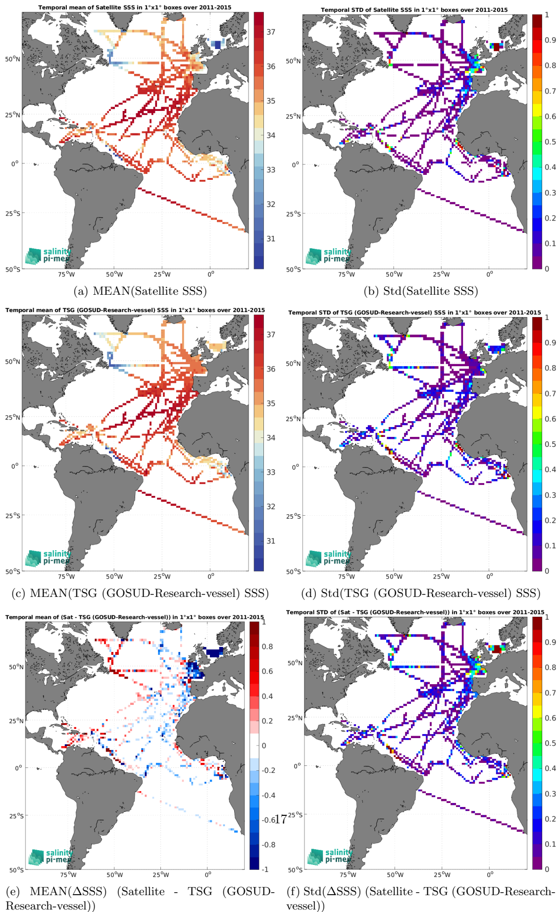
Figure 7: Temporal mean (left) and Std (right) of SSS from Aquarius SSS L3 OR v5 - 7-Day running - Rain mask (NASA-GSFC) (top), TSG (GOSUD-Research-vessel) (middle), and of \Delta SSS (Satellite - TSG (GOSUD-Research-vessel)). Only match-up pairs are used to generate these maps.
