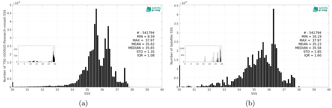
Figure 3: Histograms of SSS from TSG (GOSUD-Research-vessel) (a) and Aquarius SSS L3 OR v5 - 7-Day running - Rain mask (NASA-GSFC) (b) considering all match-up pairs per bins of 0.1 over the Atlantic Ocean Pi-MEP region and for the full satellite product period.
