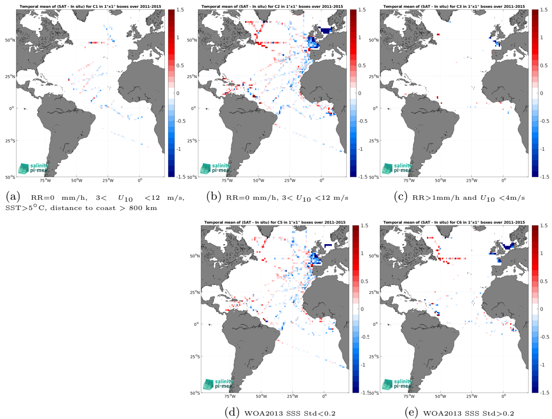
Figure 14: Temporal mean gridded over spatial boxes of size 1^\circ \times 1^\circ of \Delta SSS (Aquarius SSS L3 OR v5 - 7-Day running - Rain mask (NASA-GSFC) - TSG (GOSUD-Research-vessel)) for 5 different subdatasets corresponding to:RR=0 mm/h, 3 < U_{10} < 12 m/s, SST >5^\circ\text{C} , distance to coast > 800 km (a), RR=0 mm/h, 3 < U_{10} < 12 m/s (b), RR >1 mm/h and U_{10} < 4 m/s (c), WOA2013 SSS Std <0.2 (d), WOA2013 SSS Std >0.2 (e).
