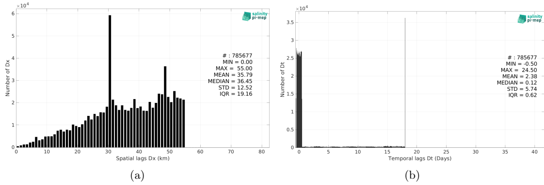
Figure 5: Histograms of the spatial (a) and temporal (b) lags between the location/time of the TSG (GOSUD-Research-vessel) measurement and the date of the corresponding Aquarius SSS L3 OR v5 - 7-Day running - Rain mask (NASA-GSFC) SSS pixel.
