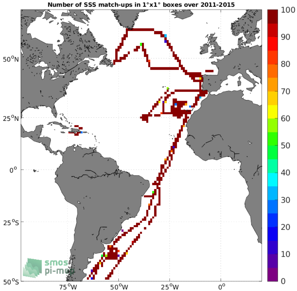
Figure 4: Number of SSS match-ups between TSG (CSIC-UTM) SSS and the Aquarius SSS L3 OR v5 - 7-Day running - Rain mask (NASA-GSFC) SSS product for the Atlantic Ocean Pi-MEP region over 1°x1° boxes and for the full satellite product period.
