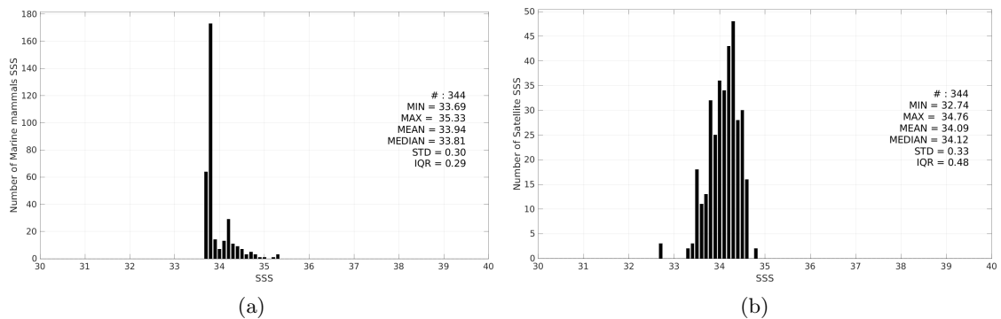
Figure 3: Histograms of SSS from Marine mammals (a) and Aquarius SSS L3 OR v5 - 7-Day running - Rain mask (NASA-GSFC) (b) considering all match-up pairs per bins of 0.1 over the Atlantic Ocean Pi-MEP region and for the full satellite product period.
