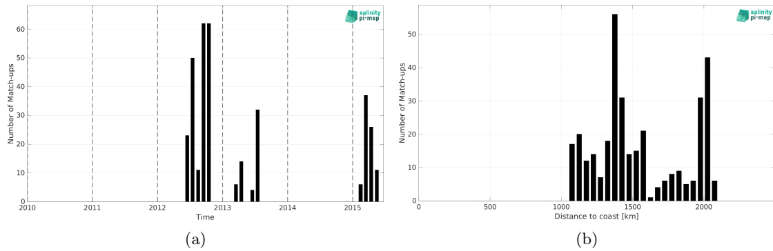
Figure 2: Number of match-ups between Marine mammals and Aquarius SSS L3 OR v5 - 7-Day running - Rain mask (NASA-GSFC) SSS as a function of time (a) and as function of the distance to coast (b) over the Atlantic Ocean Pi-MEP region and for the full satellite product period.
