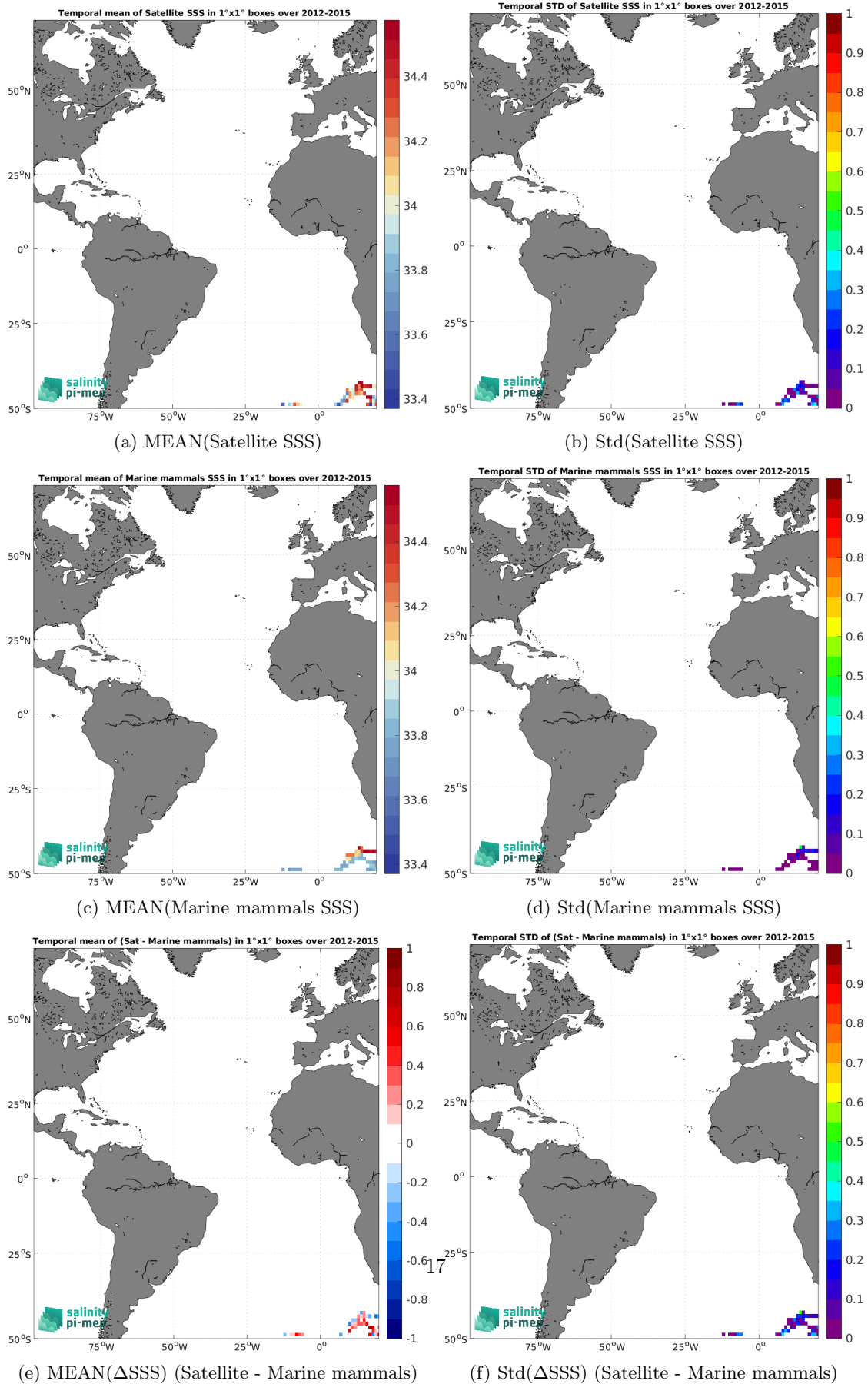
Figure 7: Temporal mean (left) and Std (right) of SSS from Aquarius SSS L3 OR v5 - 7-Day running - Rain mask (NASA-GSFC) (top), Marine mammals (middle), and of \Delta SSS (Satellite - Marine mammals). Only match-up pairs are used to generate these maps.
