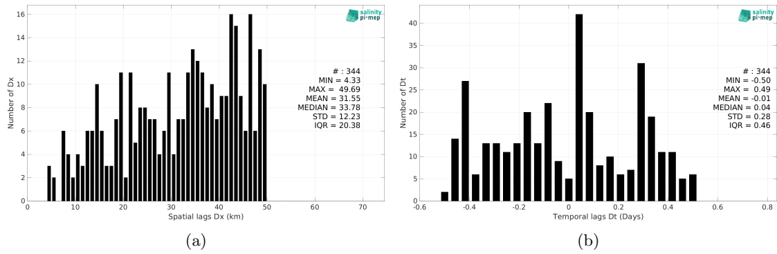
Figure 6: Histograms of the spatial (a) and temporal (b) lags between the location/time of the Marine mammals measurement and the date of the corresponding Aquarius SSS L3 OR v5 - 7-Day running - Rain mask (NASA-GSFC) SSS pixel.
