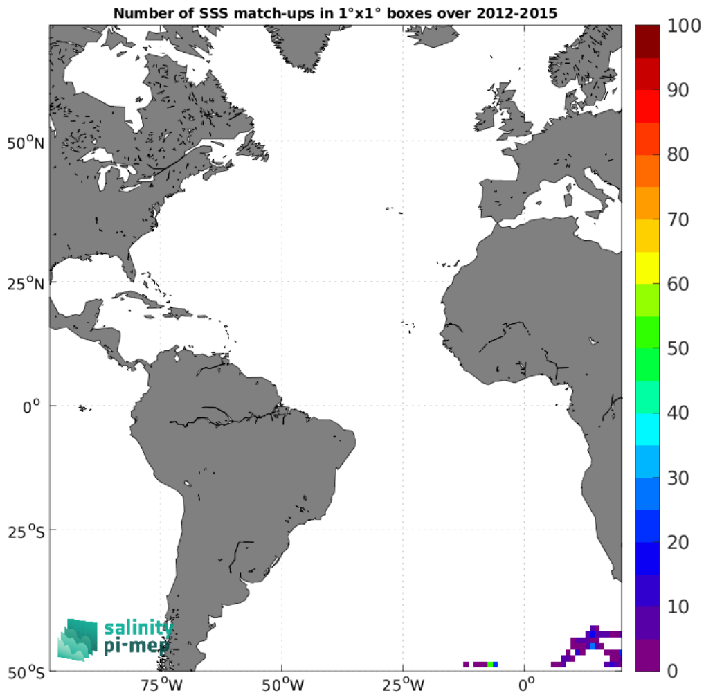
Figure 5: Number of SSS match-ups between Marine mammals SSS and the Aquarius SSS L3 OR v5 - 7-Day running - Rain mask (NASA-GSFC) SSS product for the Atlantic Ocean Pi-MEP region over 1^\circ \times 1^\circ boxes and for the full satellite product period.
