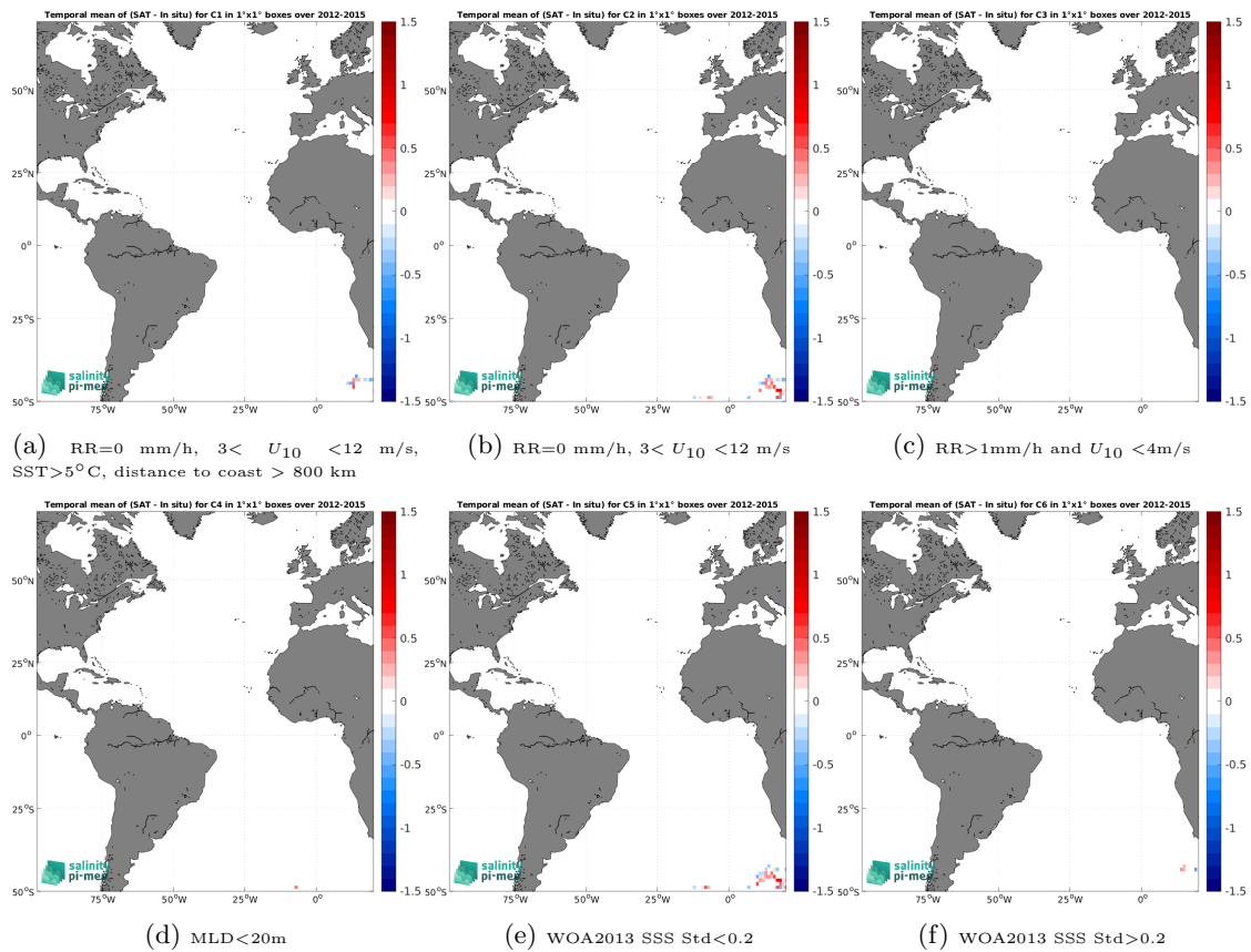
Figure 14: Temporal mean gridded over spatial boxes of size 1^\circ \times 1^\circ of \Delta SSS (Aquarius SSS L3 OR v5 - 7-Day running - Rain mask (NASA-GSFC) - Marine mammals) for 6 different subdatasets corresponding to:RR=0 mm/h, 3 < U_{10} < 12 m/s, SST>5°C, distance to coast > 800 km (a), RR=0 mm/h, 3 < U_{10} < 12 m/s (b), RR>1mm/h and U_{10} < 4 m/s (c),MLD<20m (d),WOA2013 SSS Std<0.2 (e),WOA2013 SSS Std>0.2 (f).
