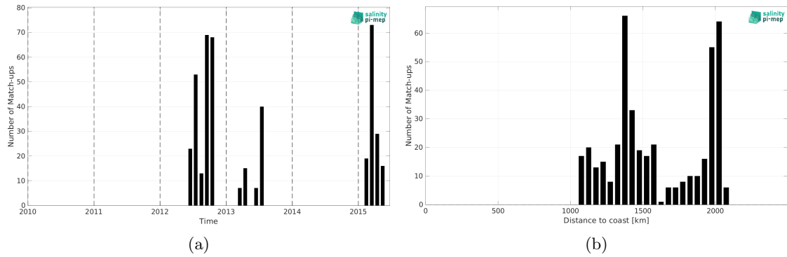
Figure 1: Number of match-ups between Marine mammals and Aquarius SSS L3 OR v5 - 7-Day running - Rain mask (NASA-GSFC) SSS as a function of time (a) and as function of the distance to coast (b) over the Atlantic Ocean Pi-MEP region and for the full satellite product period.
