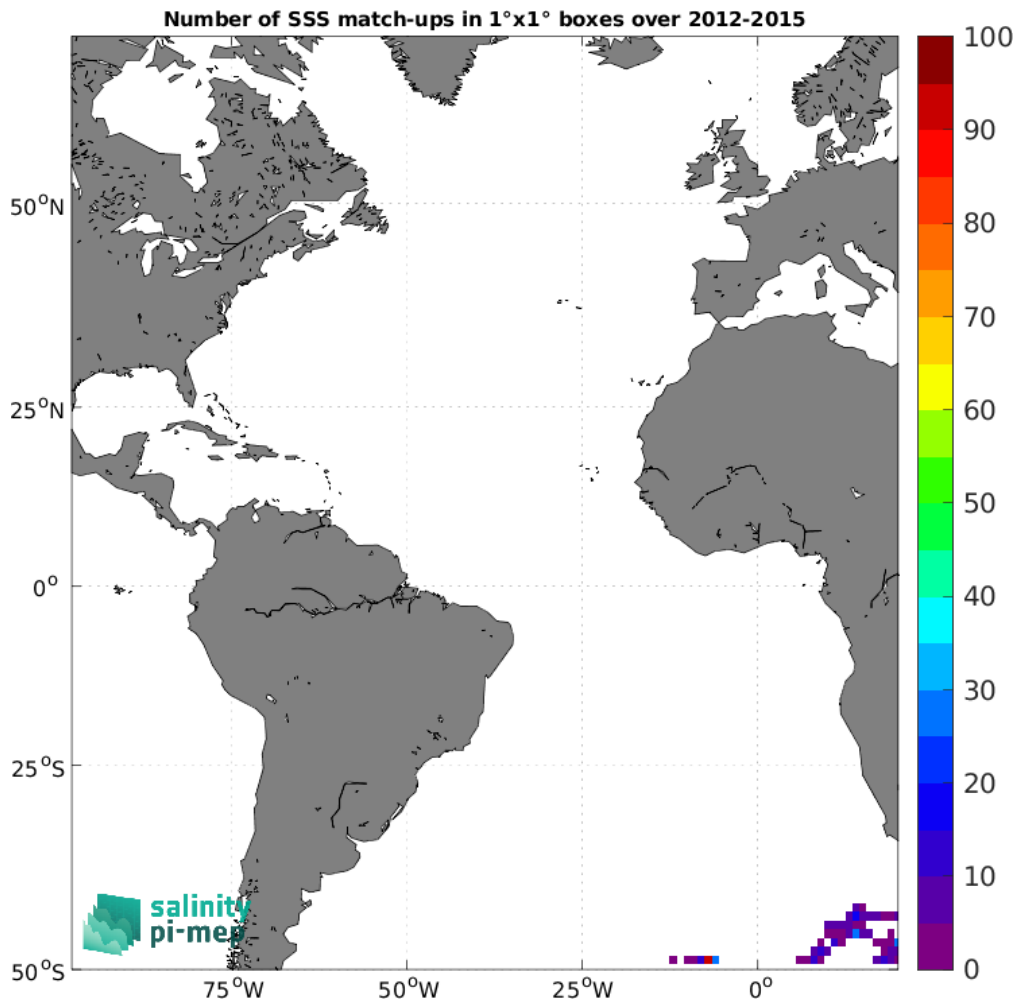
Figure 4: Number of SSS match-ups between Marine mammals SSS and the Aquarius SSS L3 OR v5 - 7-Day running - Rain mask (NASA-GSFC) SSS product for the Atlantic Ocean Pi-MEP region over 1^\circ \times 1^\circ boxes and for the full satellite product period.
