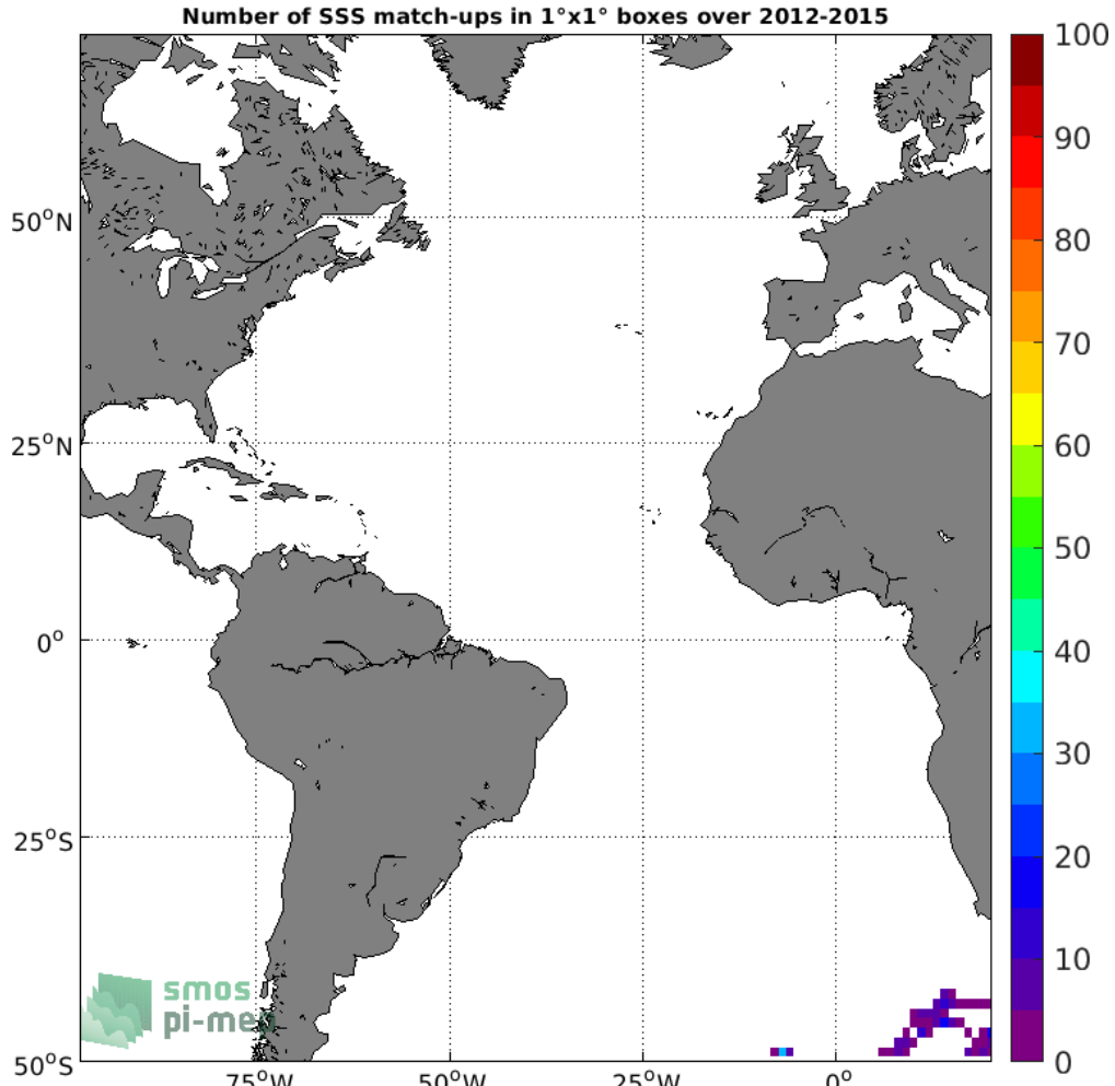
Figure 4: Number of SSS match-ups between Marine mammals SSS and the Aquarius SSS L3 OR v5 - 7-Day running - Rain mask (NASA-GSFC) SSS product for the Atlantic Ocean Pi-MEP region over 1^\circ \times 1^\circ boxes and for the full satellite product period.
