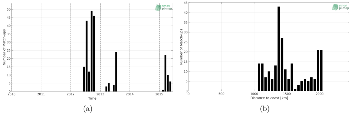
Figure 1: Number of match-ups between Sea mammals and Aquarius-L3-OR-V5-7DAY-RUNNING-RAIN-MASK-1DEG SSS as a function of time (a) and as function of the distance to coast (b) over the Atlantic Ocean Pi-MEP region and for the full satellite product period.
