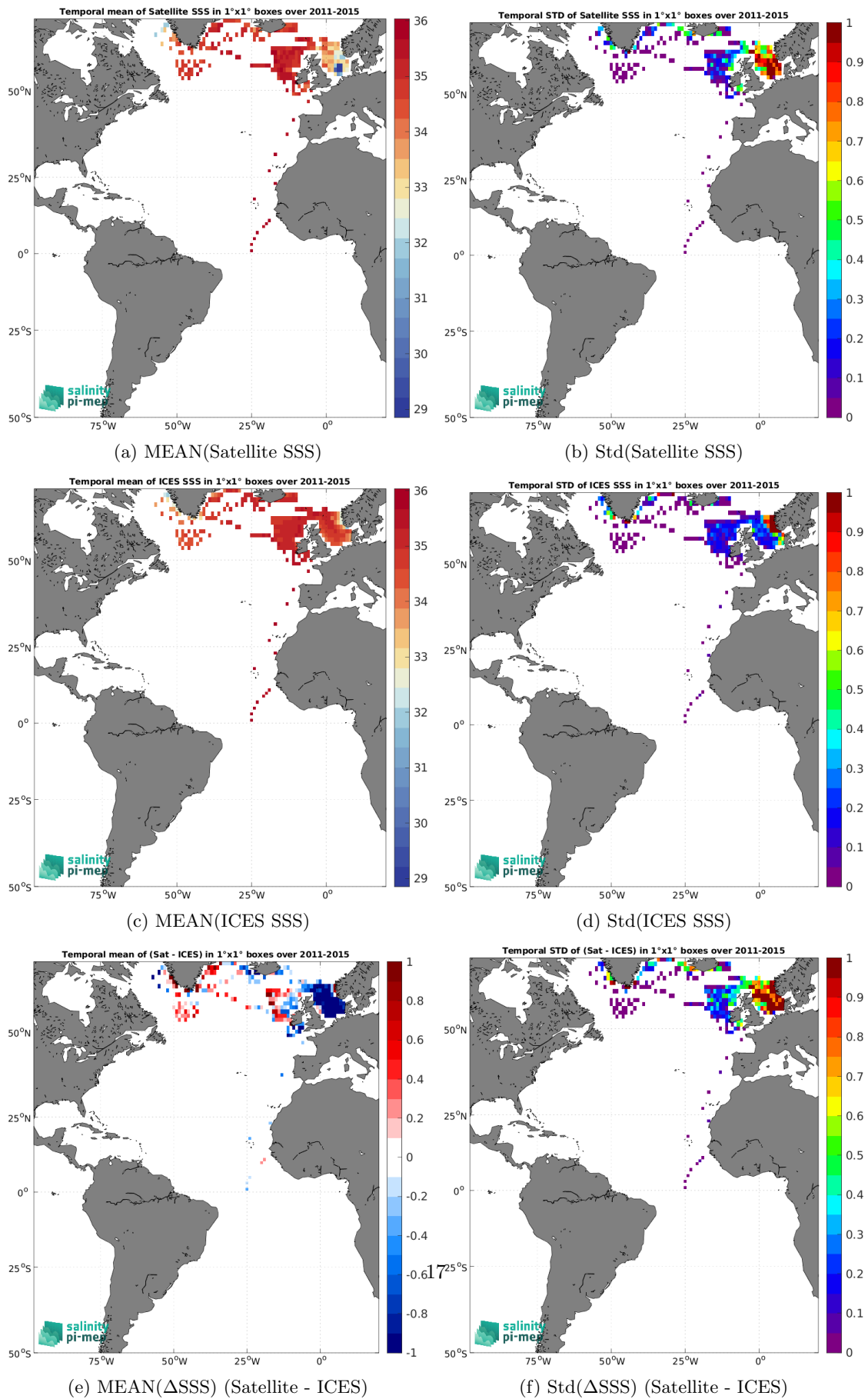
Figure 7: Temporal mean (left) and Std (right) of SSS from Aquarius SSS L3 OR v5 - 7-Day running - Rain mask (NASA-GSFC) (top), ICES (middle), and of \Delta SSS (Satellite - ICES). Only match-up pairs are used to generate these maps.
