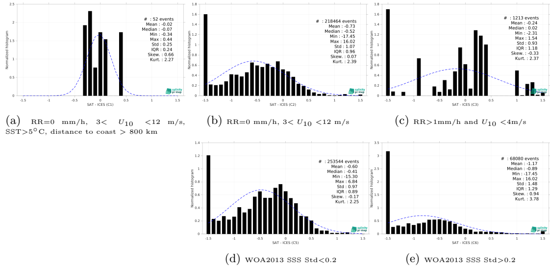
Figure 15: Normalized histogram of \Delta SSS (Aquarius SSS L3 OR v5 - 7-Day running - Rain mask (NASA-GSFC) - ICES) for 5 different subdatasets corresponding to: RR=0 mm/h, 3 < U_{10} < 12 m/s, SST>5°C, distance to coast > 800 km (a), RR=0 mm/h, 3 < U_{10} < 12 m/s (b), RR>1mm/h and U_{10} < 4 m/s (c), WOA2013 SSS Std<0.2 (d), WOA2013 SSS Std>0.2 (e).
