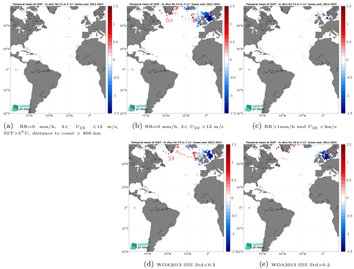
Figure 14: Temporal mean gridded over spatial boxes of size 1^\circ \times 1^\circ of \Delta\text{SSS} (Aquarius SSS L3 OR v5 - 7-Day running - Rain mask (NASA-GSFC) - ICES) for 5 different subdatasets corresponding to:RR=0 mm/h, 3 < U_{10} < 12 m/s, SST>5°C, distance to coast > 800 km (a), RR=0 mm/h, 3 < U_{10} < 12 m/s (b), RR>1mm/h and U_{10} < 4 m/s (c), WOA2013 SSS Std<0.2 (d), WOA2013 SSS Std>0.2 (e).
