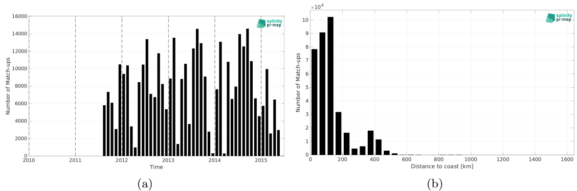
Figure 2: Number of match-ups between ICES and Aquarius SSS L3 OR v5 - 7-Day running - Rain mask (NASA-GSFC) SSS as a function of time (a) and as function of the distance to coast (b) over the Atlantic Ocean Pi-MEP region and for the full satellite product period.
