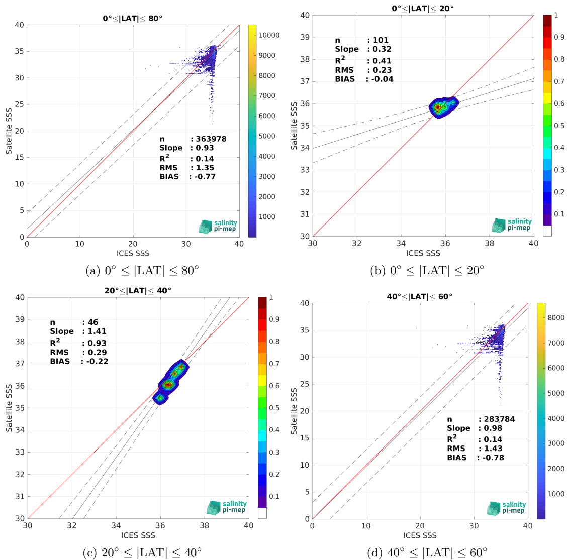
Figure 10: Contour maps of the concentration of Aquarius SSS L3 OR v5 - 7-Day running - Rain mask (NASA-GSFC) SSS (y-axis) versus ICES SSS (x-axis) at match-up pairs for different latitude bands. For each plot, the red line shows x=y . The black thin and dashed lines indicate a linear fit through the data cloud and the \pm 95\% confidence levels, respectively. The number match-up pairs n , the slope and R^2 coefficient of the linear fit, the root mean square (RMS) and the mean bias between satellite and in situ data are indicated for each latitude band in each plots.
