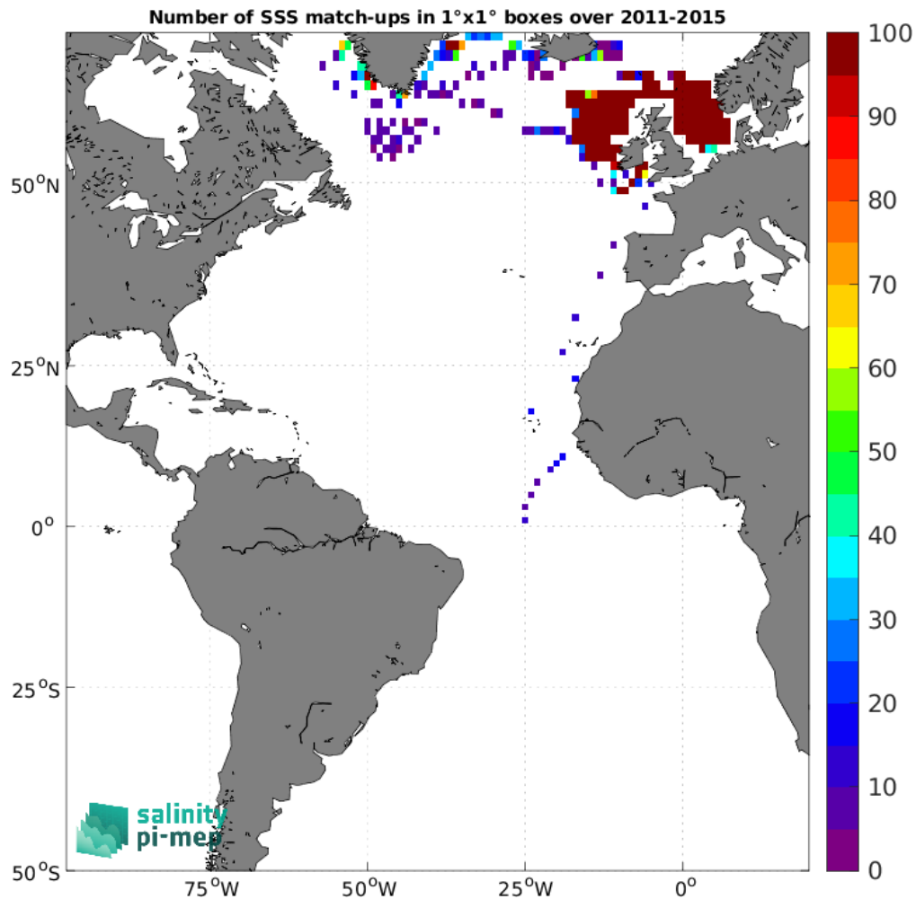
Figure 5: Number of SSS match-ups between ICES SSS and the Aquarius SSS L3 OR v5 - 7-Day running - Rain mask (NASA-GSFC) SSS product for the Atlantic Ocean Pi-MEP region over 1^\circ \times 1^\circ boxes and for the full satellite product period.
