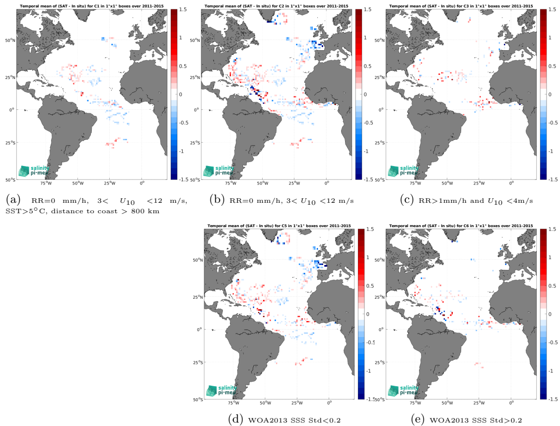
Figure 13: Temporal mean gridded over spatial boxes of size 1^\circ \times 1^\circ of \Delta SSS (Aquarius SSS L3 OR v5 - 7-Day running - Rain mask (NASA-GSFC) - Surface drifters) for 5 different subdatasets corresponding to:RR=0 mm/h, 3 < U_{10} < 12 m/s, SST >5^\circ\text{C} , distance to coast > 800 km (a), RR=0 mm/h, 3 < U_{10} < 12 m/s (b), RR >1 mm/h and U_{10} < 4 m/s (c), WOA2013 SSS Std <0.2 (d), WOA2013 SSS Std >0.2 (e).
