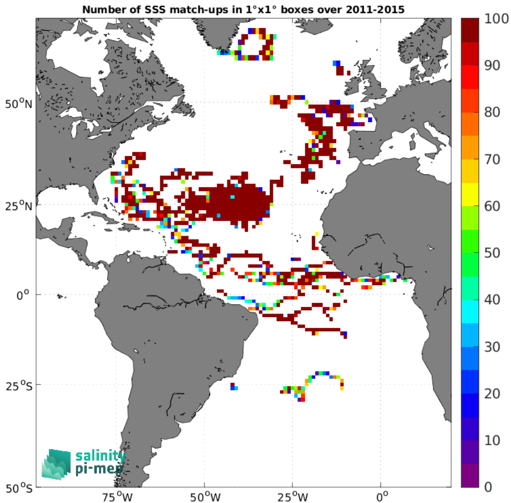
Figure 4: Number of SSS match-ups between Surface drifters SSS and the Aquarius SSS L3 OR v5 - 7-Day running - Rain mask (NASA-GSFC) SSS product for the Atlantic Ocean Pi-MEP region over 1^\circ \times 1^\circ boxes and for the full satellite product period.
