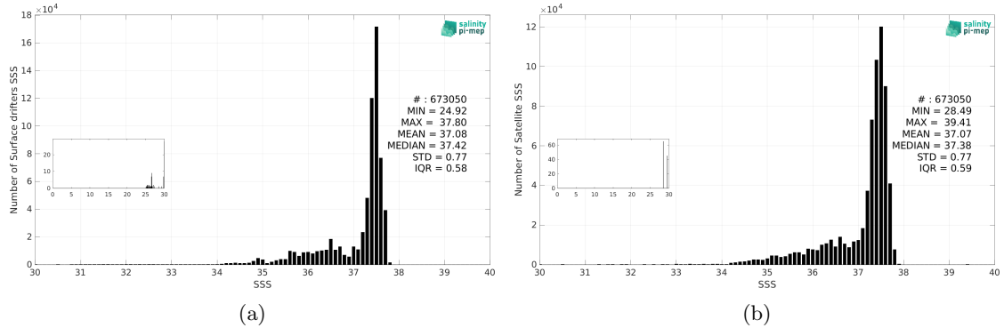
Figure 3: Histograms of SSS from Surface drifters (a) and Aquarius SSS L3 OR v5 - 7-Day running - Rain mask (NASA-GSFC) (b) considering all match-up pairs per bins of 0.1 over the Atlantic Ocean Pi-MEP region and for the full satellite product period.
