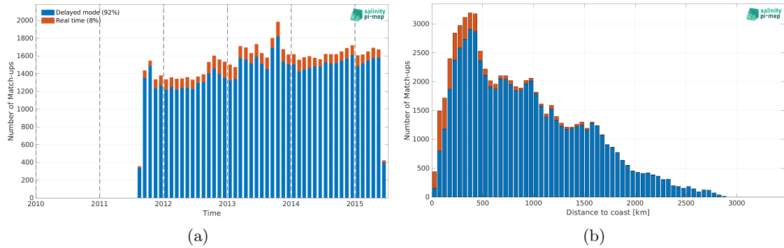
Figure 2: Number of match-ups between Argo and Aquarius SSS L3 OR v5 - 7-Day running - Rain mask (NASA-GSFC) SSS as a function of time (a) and as function of the distance to coast (b) over the Atlantic Ocean Pi-MEP region and for the full satellite product period.
