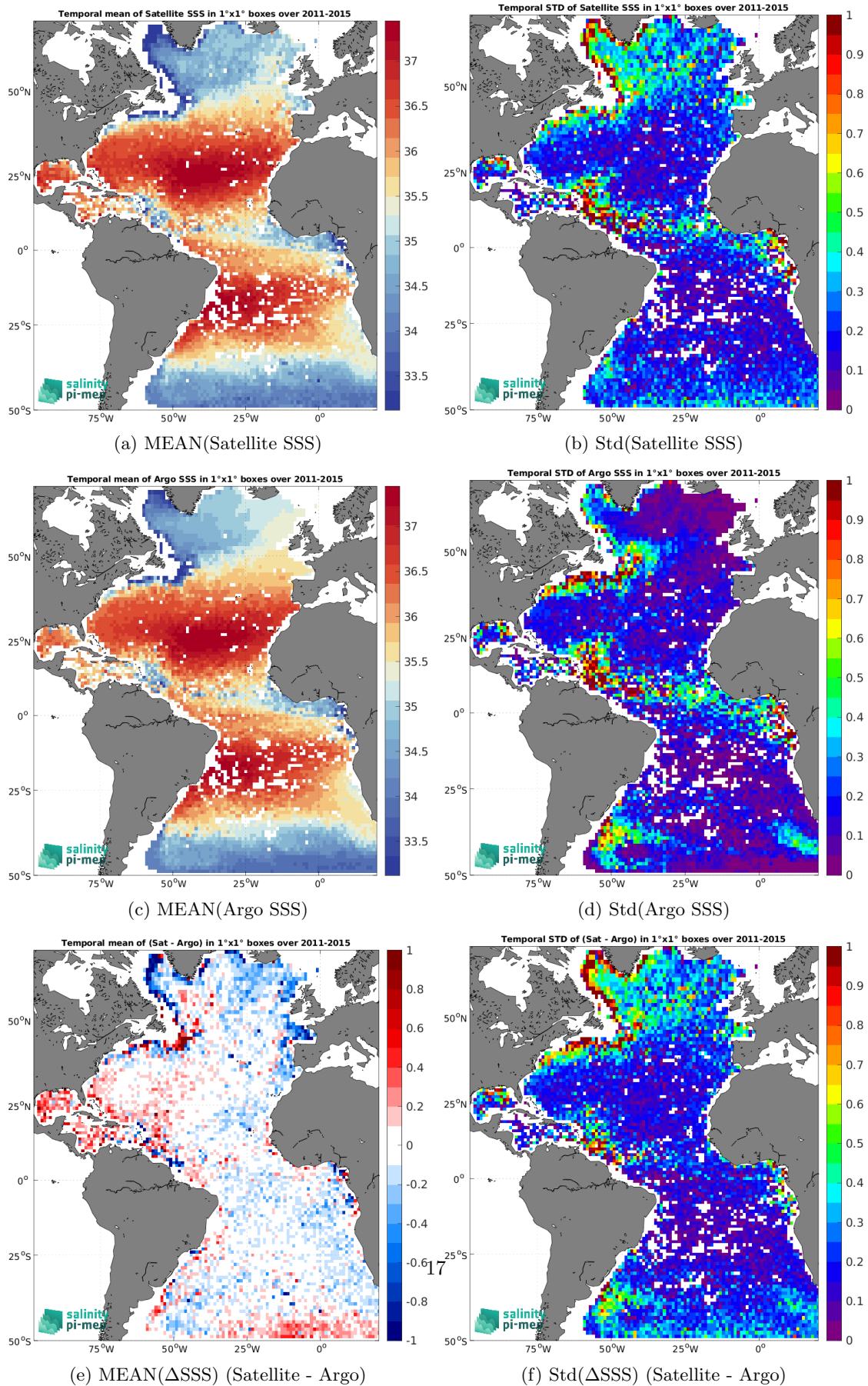
Figure 7: Temporal mean (left) and Std (right) of SSS from Aquarius SSS L3 OR v5 - 7-Day running - Rain mask (NASA-GSFC) (top), Argo (middle), and of \Delta SSS (Satellite - Argo). Only match-up pairs are used to generate these maps.
