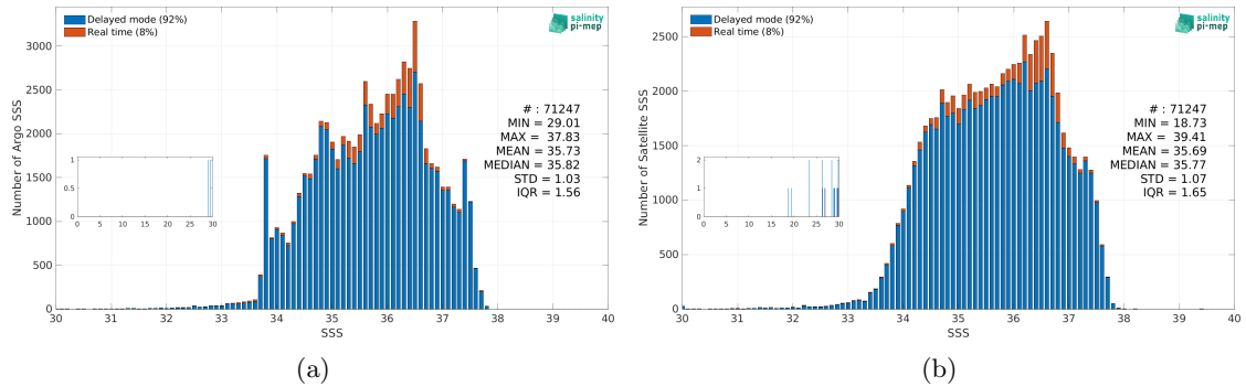
Figure 3: Histograms of SSS from Argo (a) and Aquarius SSS L3 OR v5 - 7-Day running - Rain mask (NASA-GSFC) (b) considering all match-up pairs per bins of 0.1 over the Atlantic Ocean Pi-MEP region and for the full satellite product period.
