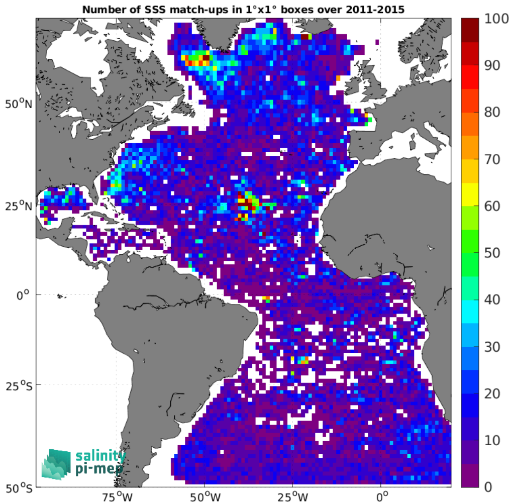
Figure 5: Number of SSS match-ups between Argo SSS and the Aquarius SSS L3 OR v5 - 7-Day running - Rain mask (NASA-GSFC) SSS product for the Atlantic Ocean Pi-MEP region over 1^\circ \times 1^\circ boxes and for the full satellite product period.
