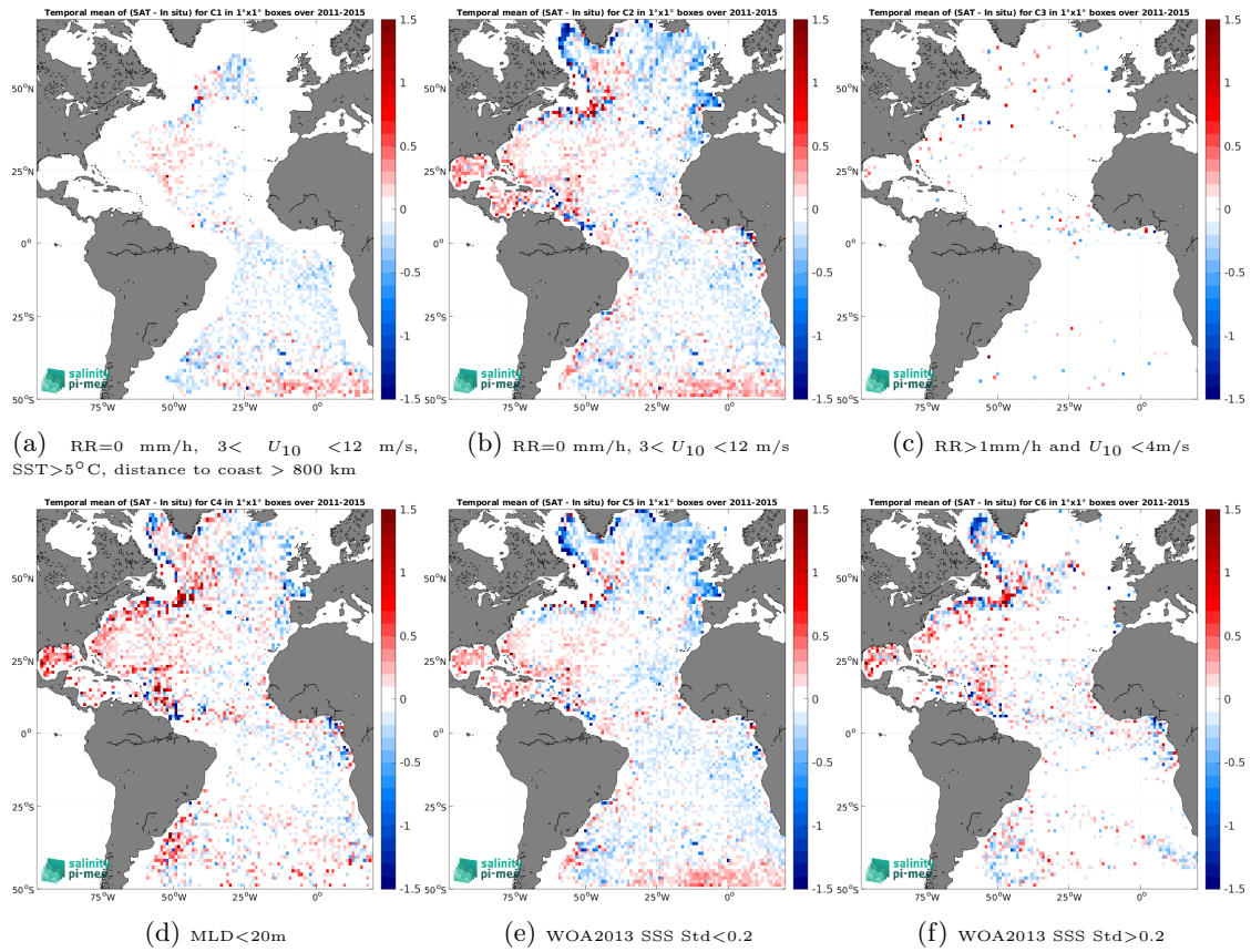
Figure 14: Temporal mean gridded over spatial boxes of size 1^\circ \times 1^\circ of \Delta\text{SSS} (Aquarius SSS L3 OR v5 - 7-Day running - Rain mask (NASA-GSFC) - Argo) for 6 different subdatasets corresponding to:RR=0 mm/h, 3 < U_{10} < 12 m/s, SST>5°C, distance to coast > 800 km (a), RR=0 mm/h, 3 < U_{10} < 12 m/s (b), RR>1mm/h and U_{10} < 4 m/s (c),MLD<20m (d),WOA2013 SSS Std<0.2 (e),WOA2013 SSS Std>0.2 (f).
